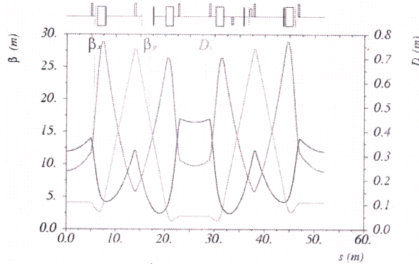
Fig. 2: 1/15 th of the in-tunnel booster lattice
