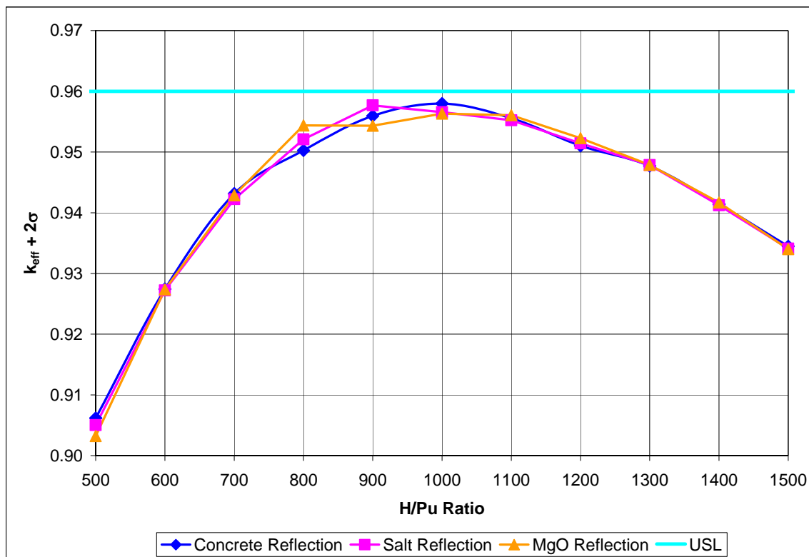
Figure A-, System Reactivity for SLB2-SWB Two-Container Model
