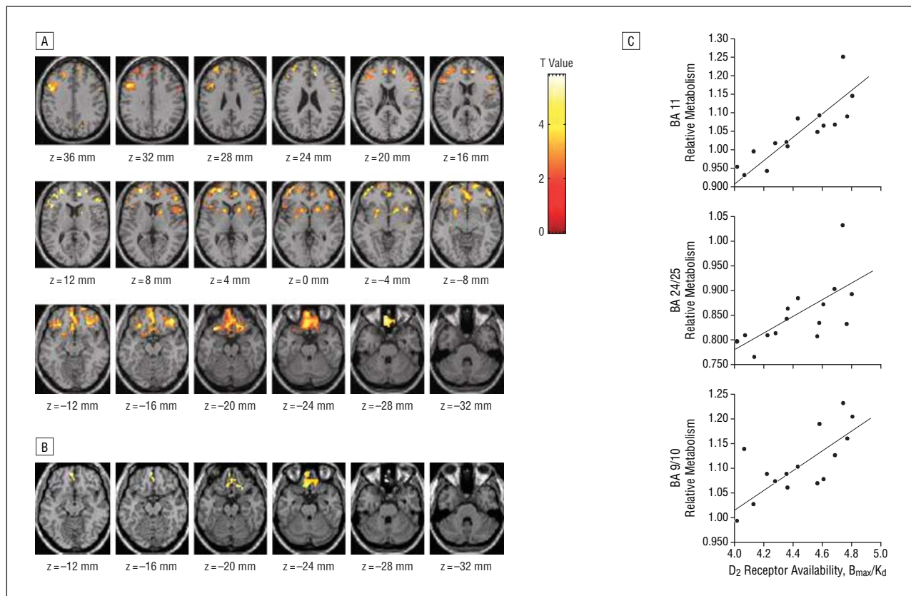
Figure 3. Correlations between dopamine D_2 receptor availability and regional brain metabolism. A, Statistical parametric mapping images for the family-positive subjects showing areas where metabolism was significantly correlated with D_2 receptor availability ( B_{max}/K_d ; see the “Methods” section for an explanation) in striatum ( P < .05 , corrected; cluster size, > 100 voxels). B, Statistical parametric mapping results for the “exploratory analysis” showing only planes where differences were significant at P < .005 (corrected; cluster size, > 100 voxels). C, Regression plots for the correlations between D_2 receptor availability in striatum and metabolic activity in orbitofrontal cortex (Brodmann area [BA] 11) ( r = 0.85 ; P < .001 ), ventral cingulate gyrus (BA 24/25) ( r = 0.66 ; P < .008 ), and prefrontal cortex (BA 9/10) ( r = 0.72 ; P < .003 ). The correlations in the family-negative subjects were not significant.
