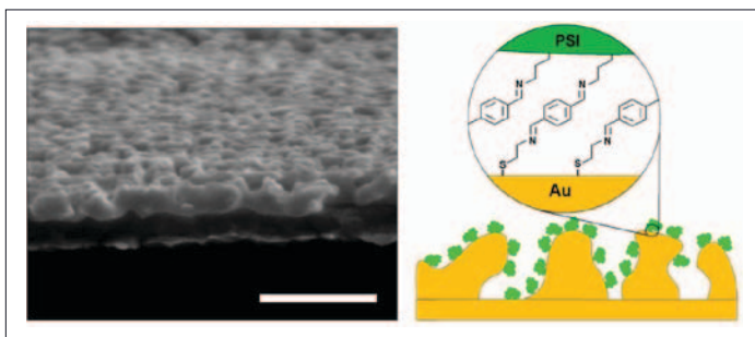
Figure 1.5. Nanoporous gold leaf electrodes ( left : cross-section view; scale bar is 300 nm) can be used to immobilize functional biological species, in this case, a species called photosystem I. (Reprinted with permission from ACS Nano 2, 2465, © 2008 American Chemical Society.)
