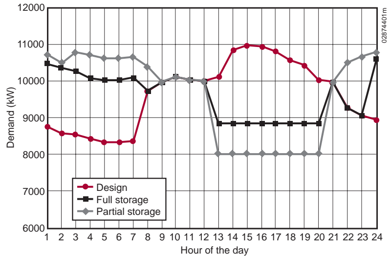
This graph represents daily demand in August for both current design conditions and the partial and full thermal storage conditions. The hospital can meet cooling requirements by producing chilled water during the period of lowest electric cost, then storing it for use during periods of high electric cost.
