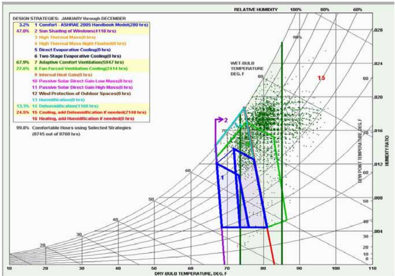
Figure 4: Psychrometric Chart
