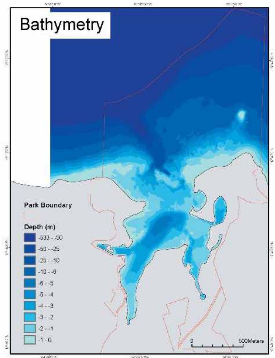
Figure 1: Interpolated bathymetry for Salt River Bay, based on the available soundings conducted in 1982 and 1977 from National Oceanic and Atmospheric Administration Geophysical Data System.
