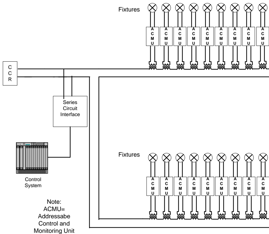
Figure 140. Typical Power Line Carrier System
