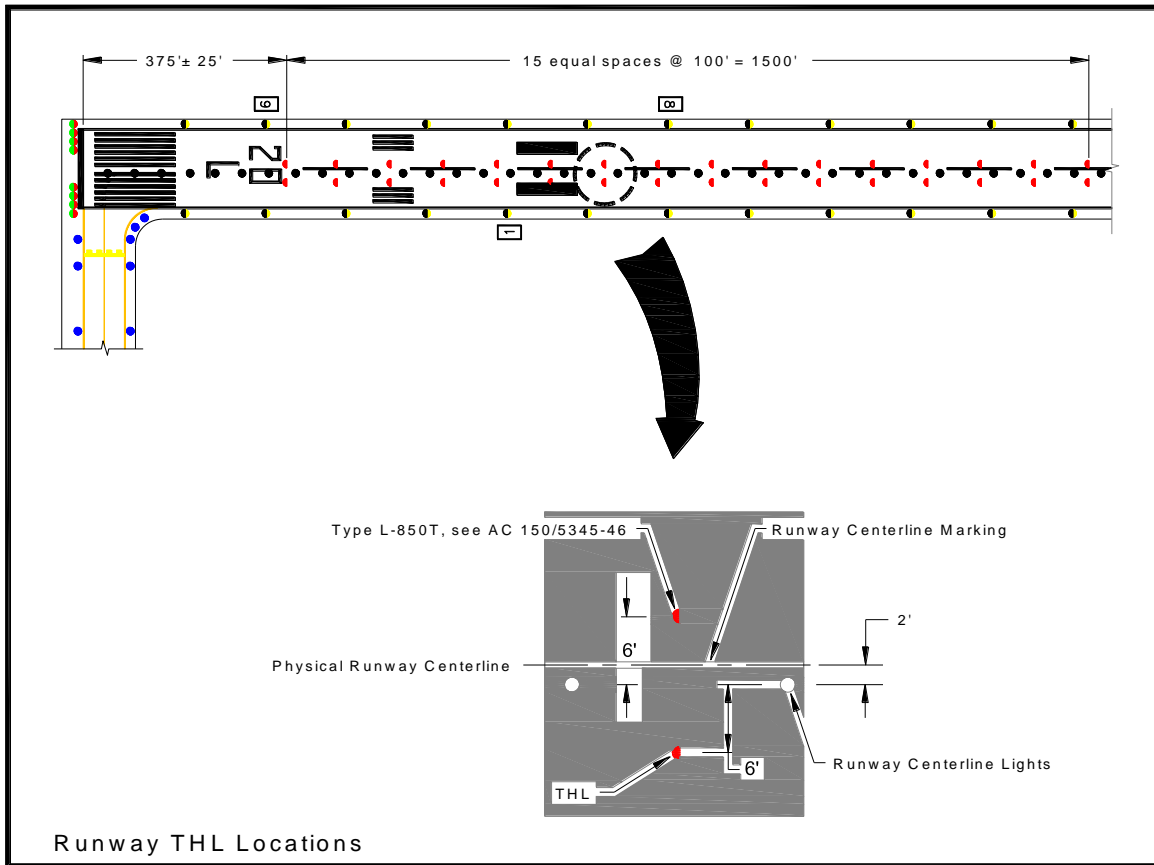
Figure 145. Takeoff/Hold Lights
