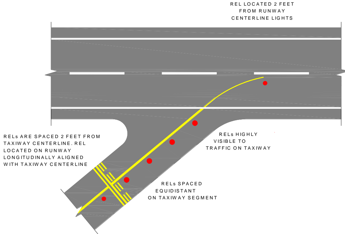
Figure 144. Angled Configuration
