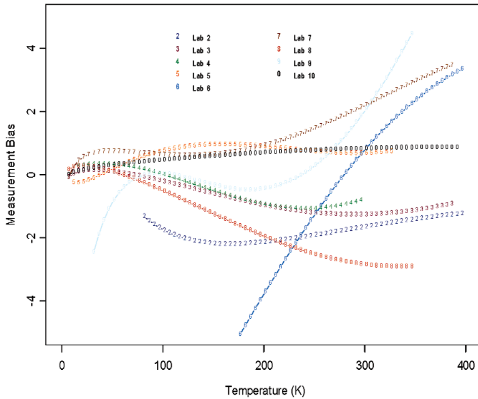
Fig. 8. Laboratory bias (deviations from the consensus mean curve, with potential sample and technique differences) for Constantan.
