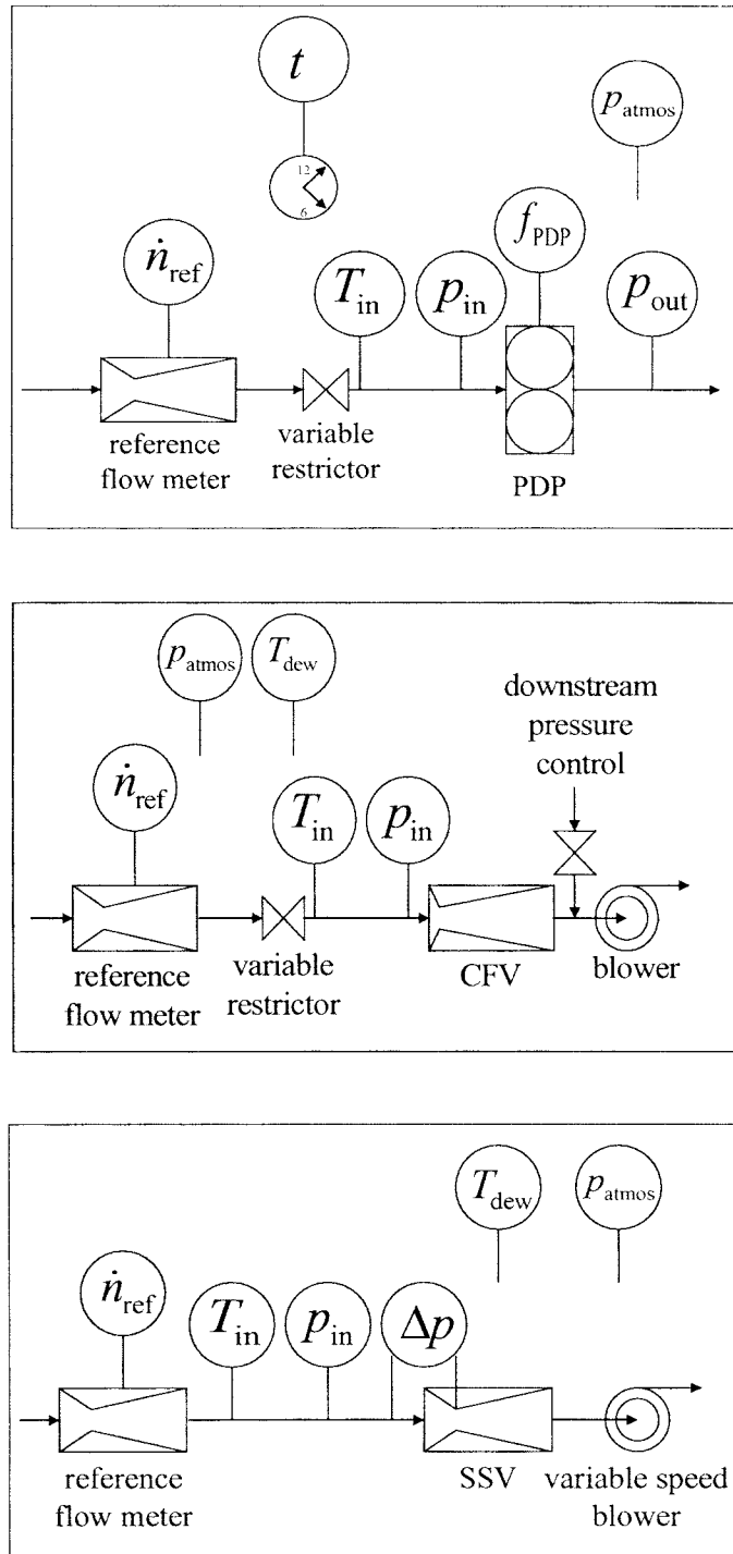
Figure 1 of 1065.340 CVS calibration configurations.
