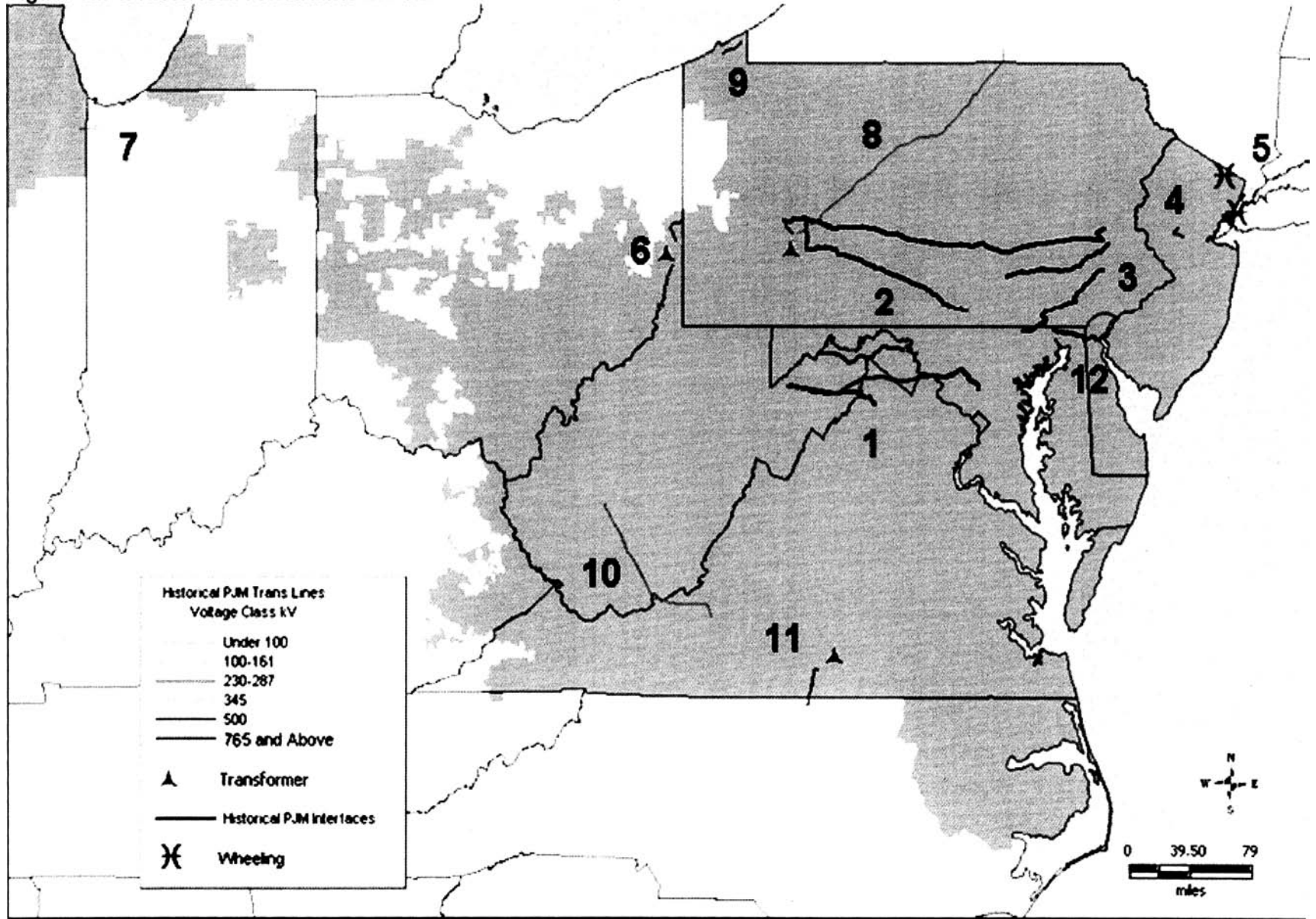
Figure VIII-1. Historical Constraints in PJM
