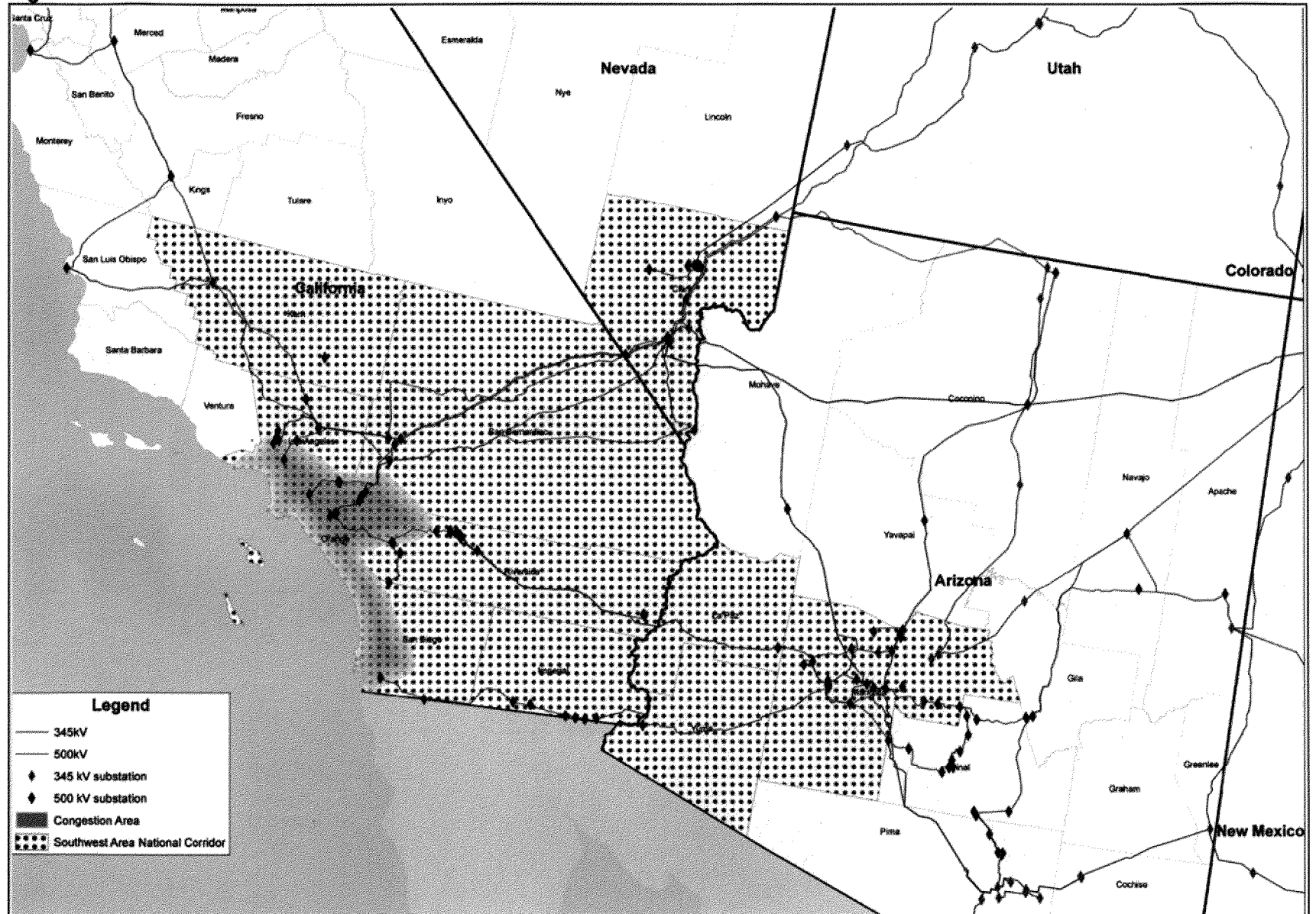
Figure IX-6. Draft Southwest Area National Corridor
