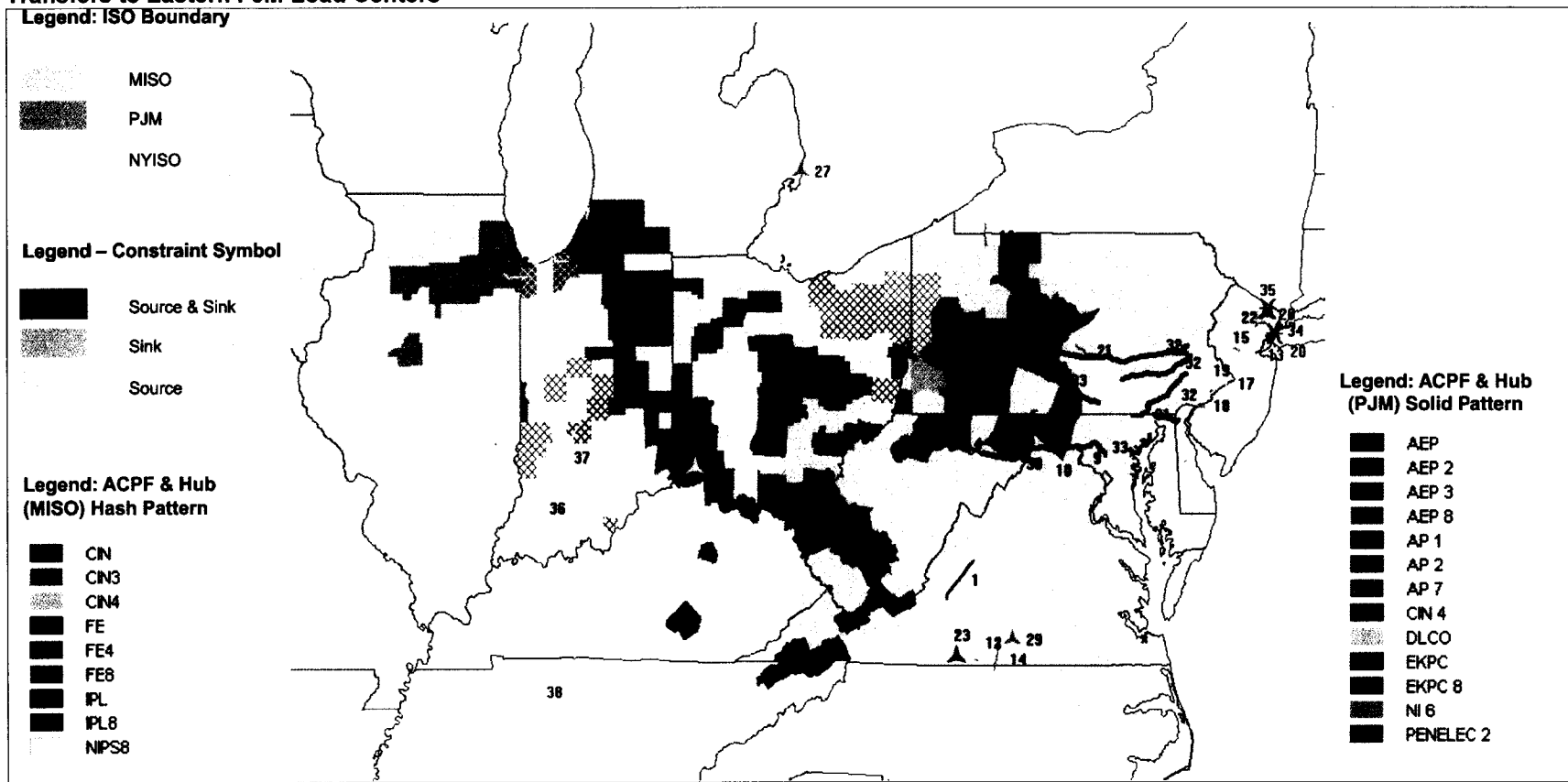
Figure VIII-4. Areas with Available Lower-Cost Generation in PJM and MISO and Transmission Constraints Limiting Electricity Transfers to Eastern PJM Load Centers
