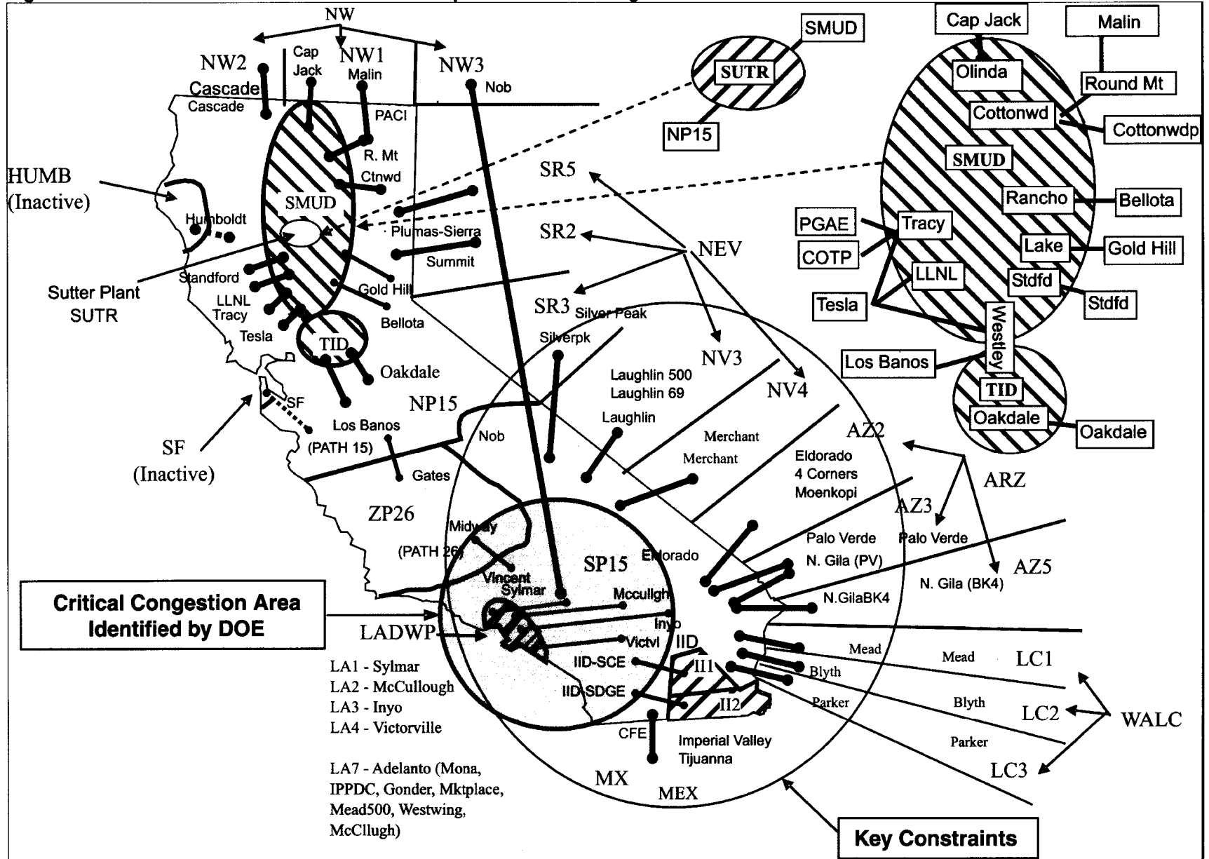
Figure IX-4. CAISO Active Zones and Branch Groups with Critical Congestion Area and Constraints
