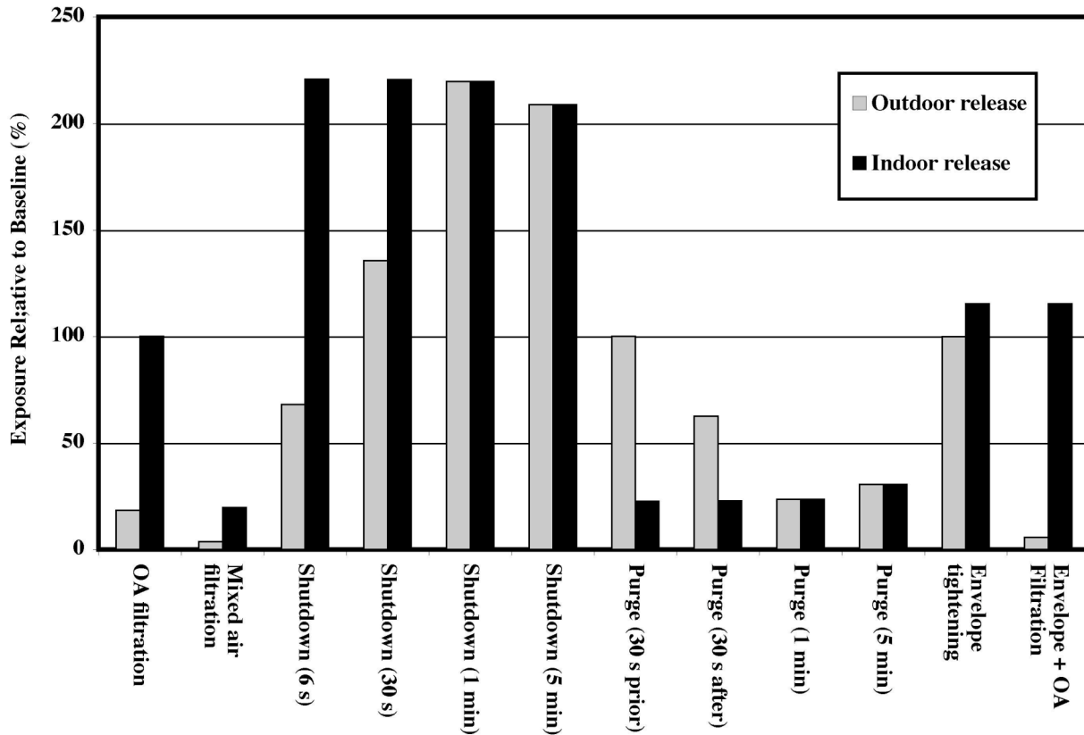
Figure 2 Single-zone exposure results for gaseous contaminant G
