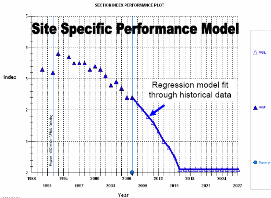
Figure 3. Example of a site-specific performance curve.
