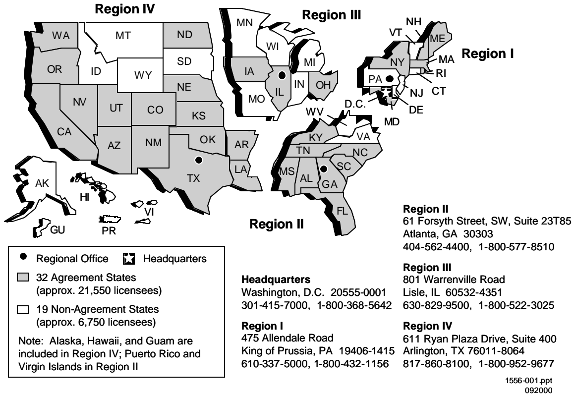
Figure 2.2 U.S. Map. Location of NRC Regional Offices and Agreement States.
