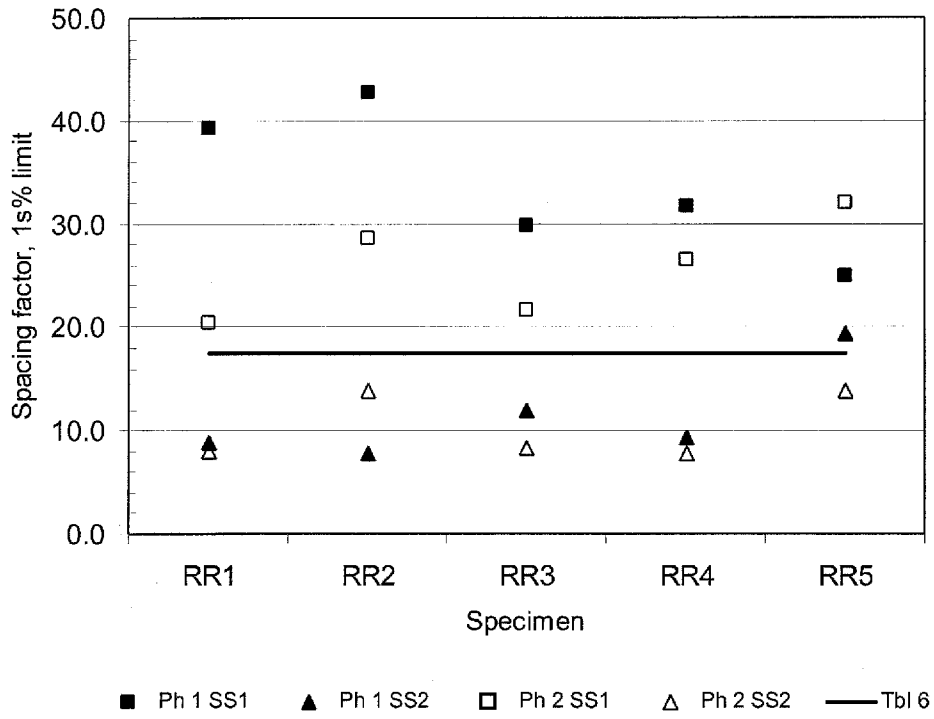
Figure 26. Multilaboratory precision for spacing factor
