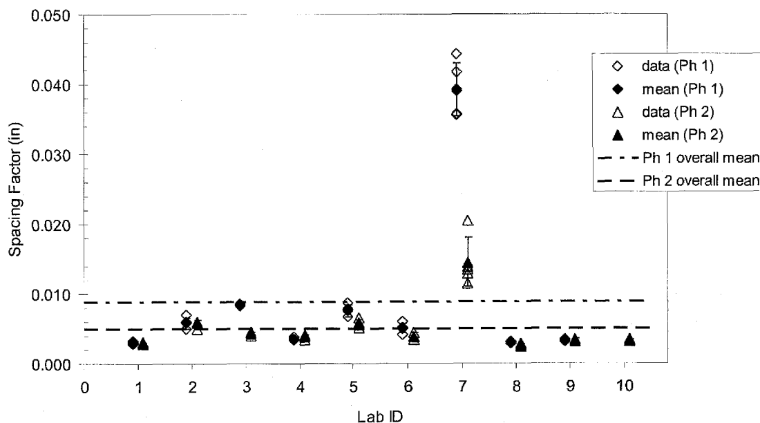
Figure 5. Within and between-laboratory spacing factor, RR2/RR2X
