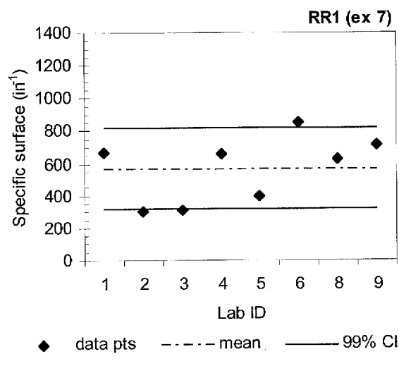
Figure 10. Between-laboratory comparison of air void parameters, RR1
