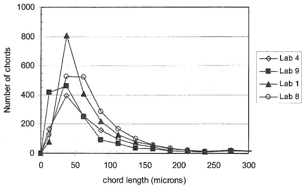
Figure 32. Lower end of chord distributions for RR5
