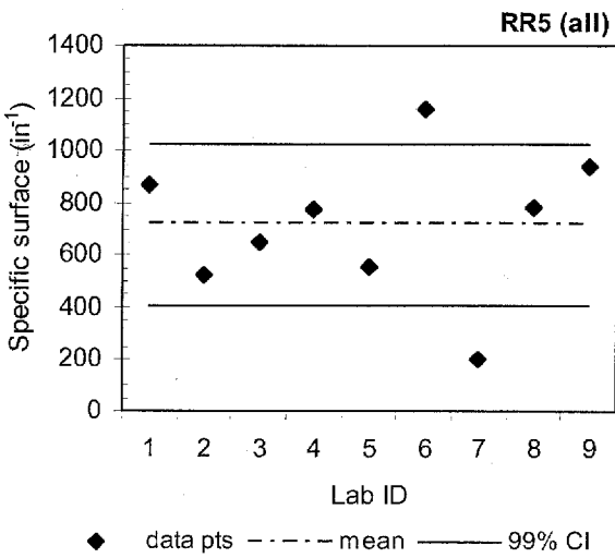
Figure 13. Between-laboratory comparison of air void parameters, RR5
