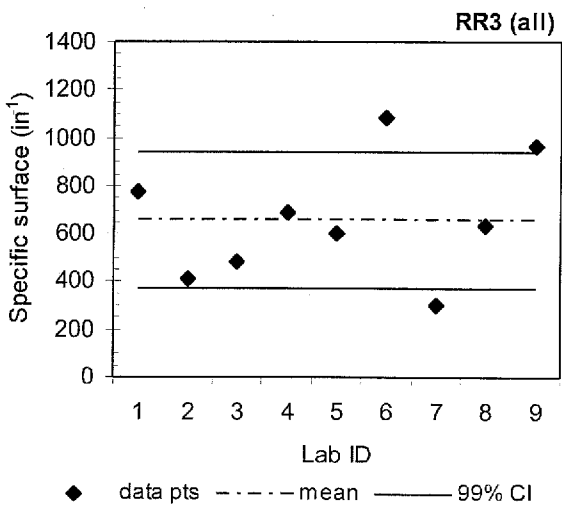
Figure 11. Between-laboratory comparison of air void parameters, RR3
