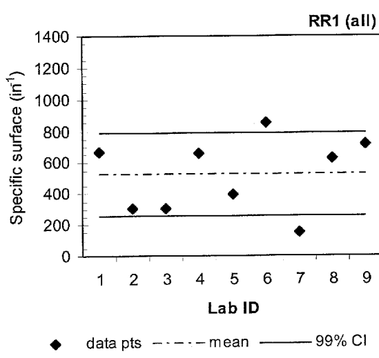
Figure 10. Between-laboratory comparison of air void parameters, RR1
