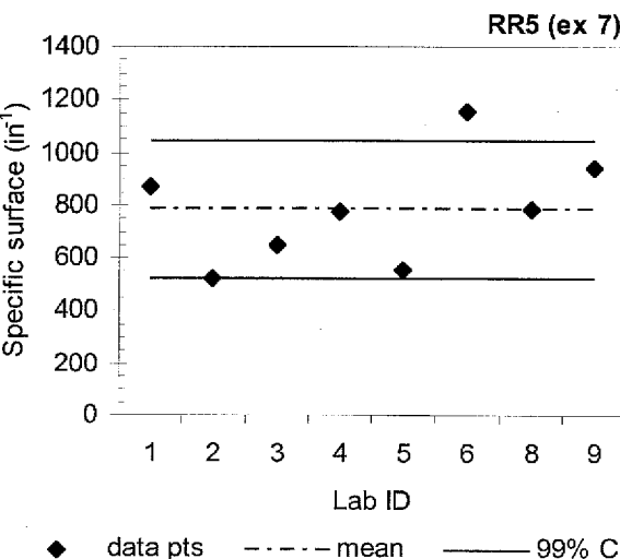
Figure 13. Between-laboratory comparison of air void parameters, RR5
