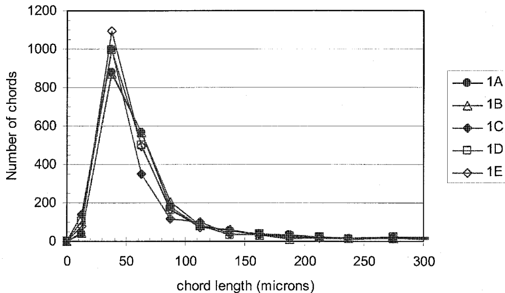
Figure 28. Chord distributions for RR2, Lab 1
