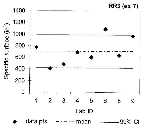
Figure 11. Between-laboratory comparison of air void parameters, RR3
