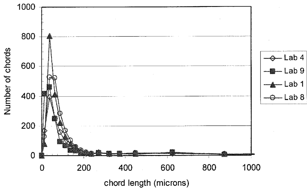
Figure 31. Chord distributions for RR5
