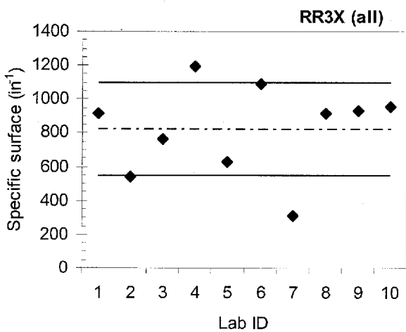
Figure 15. Between-laboratory comparison of air void parameters, RR3X
