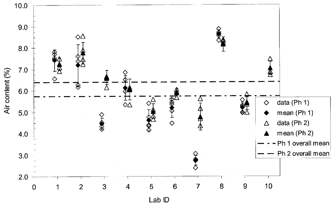
Figure 3. Within and between-laboratory air content, RR2/RR2X
