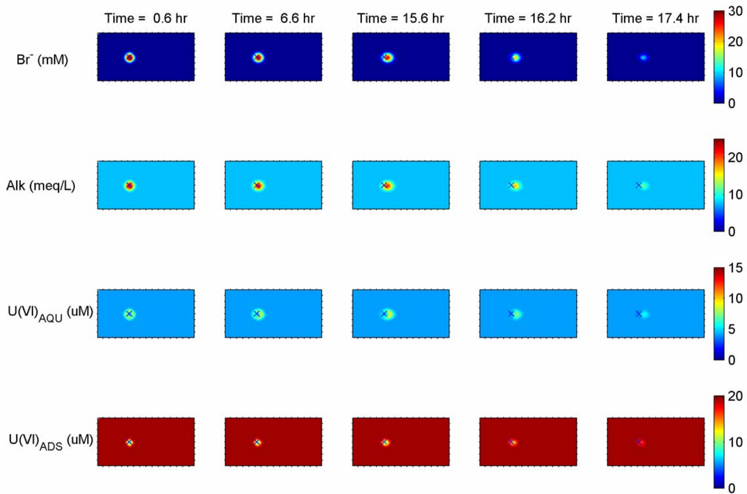
Figure 3.3. Temporal evolution of bromide, alkalinity, total dissolved U(VI) ( \text{U(VI)}_{\text{AQU}} ), and total adsorbed U(VI) ( \text{U(VI)}_{\text{ADS}} )
