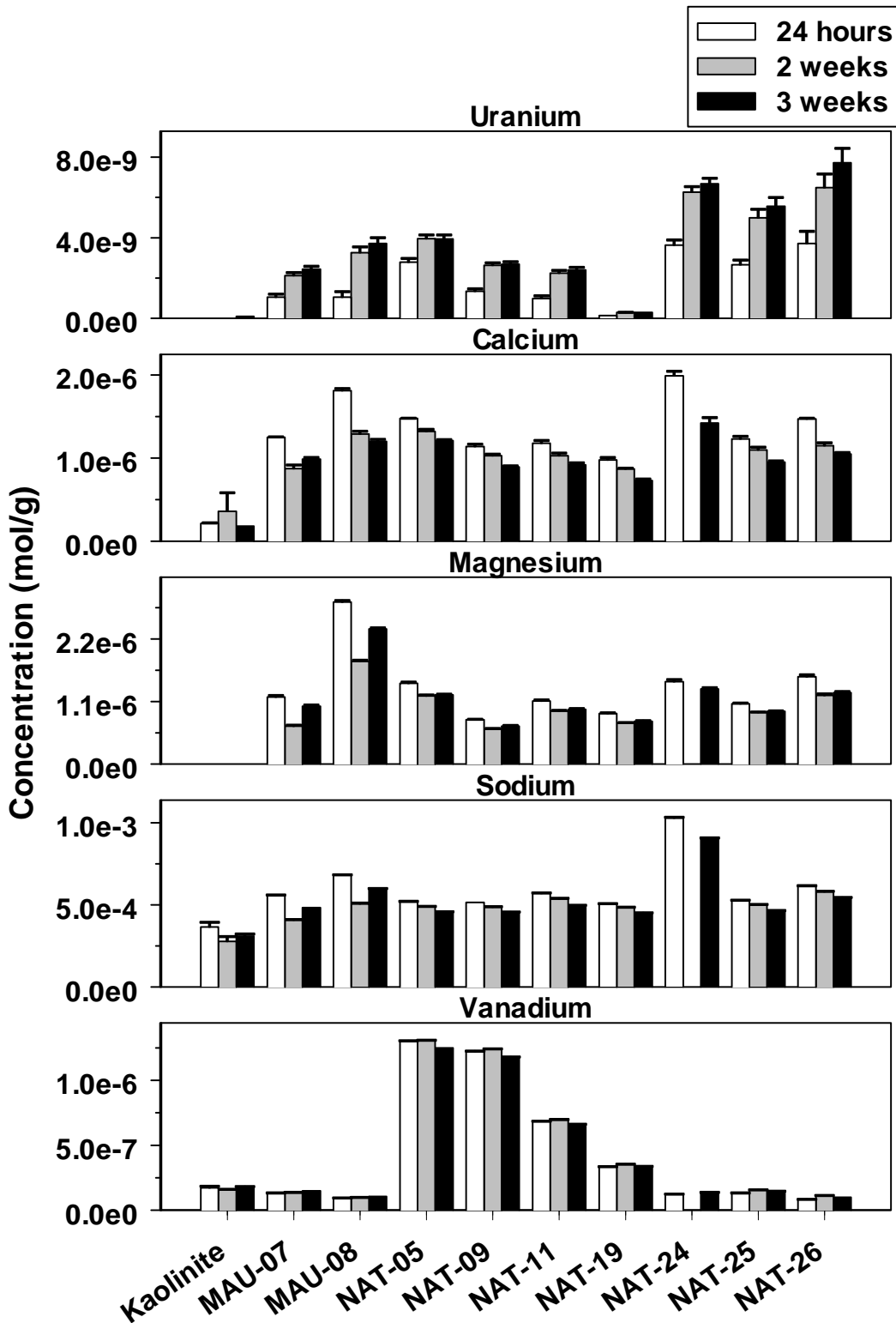
Figure 2.7. Concentrations of elements extracted at various times from kaolinite after exposure to groundwater for 1 month. For U(VI) and V, the data are corrected for the amounts of U(VI) and V that were present in entrained water when the kaolinite samples were collected. None of the other elements were corrected for the amount present in entrained water. Sample labeled 'Kaolinite' shows data for extractions without field deployment.
