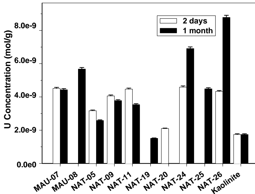
Figure 2.4. Comparison of U(VI) concentrations for kaolinite samples deployed in dialysis tubing and placed in wells for 2 days or 1 month. U(VI) concentrations in (A) carbonate solution extracts, and (B) nitric acid extracts. Sample labeled 'Kaolinite' shows data for extractions without field deployment.
