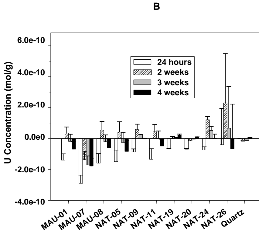
Figure 2.9. Calculated amounts of U(VI) extracted by carbonate solution from quartz samples for various extraction times. The data presented represent the average from two dialysis bags containing quartz that were deployed in each well. Part (A) shows the amount of U(VI) extracted without correction for U(VI) in the water entrained with the quartz samples. Part (B) illustrates the same data after the correction is applied.
