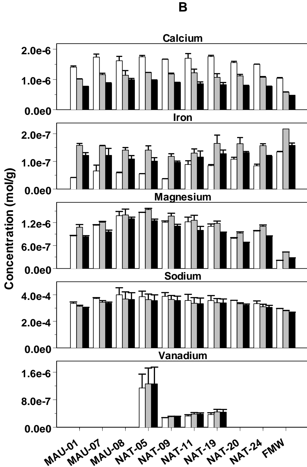
Figure 2.16 (continued). The concentrations of various elements dissolved in carbonate solution extracts of 40-Mile Wash sediments. Part (A) shows U, Part (B) shows Ca, Fe, Mg, Na, and V, and Part (C) shows individual replicate samples for U and V. Parts (A) and (B) show the average of two replicate samples. U and V data are corrected for the amount present in entrained water. Data below the detection limit for V are not plotted. Sample labeled 'FMW' shows data for extractions of the 40-Mile Wash sediment composite without field deployment.
