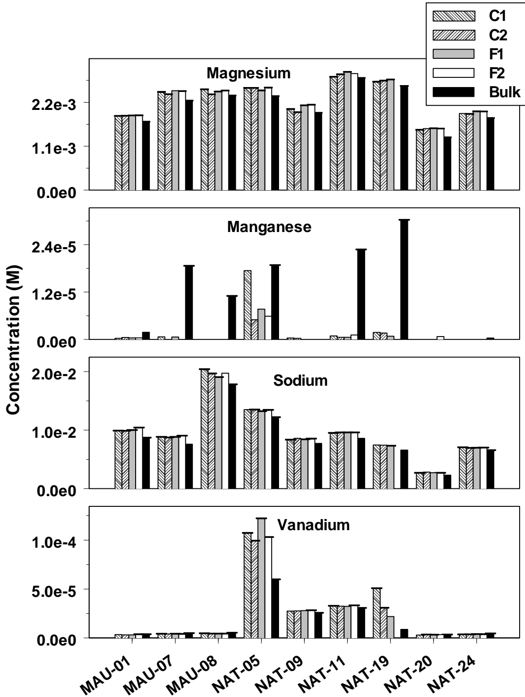
Figure 2.3 (continued). Comparison of various elemental concentrations measured in replicate clinoptilolite (C1, C2) and 40-Mile Wash composite (F1, F2) dialysis bags compared with bulk groundwater (bulk) in December 2005. Data below the detection limit for Fe ( 1.8 \times 10^{-6} M), K ( 2.0 \times 10^{-4} M), and Mn ( 2.5 \times 10^{-7} M) is not plotted.
