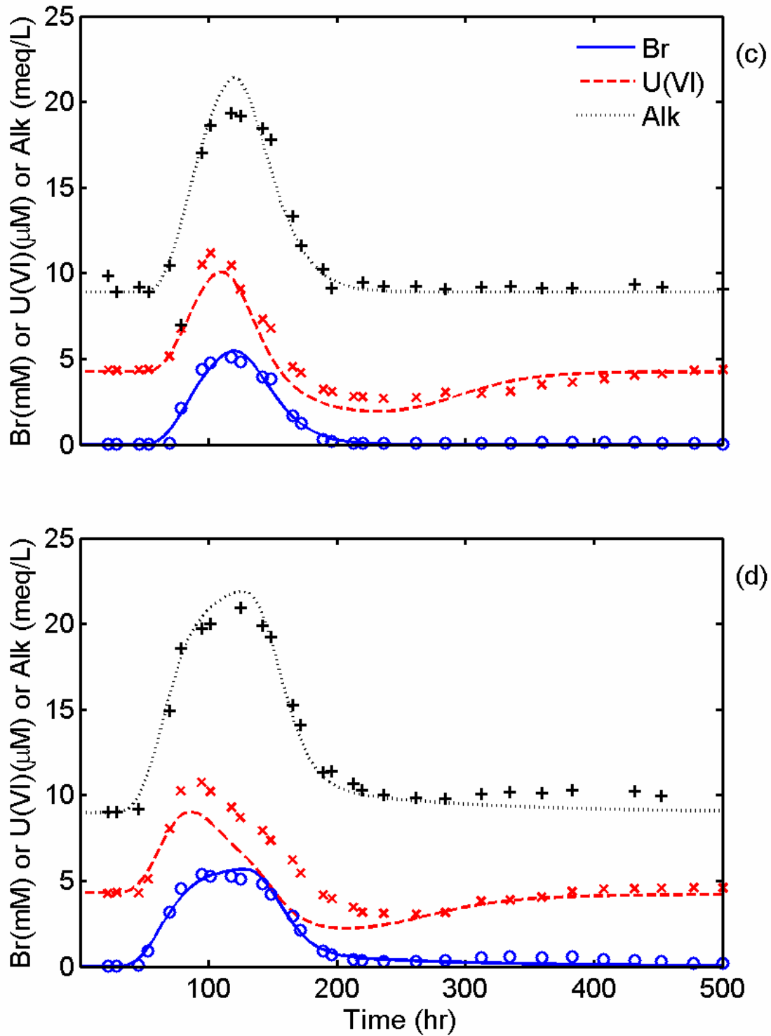
Figure 5-6 (cont). Observed and simulated bromide, U(VI) and alkalinity concentrations in migration test MT3 at observations wells (c) M2, and (d) N2.
