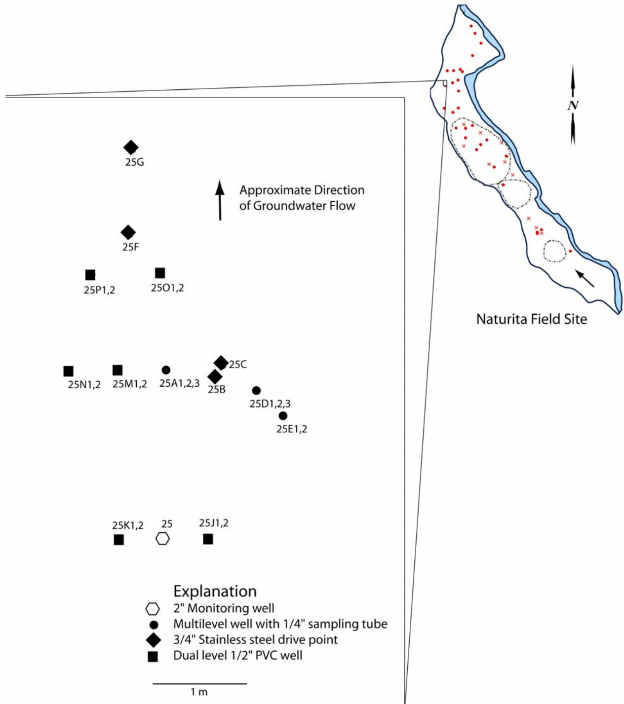
Figure 4.1. Map of the small-scale tracer test site developed near well NAT25. The numbers after the well designations indicate the different sampling levels, with 1 being the deepest screened interval.
