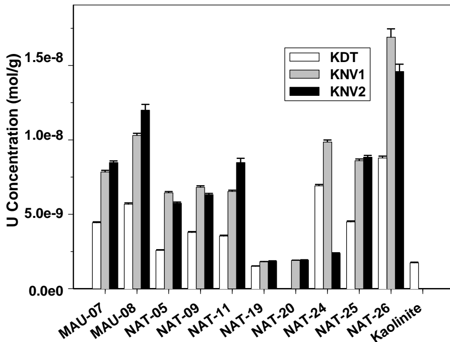
Figure 2.5. Comparison of U(VI) extracted from kaolinite deployed in different sample holder types: KDT (dialysis tubing) and KNV (nylon vial), with U(VI) extracted by carbonate solution (A) and nitric acid (B). Sample labeled ‘Kaolinite’ shows data for extractions without field deployment.
