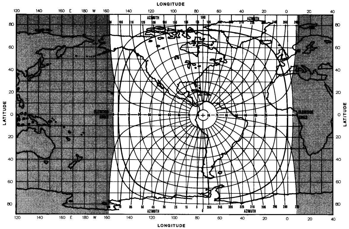
Figure 8. Pointing angles for GOES/East.
