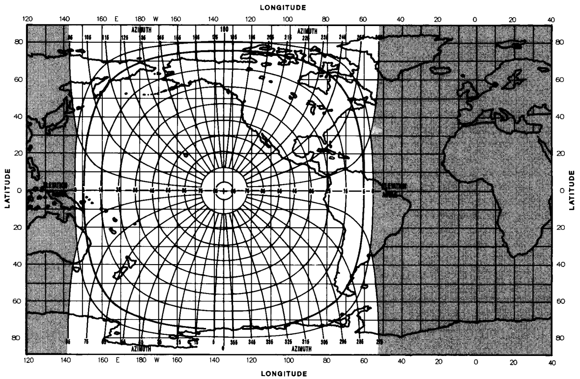
Figure 9. Pointing angles for GOES/West.
