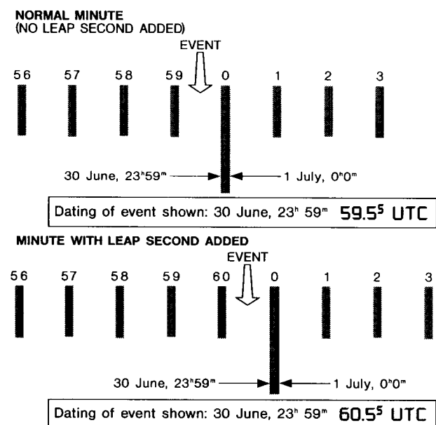
Figure A. Dating of events near a leap second.
