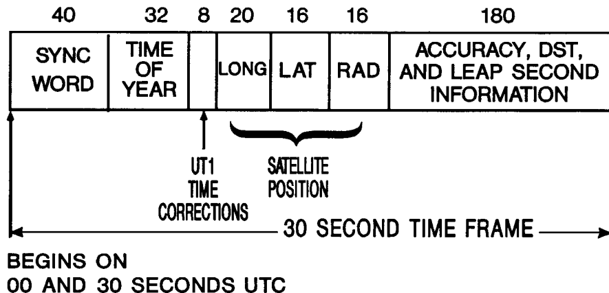
Figure D. (Top) GOES satellite interrogation channel format. (Bottom) GOES time code format.
