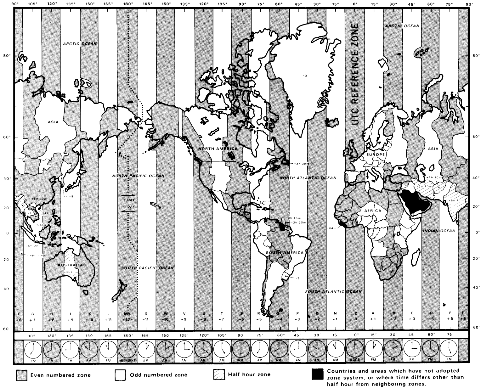
Figure 3. Standard time zones of the world and their relationship to UTC.
