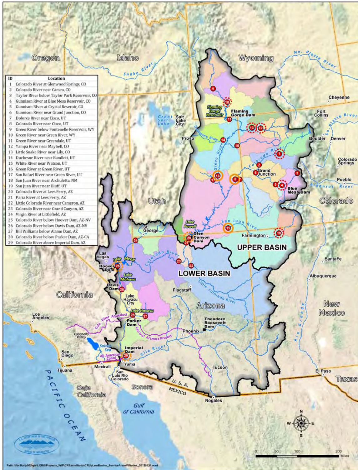
FIGURE B-3 Colorado River Basin and 29 Natural Flow Locations (Source: Reclamation, 2011) Circled stations are used for climate and streamflow in this report; dashed circles are used to describe climate, and solid circled stations are used to describe streamflows.
