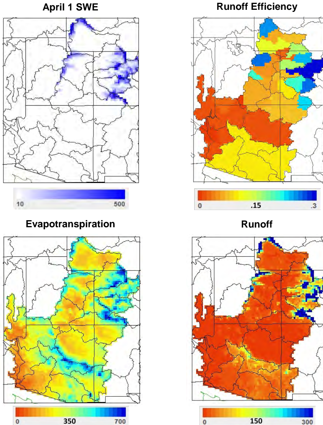
FIGURE B-8 Estimated Average Annual ET and Runoff (millimeters), April 1 SWE (millimeters), and Annual Average Runoff Efficiency (fraction of precipitation converted into runoff) for 1971–2000 Derived from historical VIC simulations.
