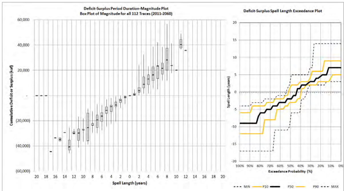
FIGURE B-51 Simulated Deficit and Surplus Spell Length and Magnitude for all 112 Climate Projections (Threshold Defined as Individual Projection Mean for 2011–2060) Box plots show the median (dash), 25th h – 75th percentile band (shading), and max/min (whiskers).
