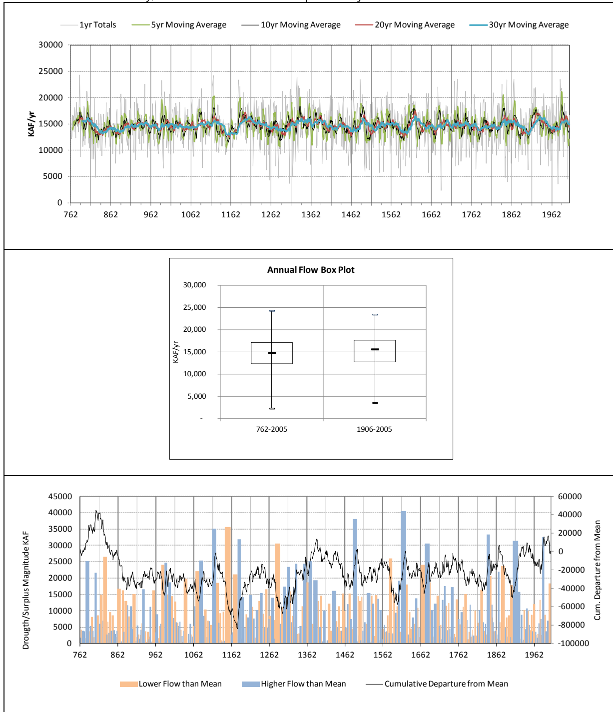
FIGURE B-19 Colorado River at Lees Ferry, Arizona Paleo Streamflow Snapshot Analysis
