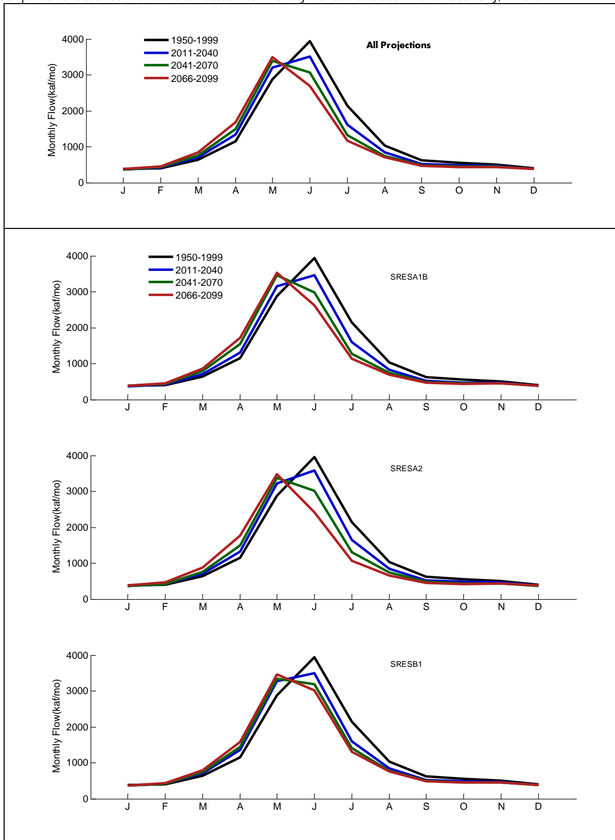
FIGURE B-49 Comparison of Observed and Future Simulated Mean Monthly Flows at Colorado River at Lees Ferry, Arizona
