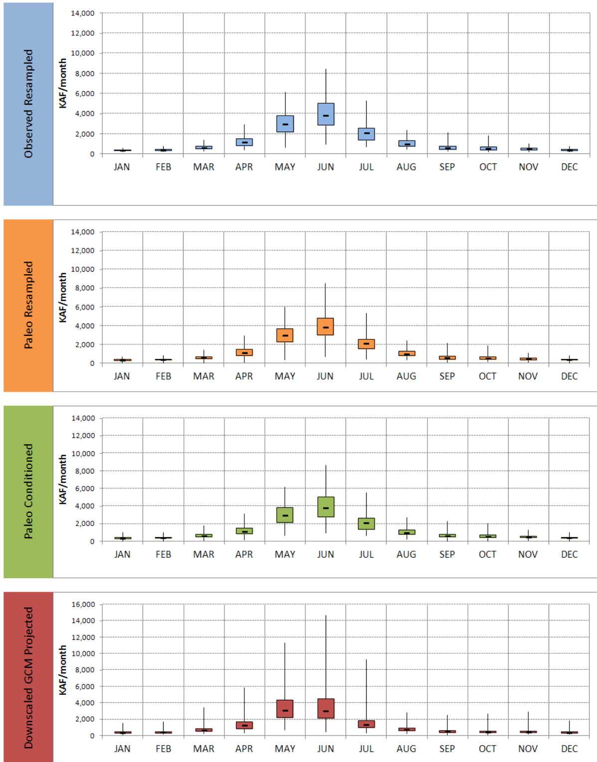
FIGURE B-55 Monthly Colorado River at Lees Ferry, Arizona Natural Flow Variability for Supply Scenarios (for 2011–2060) Figure shows the median (dash), 25th – 75th percentile band (shading), and max/min (whiskers).
