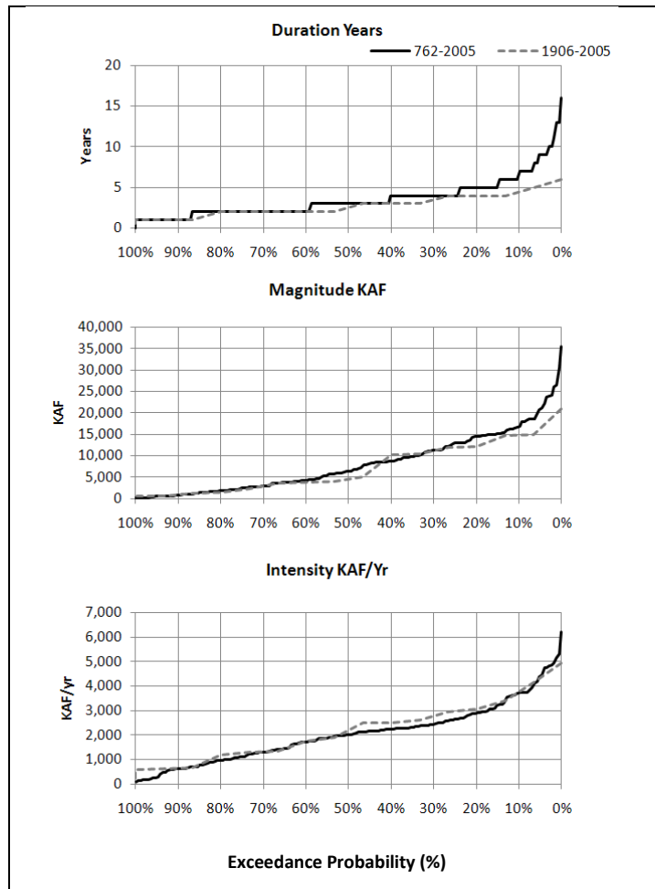
FIGURE B-20 Comparison of Drought Characteristics between a Segment of the Observed Period (1906–2005) and the Paleo Period (762–2005)
