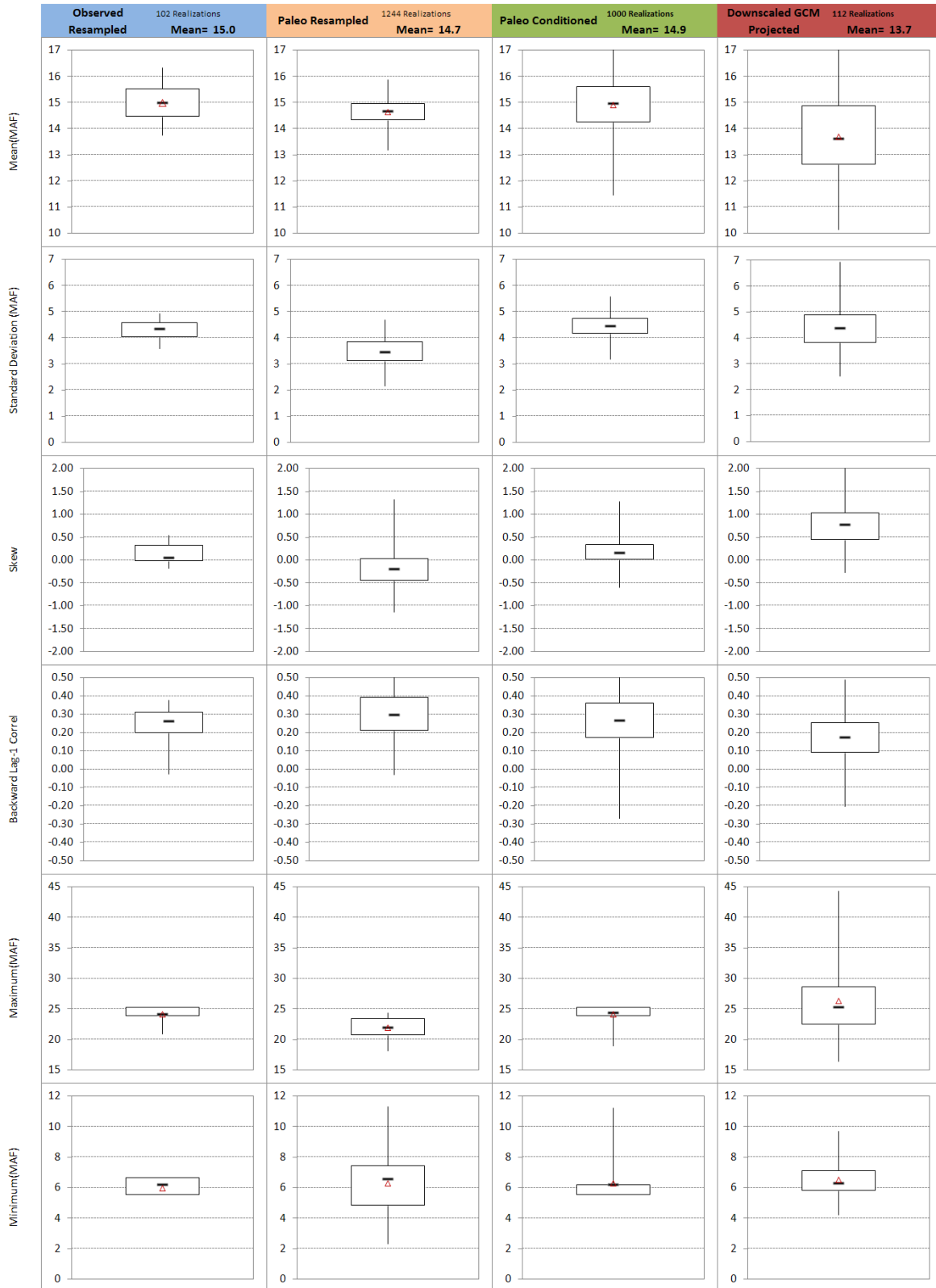
FIGURE B-53 Summary Statistics for Annual Colorado River at Lees Ferry, Arizona Natural Flows for Supply Scenarios (for 2011-2060) Figure shows the median (dash), 25th – 75th percentile band (box), and max/min (whiskers).
