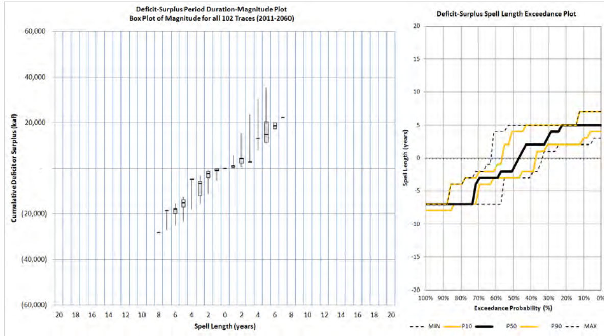
FIGURE B-25 Simulated Deficit and Surplus Spell Length and Magnitude for all 102 Realizations in the Observed Resampled Scenario Box plots show the median (dash), 25th – 75th percentile band (shading), and max/min (whiskers).
