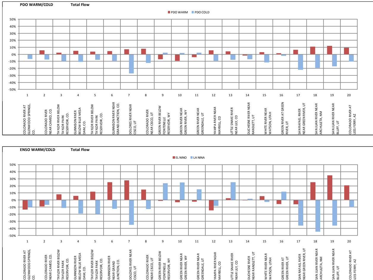
FIGURE B-11 Median Change in Flows from Long-term Average for Warm and Cold PDO (top) and ENSO (bottom) Years
