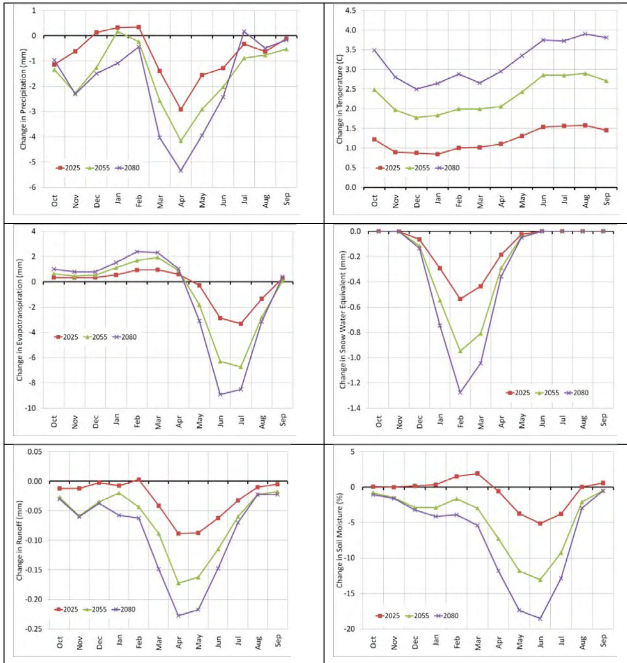
FIGURE B-43 Projected Change in Mean Monthly Climatological and Hydrologic Parameters 25-Colorado River at Hoover Dam.
