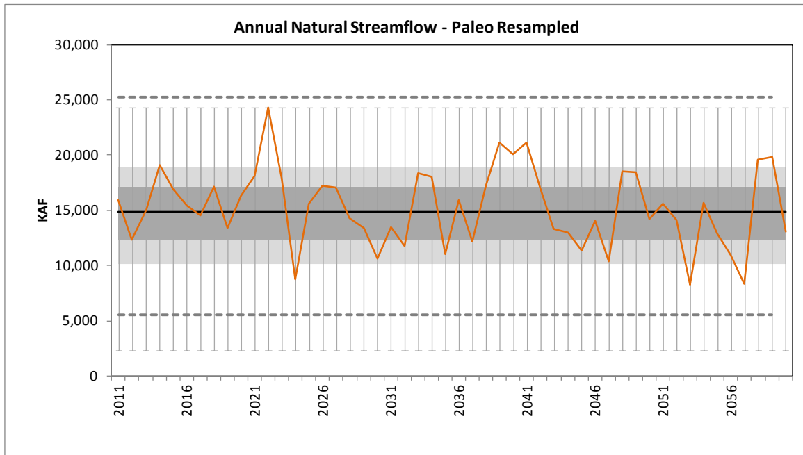
FIGURE B-27 Simulated Annual Colorado River at Lees Ferry, Arizona Natural Flow Statistics for 1,244 Traces, 2011–2060 Figure shows the median (line), 25th – 75th percentile band (dark shading), 10th – 90th percentile band (light shading), max/min (whiskers), and 1906 – 2007 observed min and max (dashed lines). The bolded line indicates a representative trace.
