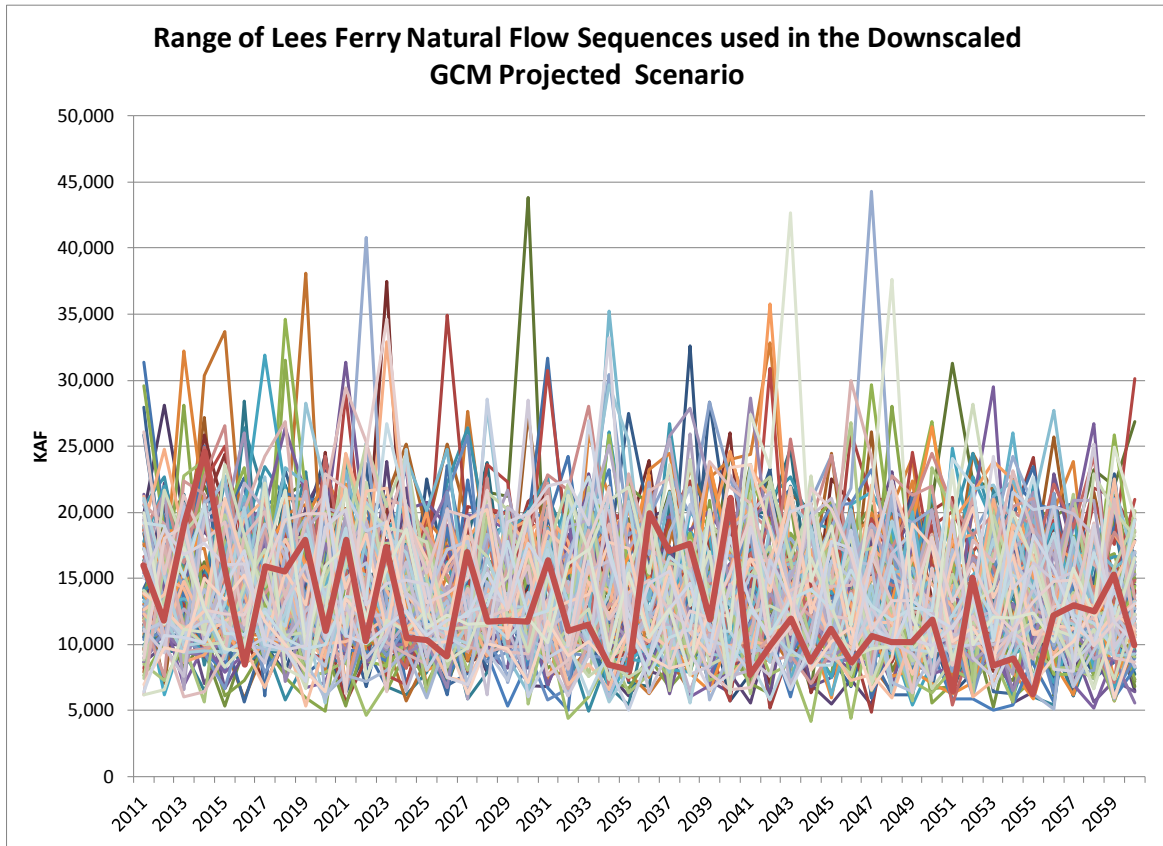
FIGURE B-44 Colorado River at Lees Ferry, Arizona Natural Flow for 112 Sequences for the Downscaled GCM Projected Scenario The bolded line indicates a representative trace.
