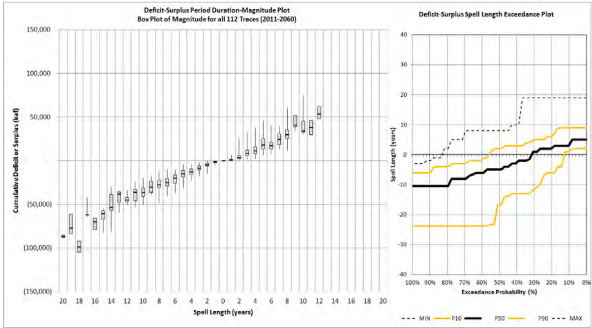
FIGURE B-50 Simulated Deficit and Surplus Spell Length and Magnitude for All 112 Climate Projections (Threshold Defined As 1906–2007 Mean Annual Flow ~ 15 maf) Box plots show the median (dash), 25th – 75th percentile band (shading), and max/min (whiskers).
