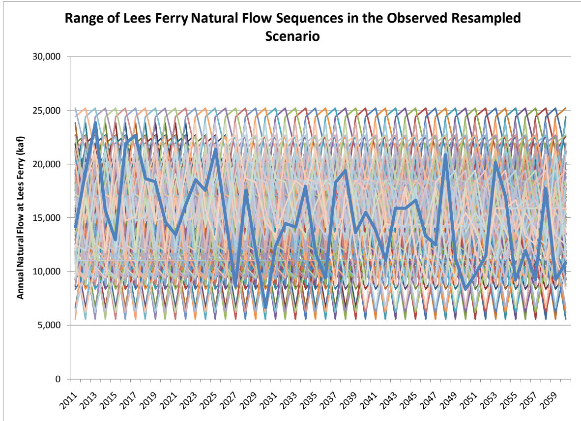
FIGURE B-21 Colorado River at Lees Ferry, Arizona Natural Flow for 102 Sequences for the Observed Resampled Scenario The bolded line indicates a representative trace.
