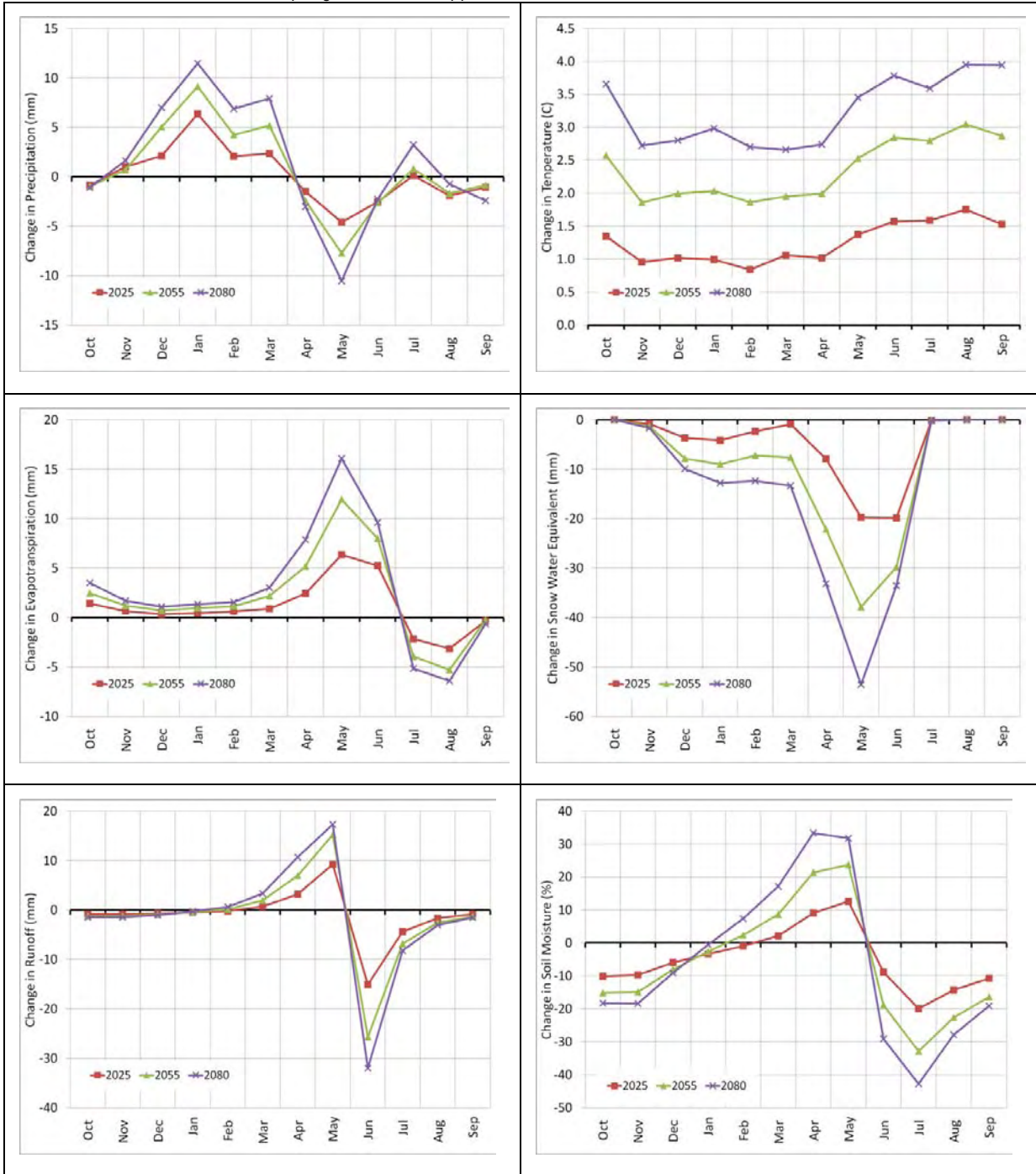
FIGURE B-42 Projected Change in Mean Monthly Climatological and Hydrologic Parameters 01-Colorado River at Glenwood Springs, Colorado (Upper Basin).
