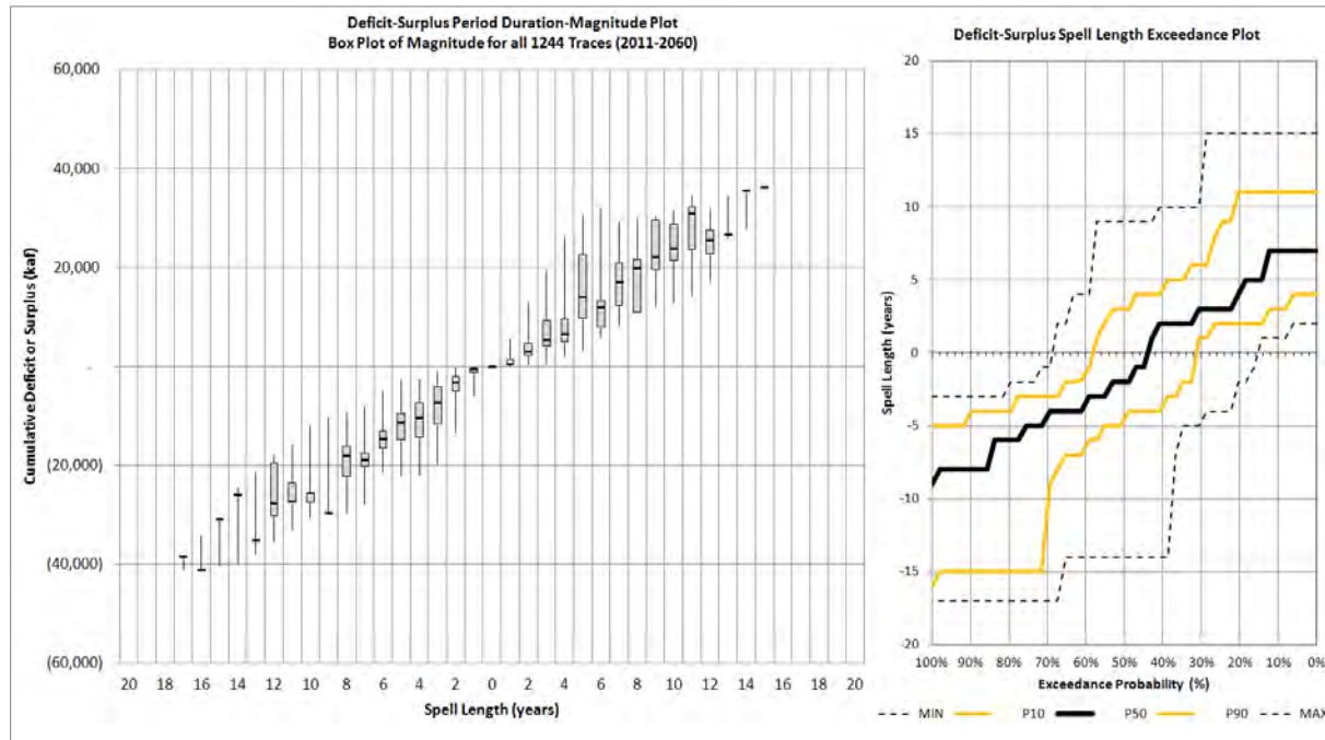
FIGURE B-30 Simulated Deficit and Surplus Spell Length and Magnitude for all 1,244 Realizations in the Paleo Resampled Scenario Box plots show the median (dash), 25th – 75th percentile band (shading), and max/min (whiskers).
