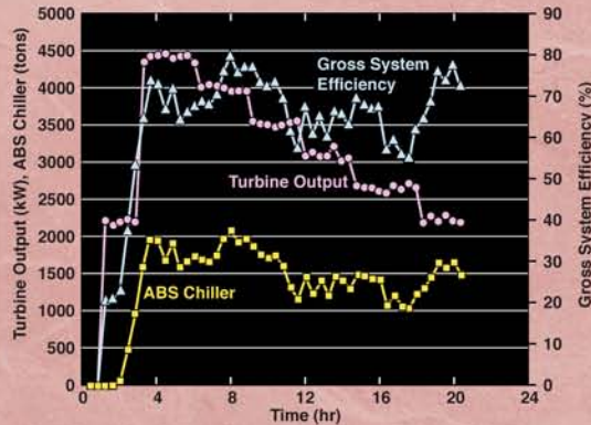
Gross efficiency for the IES reaches 80%, even when the turbine-generator is operated at part load.
