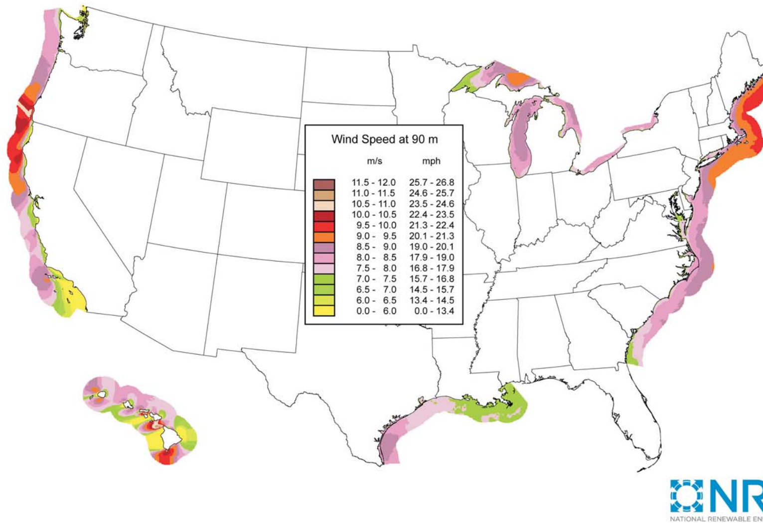
Figure 4.17 Offshore Wind Resources
