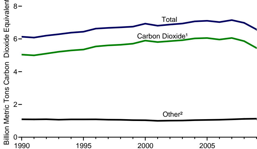
Based on Global Warming Potential, 1990-2009
