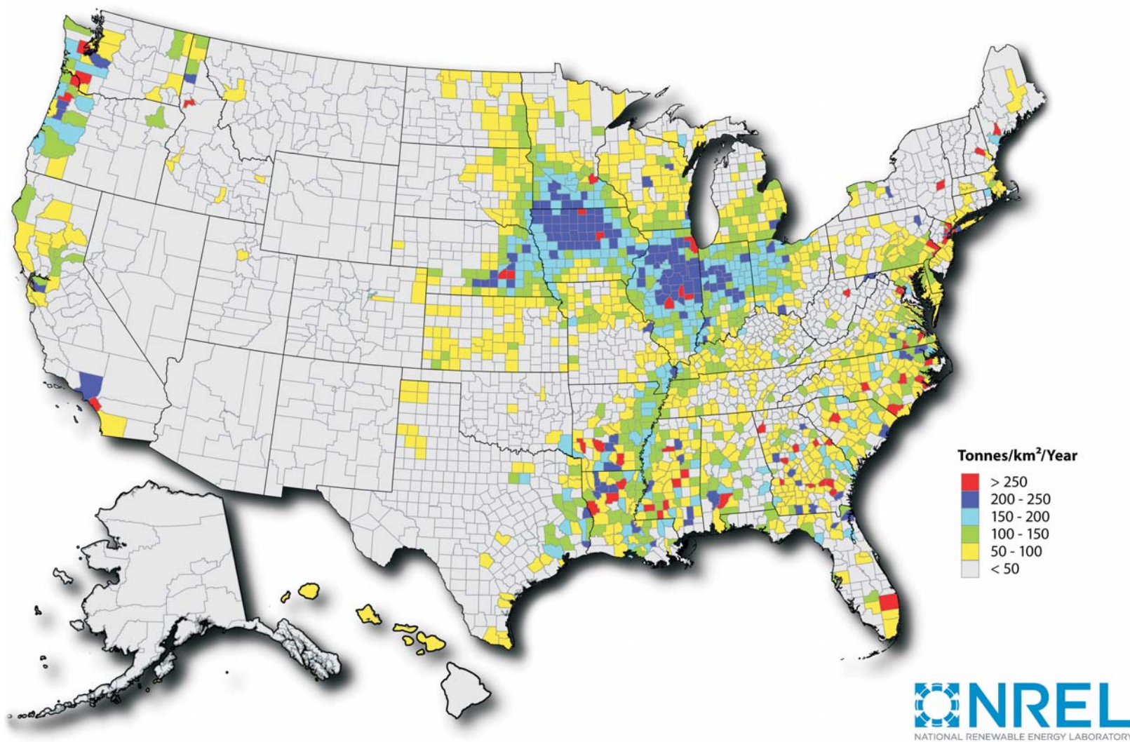
Figure 4.19 Biomass Resources
