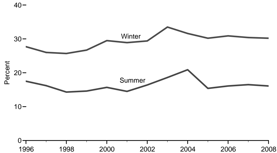
Capacity Margin, 1996-2008
