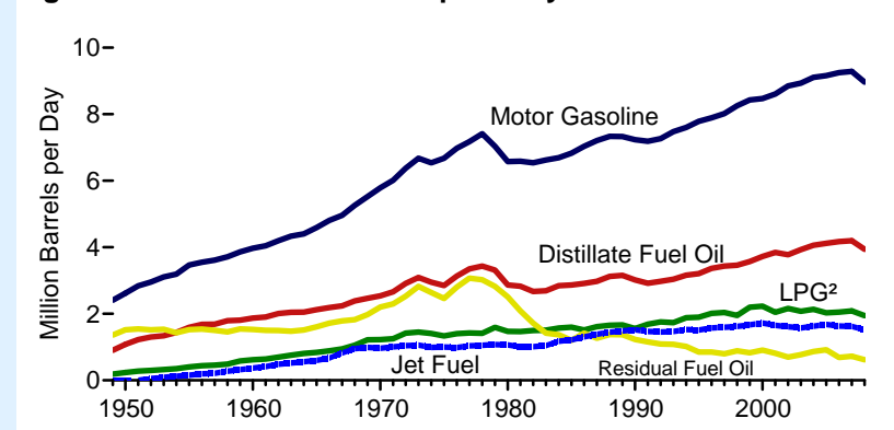
Figure 19. Petroleum Consumption 1 by Selected Product
