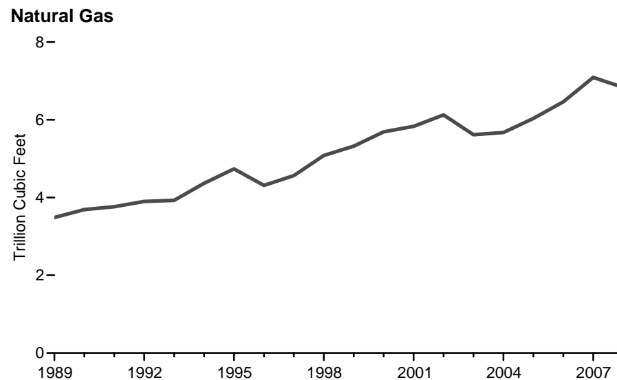
Figure 8.5a Consumption of Combustible Fuels for Electricity Generation, 1989-2008
