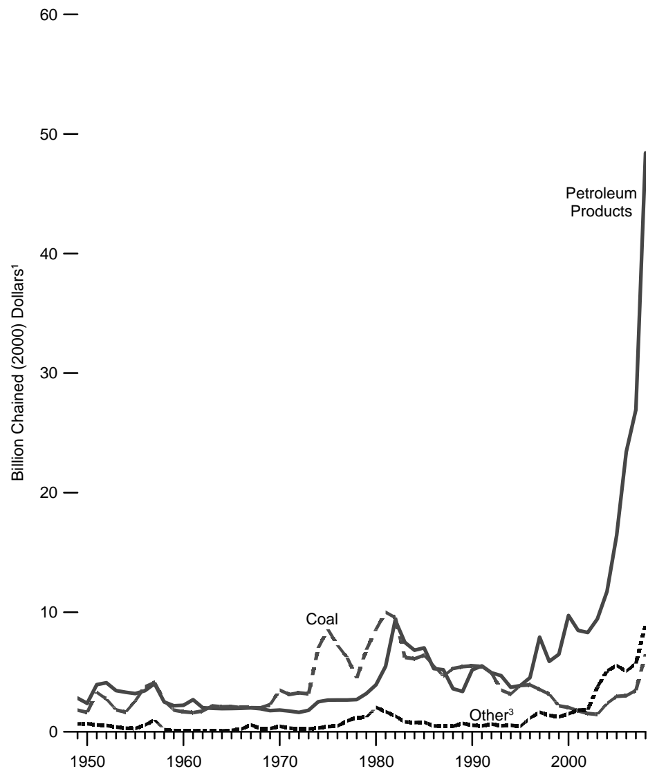
By Fuel, 1949-2008
