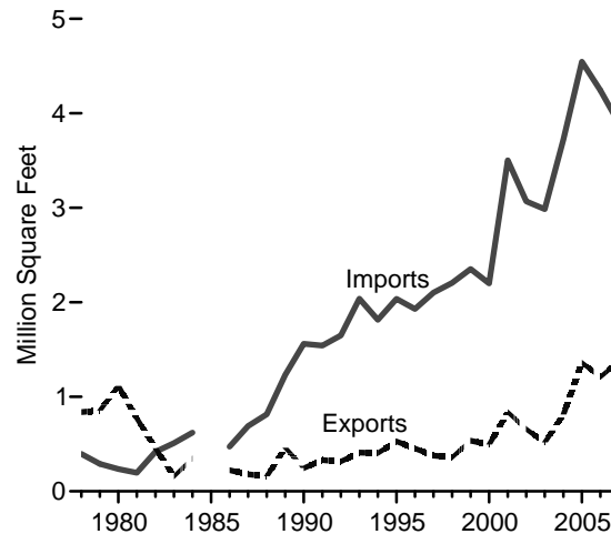
Trade, 1978-1984 and 1986-2007
