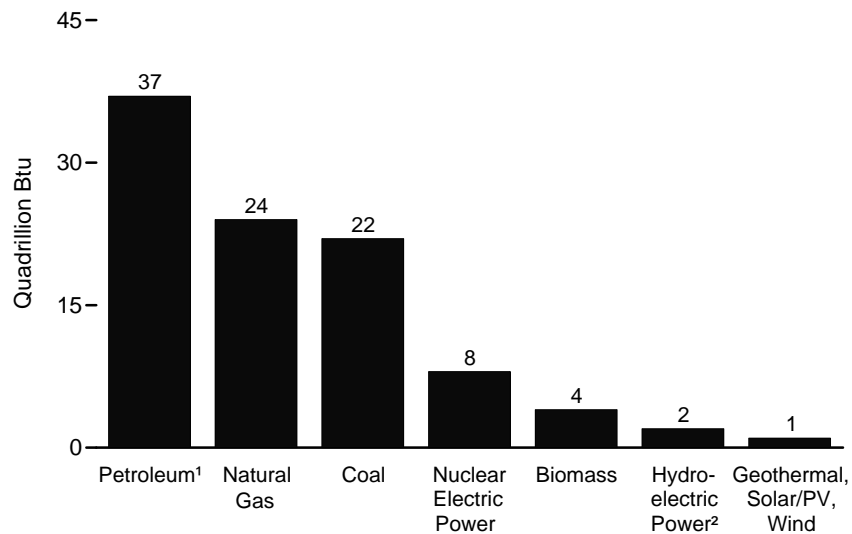
By Source, 2008
