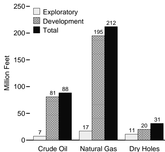
Footage Drilled, 2008
