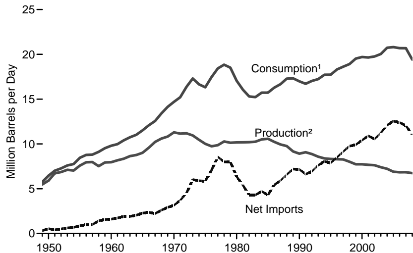
Overview, 1949-2008
