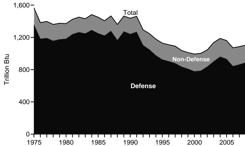
Total and U.S. Department of Defense, 1975-2008
