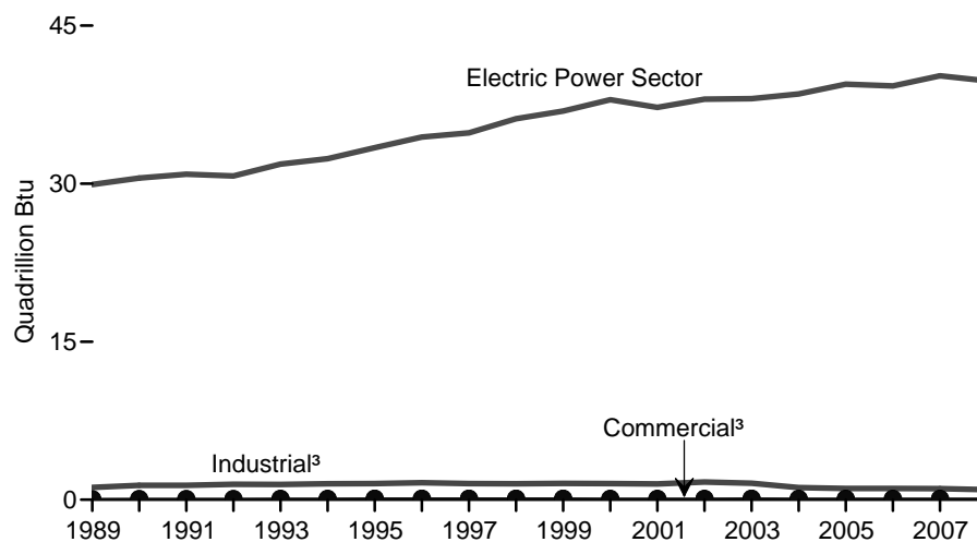
By Sector, 1989-2008
