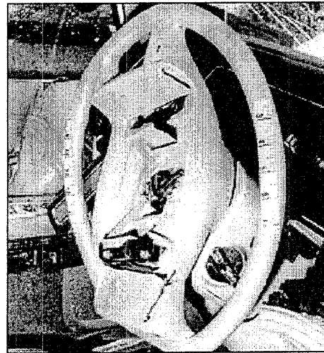
Severe steering wheel deformation from driver contact.
