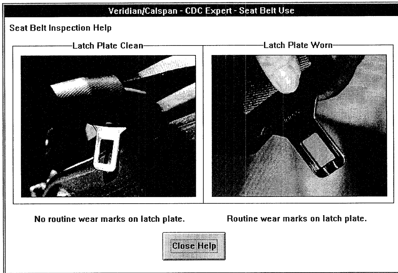
Figure 5. Routine wear marks on belt help screen.
