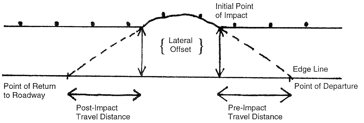
Figure 15. Distance data required for crashes producing symmetric guardrail damage patterns.
