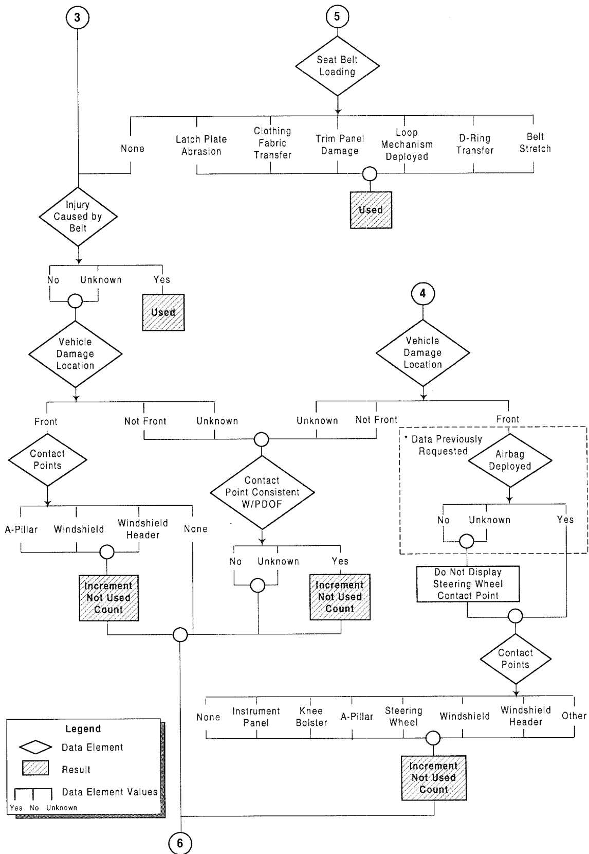
Figure 6. Seat Belt Use decision tree (continued).
