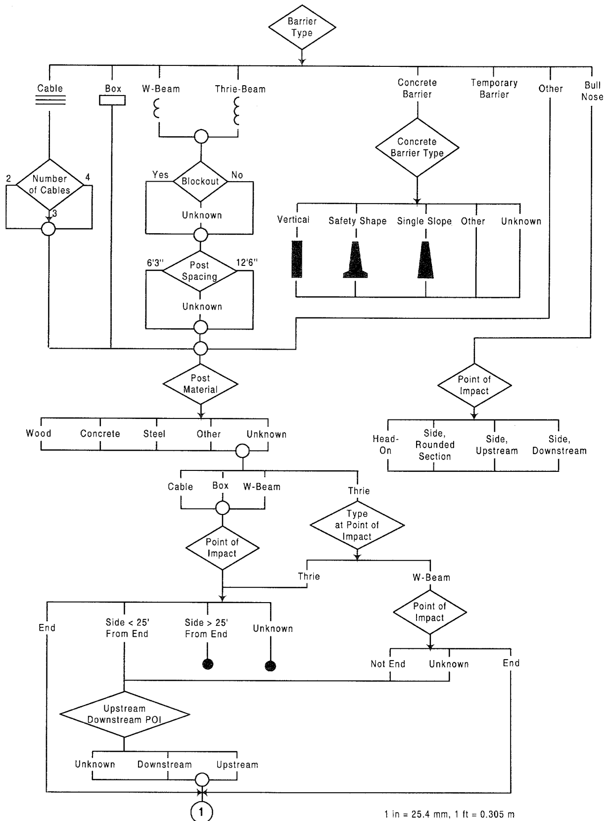
Figure 10a. Roadside Barrier main section type and point of impact.
