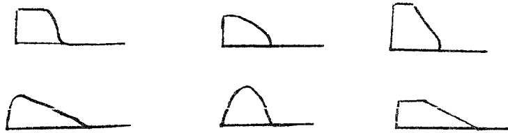
Mountable curbs.
