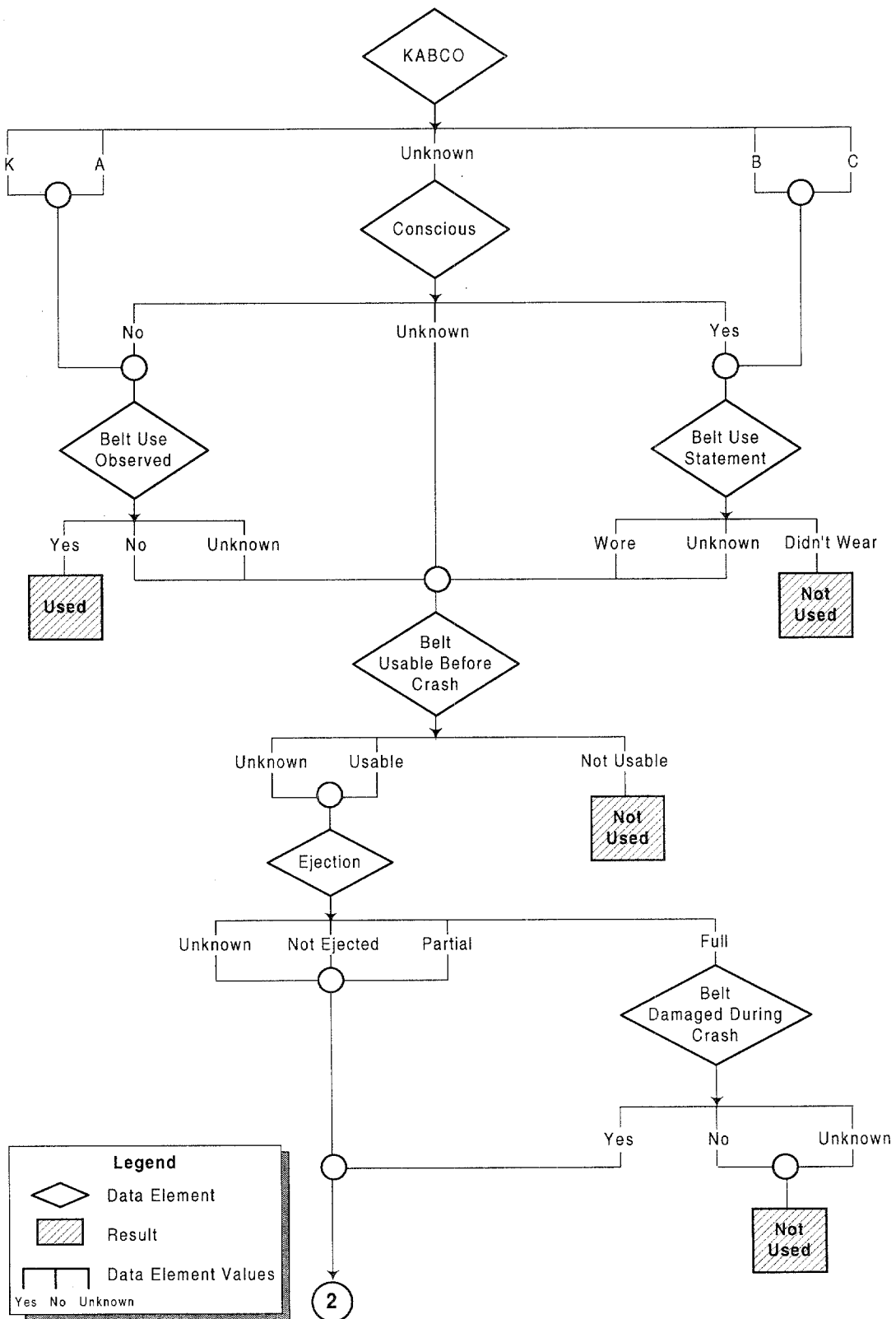
Figure 6. Seat Belt Use decision tree.
