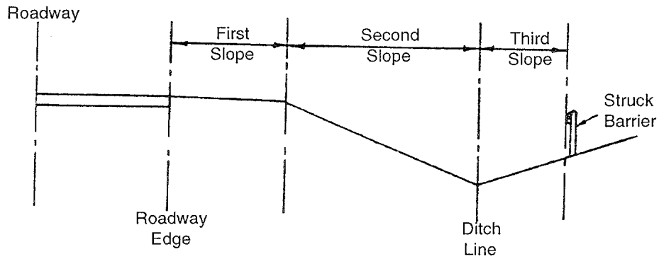
Three slopes.
