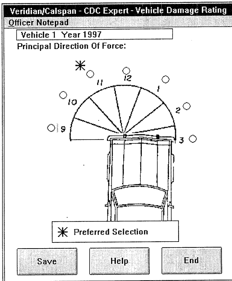
Figure 9b. Principal Direction of Force screen.
