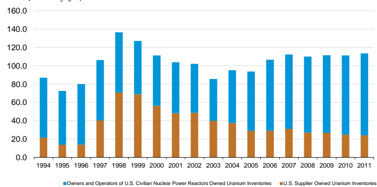
Figure S6. Total commercial uranium inventories of U.S. suppliers and owners and operators of U.S. civilian nuclear power reactors, 1994-2011
