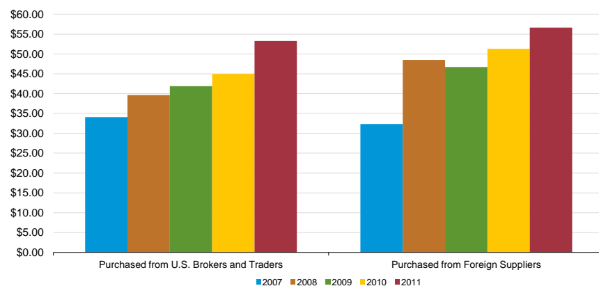
Figure 2. Weighted-average price of uranium purchased by owners and operators of U.S. civilian nuclear power reactors by supplier and delivery year, 2007-2011
