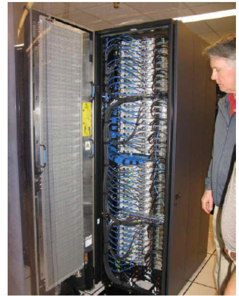
Figure 3: Inside rack RDHx, open 90°
