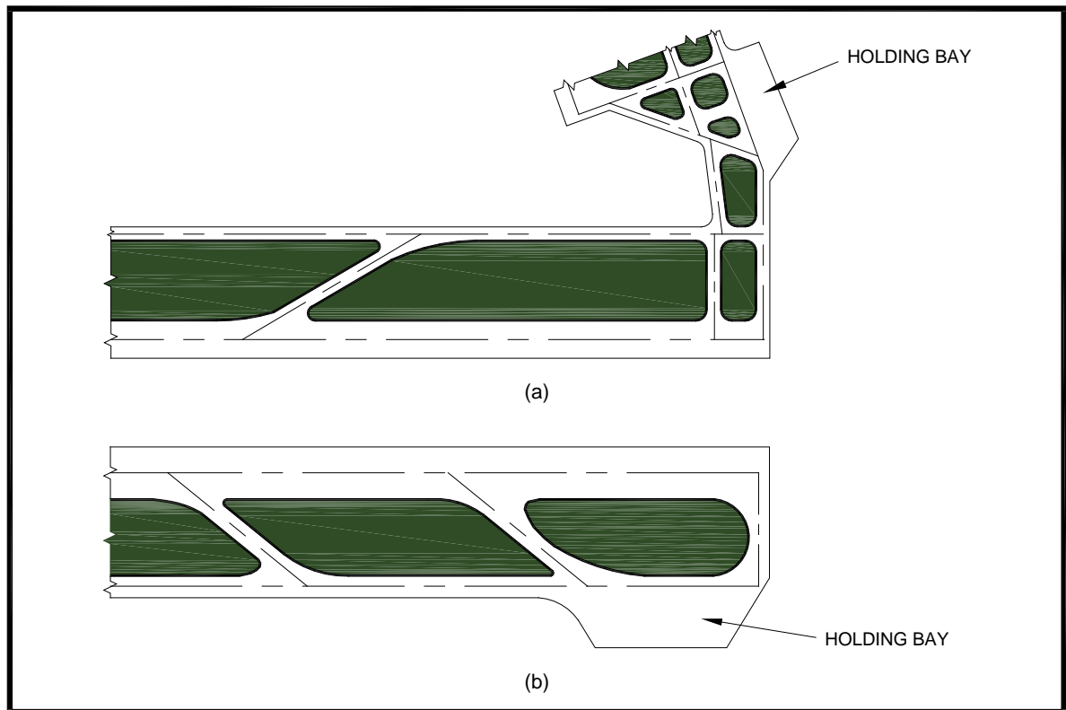
Figure 4-8. Two Typical Holding Bay Configurations
