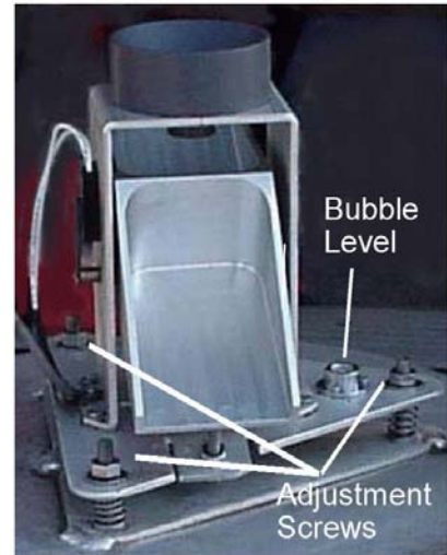
Figure F- 14. Tipping bucket level adjustments.
