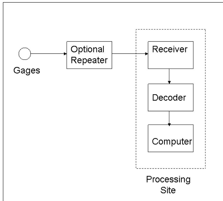
Figure 3- 4. ALERT System Configuration.
