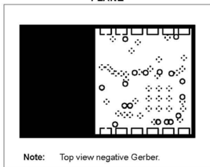
FIGURE 2-4: LAYER 2 – GROUND PLANE
