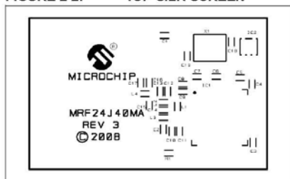
FIGURE 2-3: TOP COPPER
