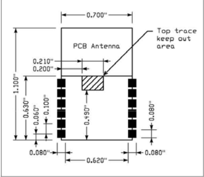
FIGURE 1-4: RECOMMENDED PCB FOOTPRINT
