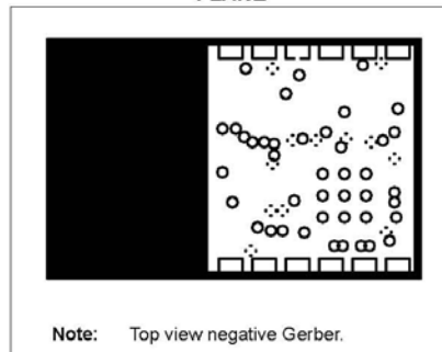
FIGURE 2-6: BOTTOM COPPER
