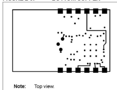
FIGURE 2-6: BOTTOM COPPER
