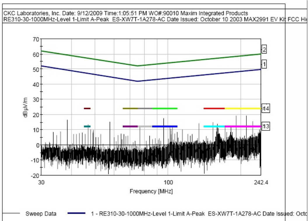
Figure 11. Radiated emissions test results for the Maxim 2990/2991 device.
