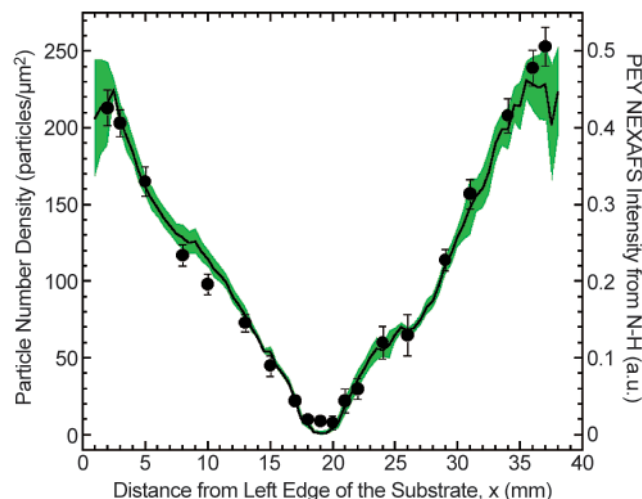
Figure 3: Particle number density (left axis) and NEXAFS PEY (right axis) profile for a “double gradient” prepared by evaporating APTES/PO mixture for 3 min from both ends of the substrate followed by immersion in colloidal gold solution for 24 h. The data points represent an average from 3 transverse scans along the gradient taken at the center of the sample ( y = 0 mm, y = -3 mm, and y = +3 mm). The area around the PEY NEXAFS line denotes the measurement uncertainty (based on 7 line scans along the gradient taken between -3 mm and +3 mm from the center of the sample).
