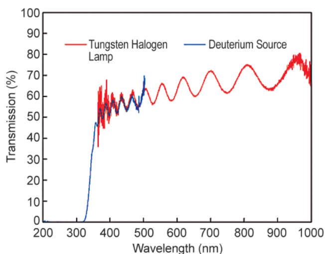
Figure 1: Test of the UV-Visible Transmission Spectrometer on a single-composition BaTiO 3 -SrTiO 3 film.
