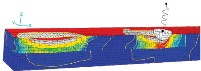
Figure 3: Contour plot of the maximum principle stress field created from two collisions between an asperity (represented by a semi sphere in the figure) and substrate.
