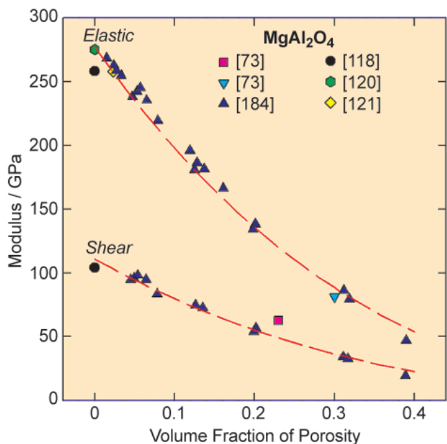
Figure 1: The elastic and shear moduli of MgAl_2O_4 at 23^\circ C decrease rapidly as the volume fraction of porosity increases. [Numbers in brackets are references in NISTIR 6853.]
