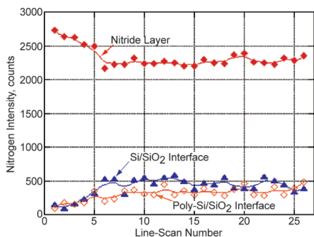
Figure 3: Integrated nitrogen intensity as a function of line-scan number in the EELS spectrum-image acquired in the dedicated STEM. The nitrogen signal at both Si/SiO 2 and poly-Si/SiO 2 interfaces increases significantly with increasing scan number. A corresponding decrease in the nitrogen signal from the nitride layer is consistent with the beam-induced nitrogen diffusion/segregation.
