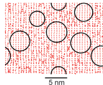
Figure 1: Local electric fields in a model for the relaxor ferroelectric PSN. Experiments suggest that relaxor ferroelectrics contain chemically-ordered regions in a disordered matrix and that such inhomogeneities may be responsible for the relaxor behavior. Computations show that chemically-ordered regions in PSN (circles) have much lower local fields than the disordered matrix.
