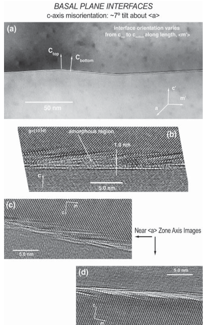
Figure 1: Bacrystal grain boundary produced by growth roughly normal to the c -plane. The crystals are misoriented by 7^\circ about the \langle a \rangle axis. Boundaries all contain Ca and Si, but some, (c) and (d), are so narrow that it is difficult to see if these elements in the form of a glass. The faceted structure of the boundary in (a) is typical of the wetted Wulff shape of crystals with these orientations.
