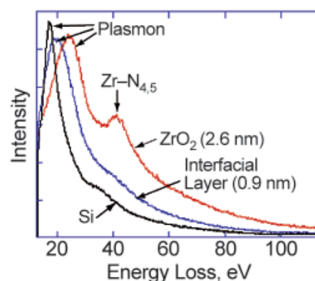
Figure 4: Upper: HRTEM image of a ZrO 2 film deposited on HF-treated silicon at 460°C. Lower: Spatially-resolved EELS spectra from the same area.
