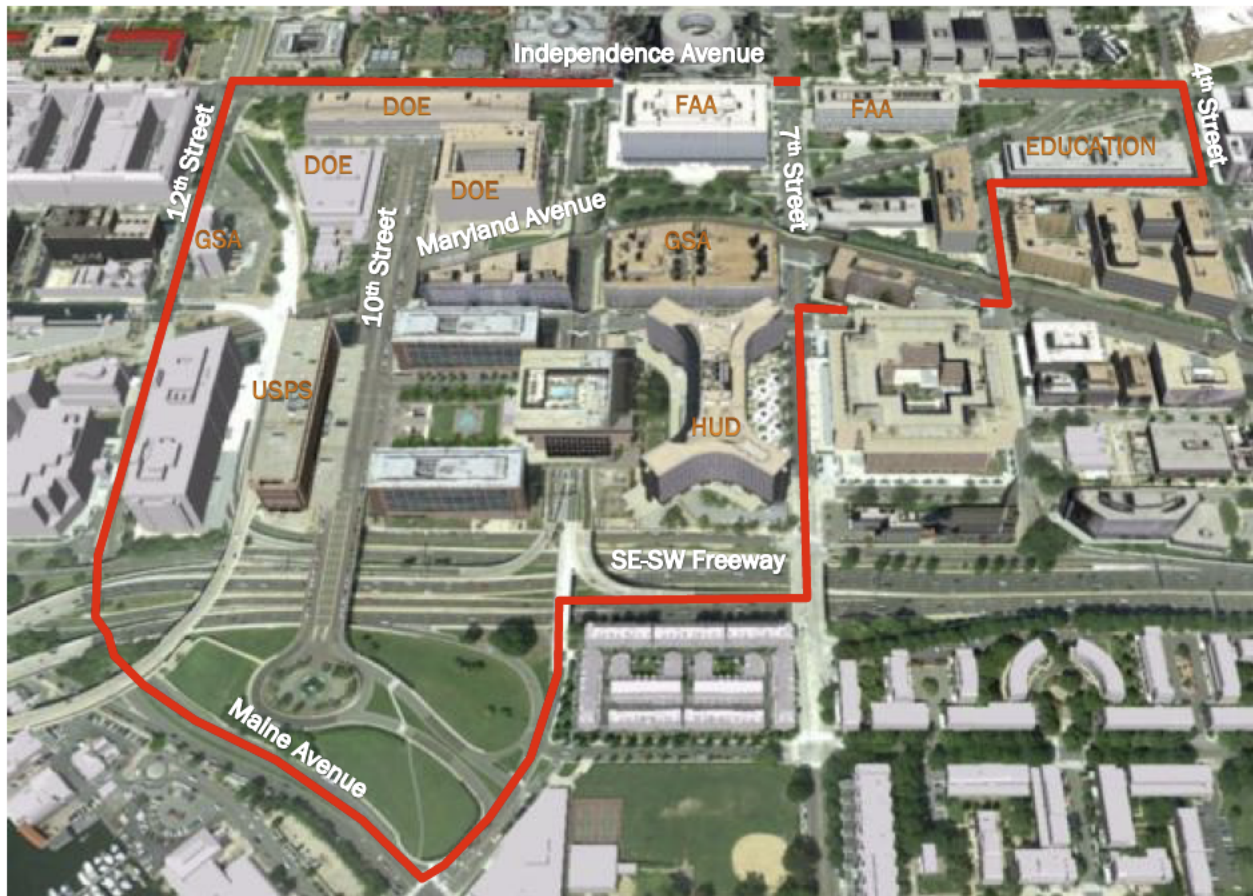
Figure 1: SW Ecodistrict Study Area.
