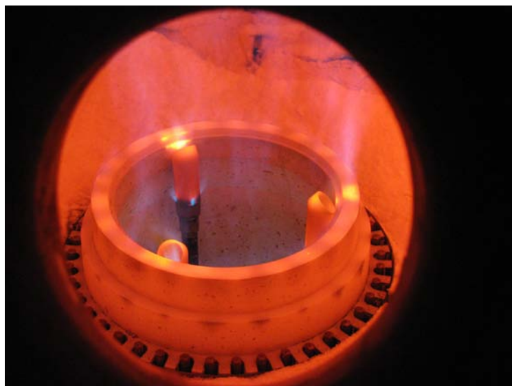
Figure 1. The commercial Zeeco Free-Jet Burner served as a base design for concept and prototype development.
