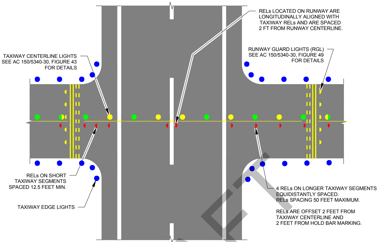
Figure 144. REL Configuration for Taxiways at 90 Degrees
