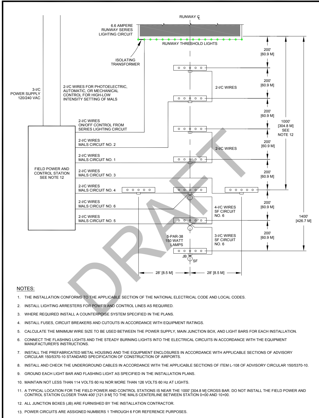
Figure 85. Typical Field Wiring Circuits for MALSF.
