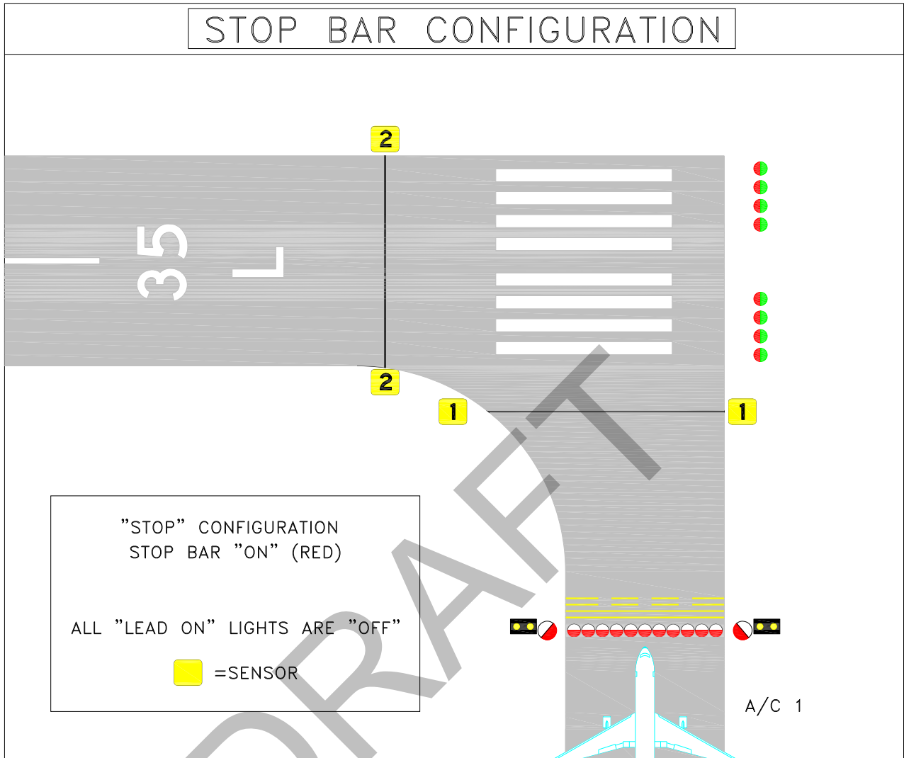
Figure 59. Controlled Stop Bar Design and Operation – “STOP” Configuration.
