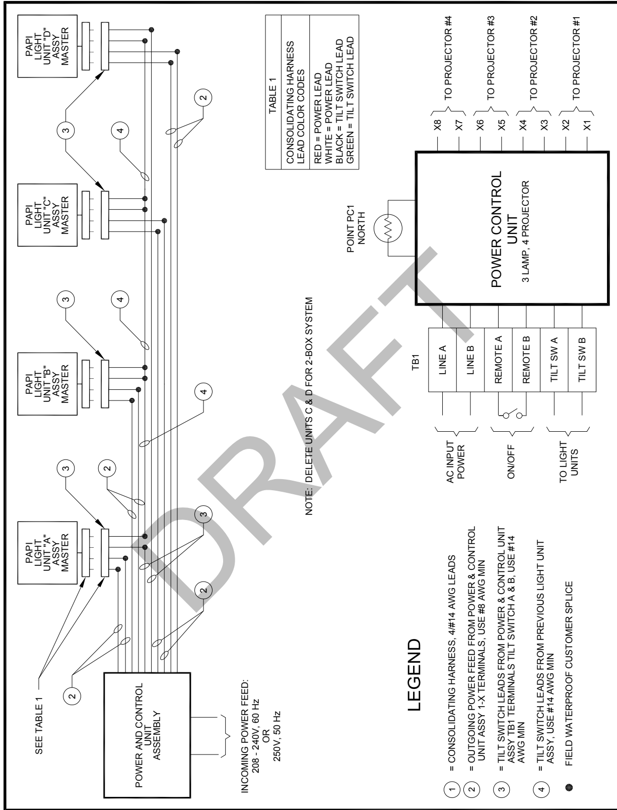
Figure 90. FAA L-880 Style A (Constant Voltage) System Wiring Diagram.
