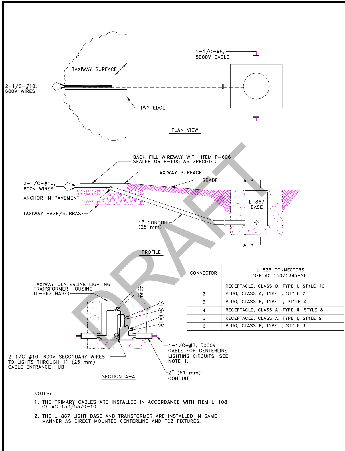
Figure 107. Typical Transformer Housing and Conduit Installation Details for Taxiway Centerline Lights.
