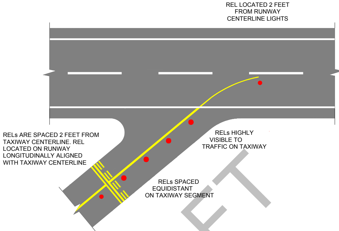
Figure 145. Angled Configuration
