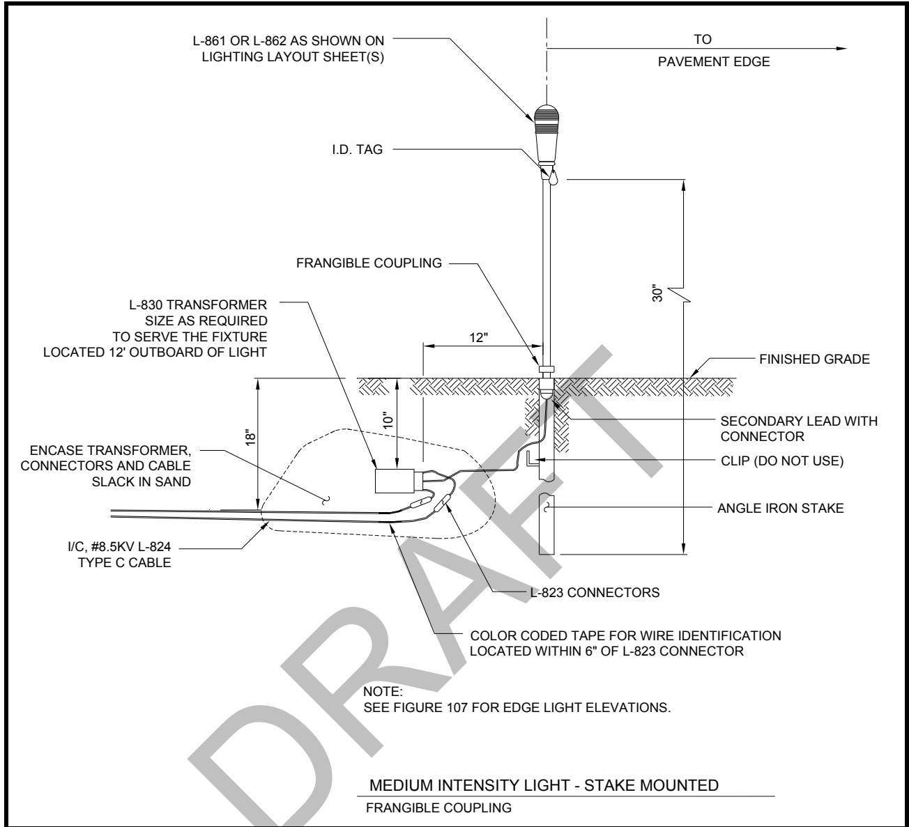
Figure 116. Typical Standard Details for Runway & Taxiway Edge Lights –Medium Intensity Light – Stake-mounted.
