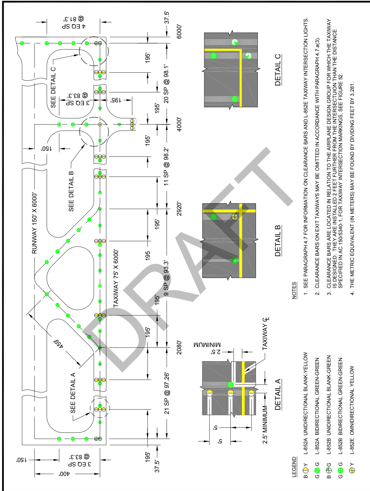
Figure 43. Typical Taxiway Centerline Lighting Configuration for Non-Standard Fillets (Centerline light spacing for operations above 1,200 ft. (365 m) RVR).
