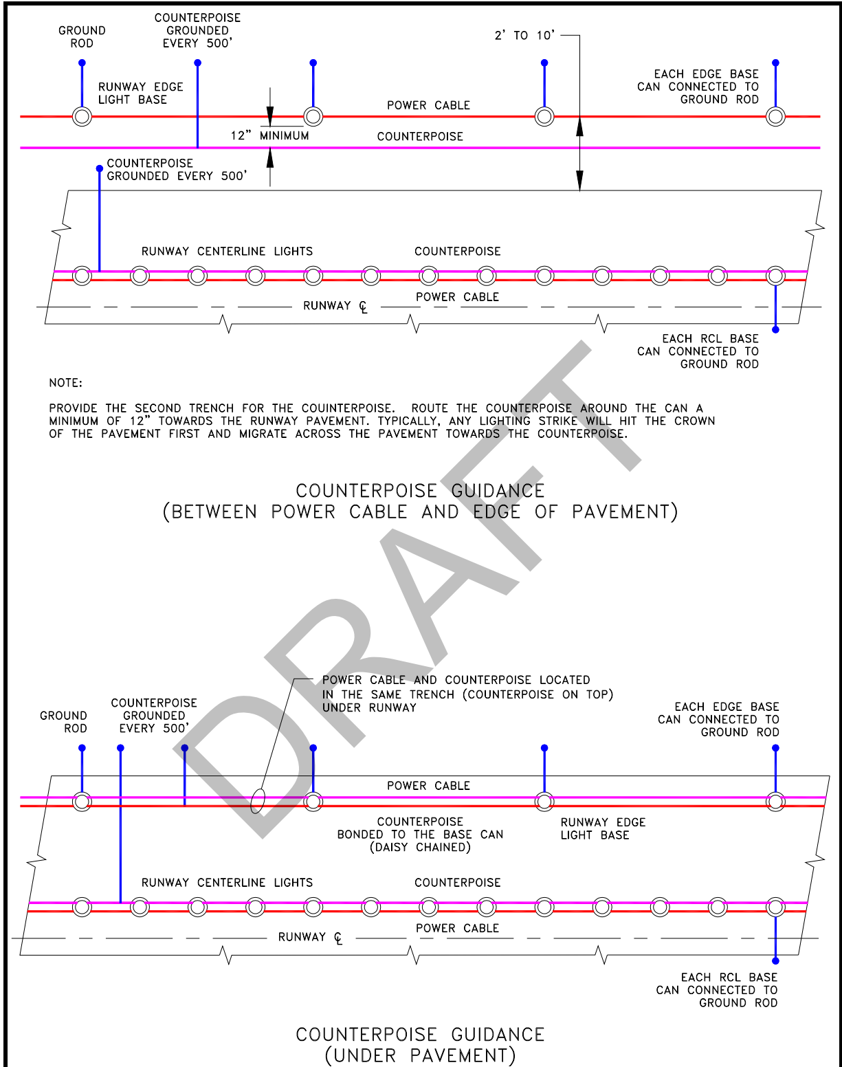
Figure 117. Typical Counterpoise and Ground Rod Connections
