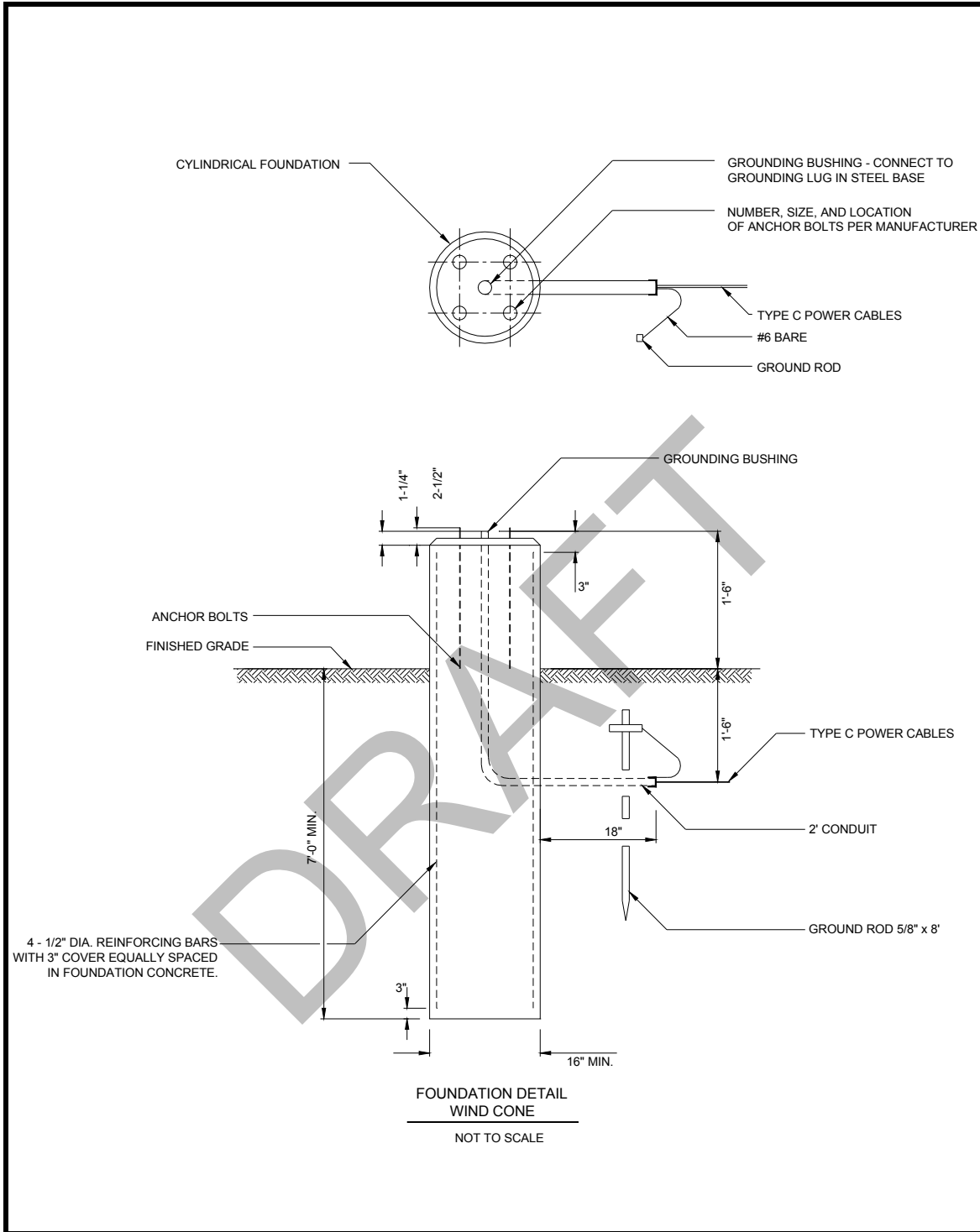
Figure 132. Standard Details for Wind Cone Foundation (L-807).
