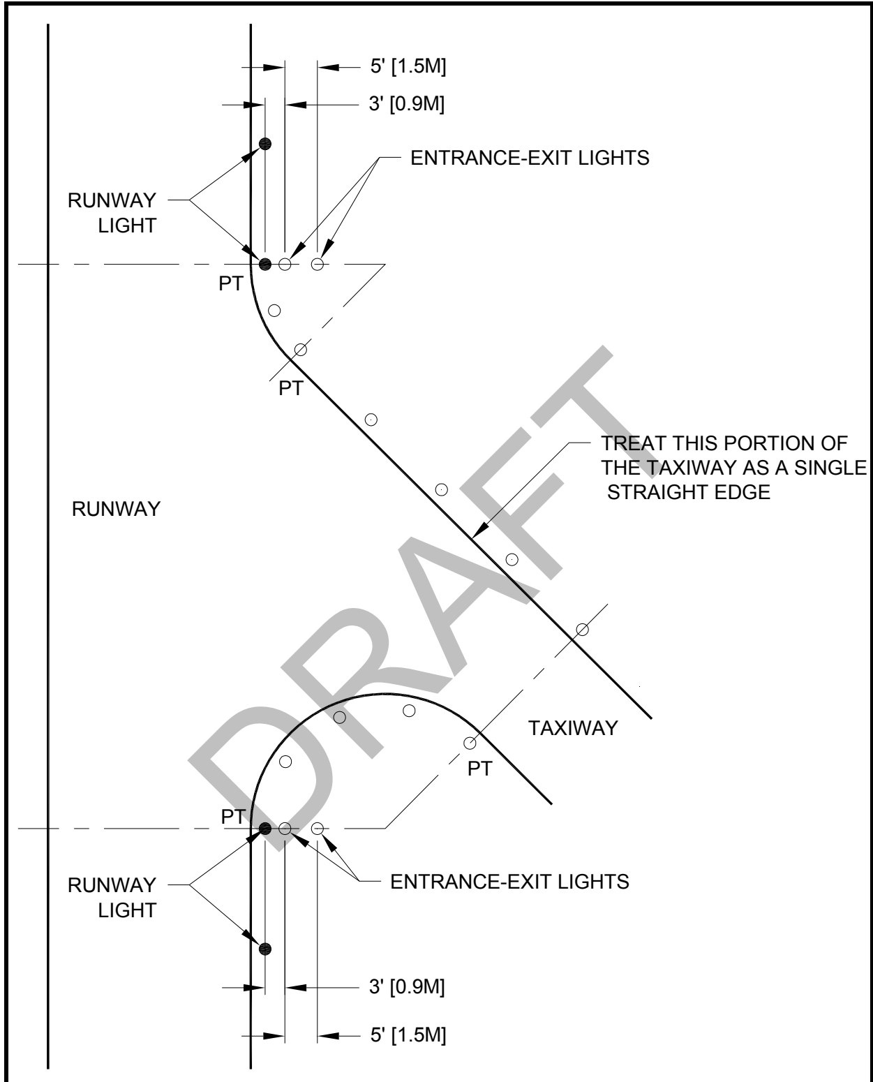
Figure 139. Location of Entrance-Exit Lights (in lieu of guidance signs).
