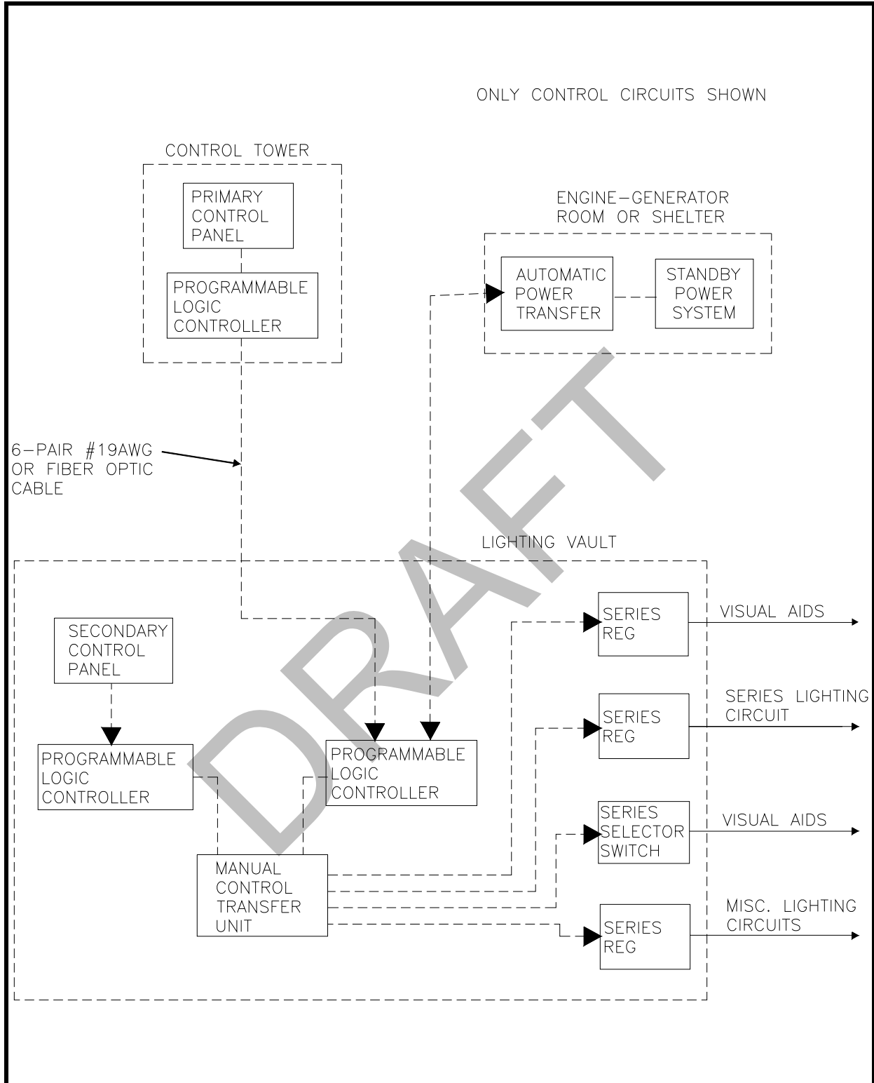
Figure 112. Typical PLC Control System Block Diagram.
