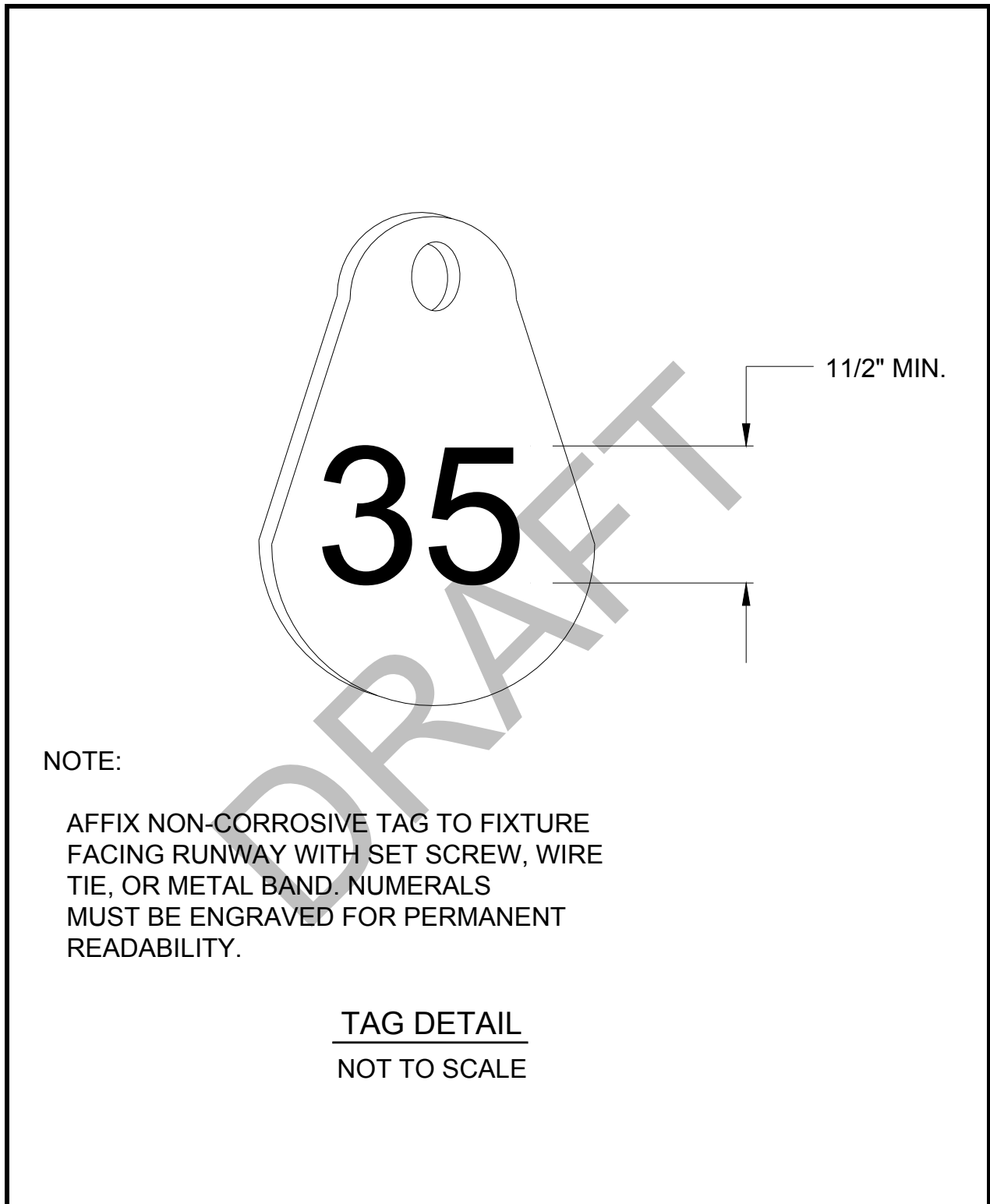
Figure 118. Identification (ID) Tag Detail.
