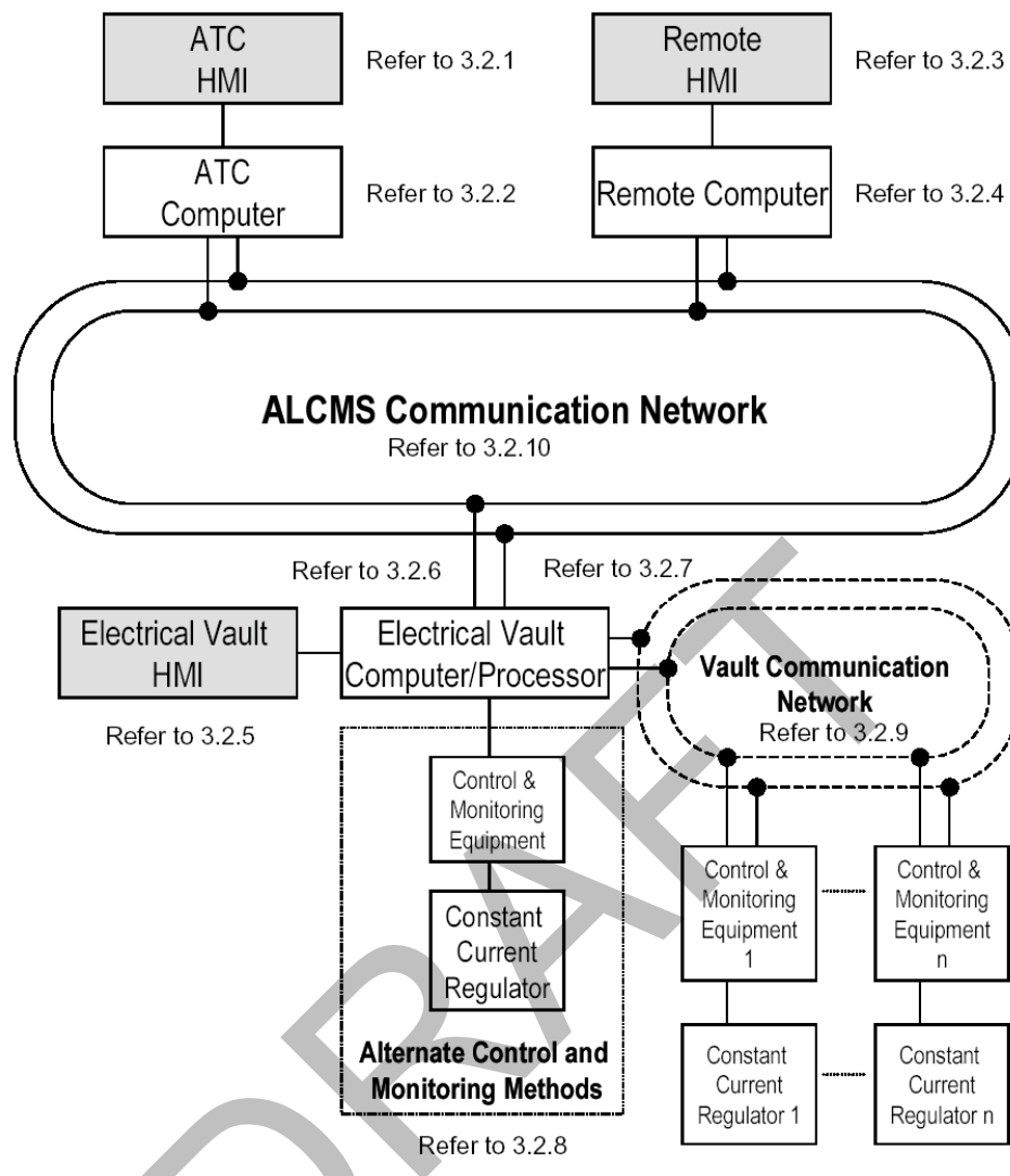
Figure 143. ALCMS Block Diagram
