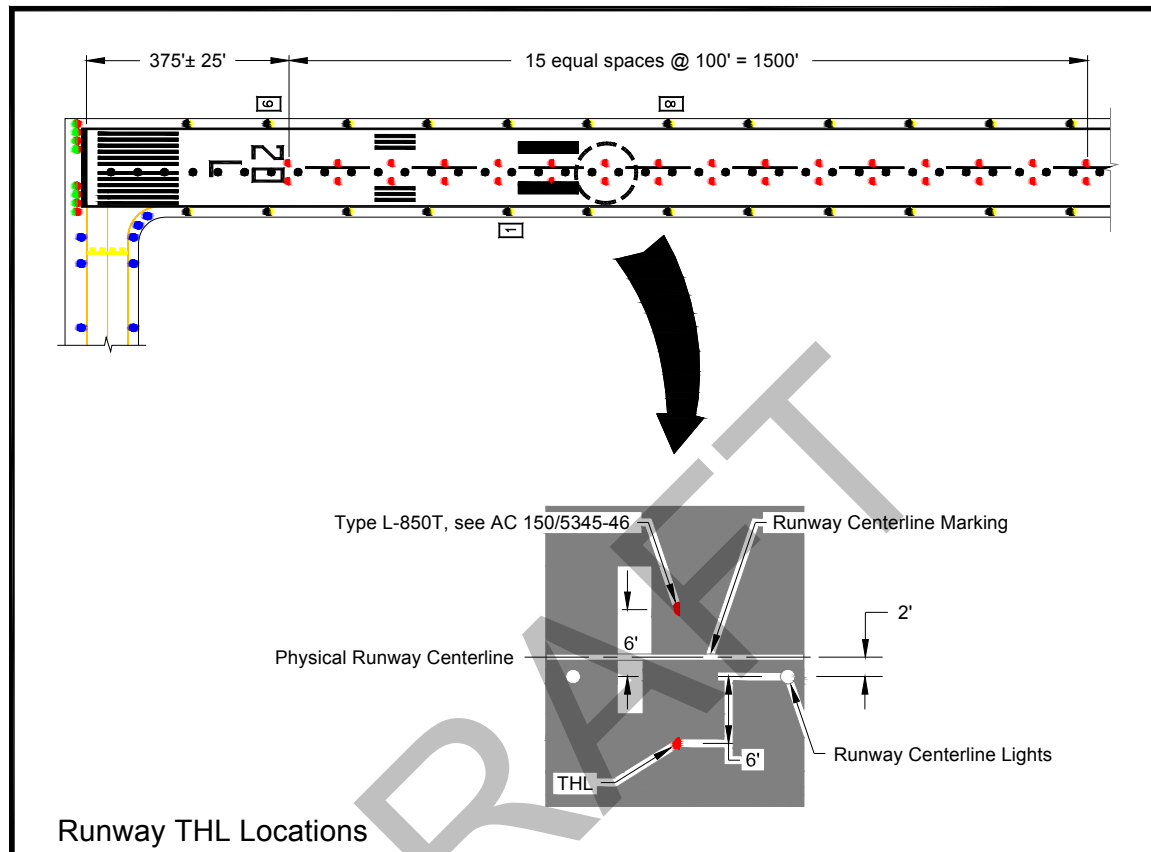
Figure 146. Takeoff/Hold Lights
