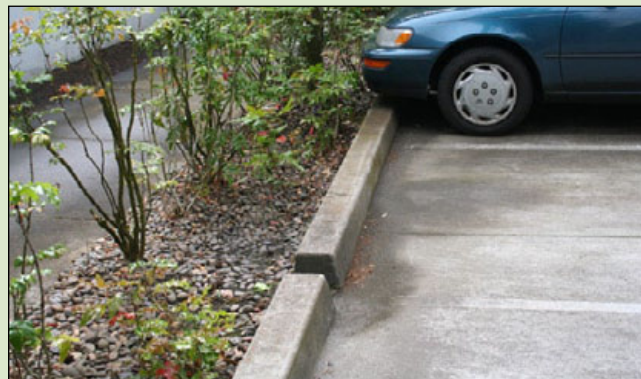
Figure C-16. Curb cut that is too small for the amount of runoff entering it.
