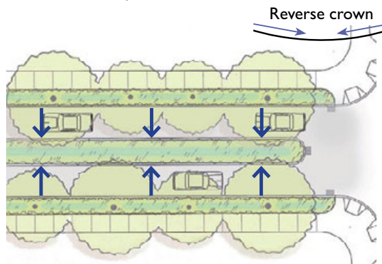
Figure C-19. Reverse crowned street.
