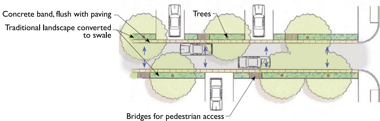
Figure 79. Side swales—plan view.
