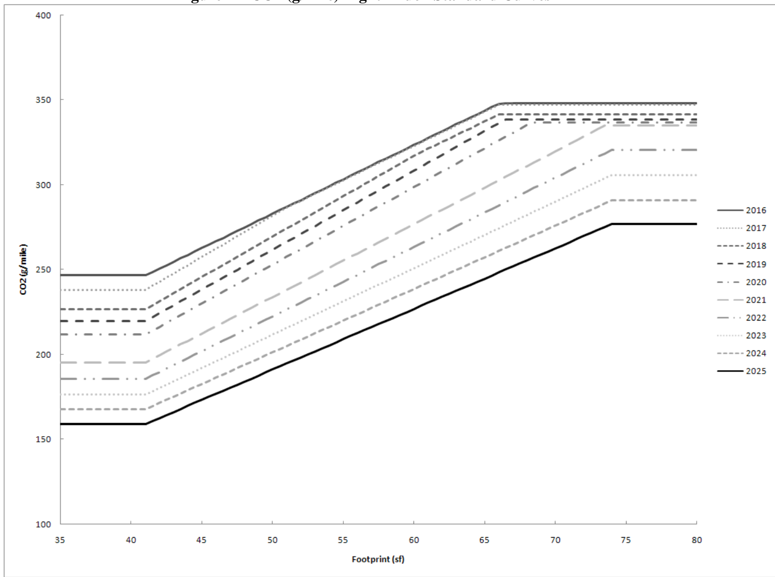
Figure I-4 CO 2 (g/mile) Light-Truck Standard Curves
