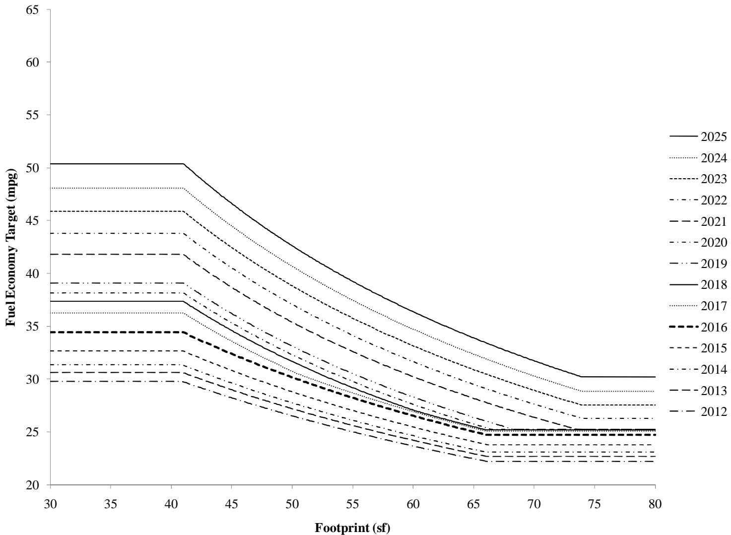
Figure IV-3 NHTSA Fuel Economy Targets for MYs 2012–2016 and 2017–2025 Light Trucks
