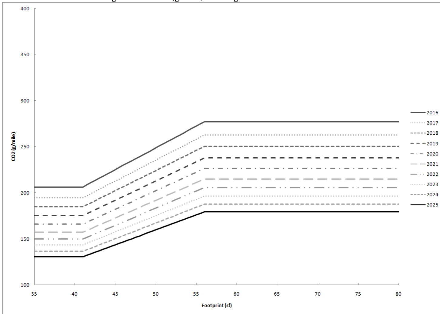
Figure I- 3 CO2 (g/mile) Passenger Car Standards Curves
