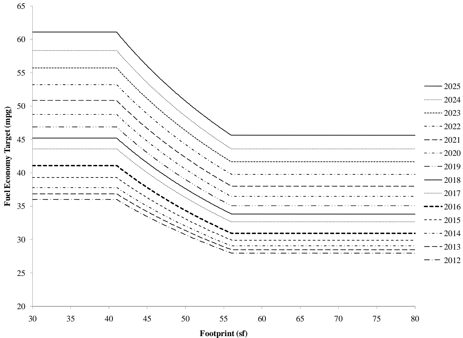
Figure IV-2 NHTSA Fuel Economy Targets for MYs 2012–2016 and 2017–2025 Passenger Cars
