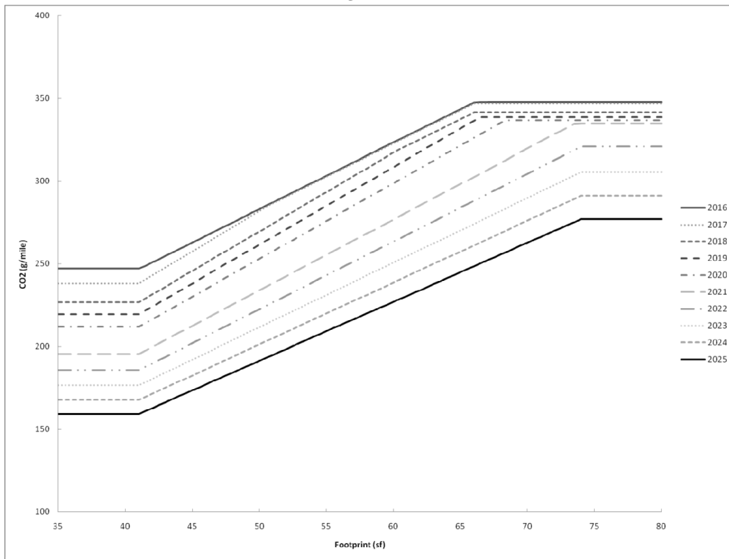
Figure III-2 –Truck Curves
