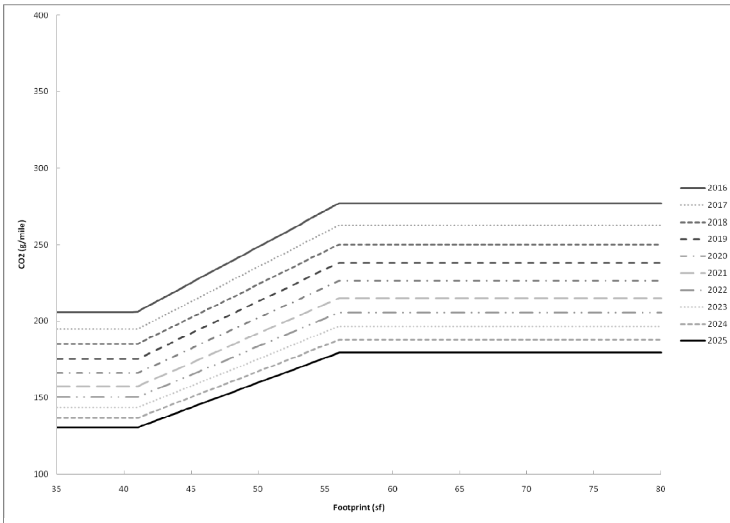
Figure III-1 Car Curves
