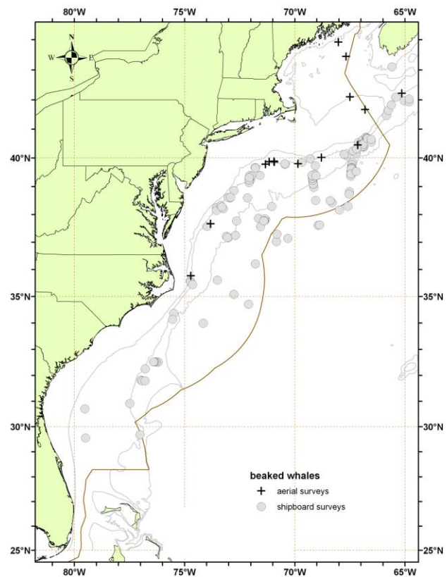
Figure 1: NEFSC and SEFSC shipboard and aerial surveys during the summers of 1998, 1999, 2002, 2004 and 2006. Isotherms are the 100-m, 1000-m and 4000-m depth contours.
