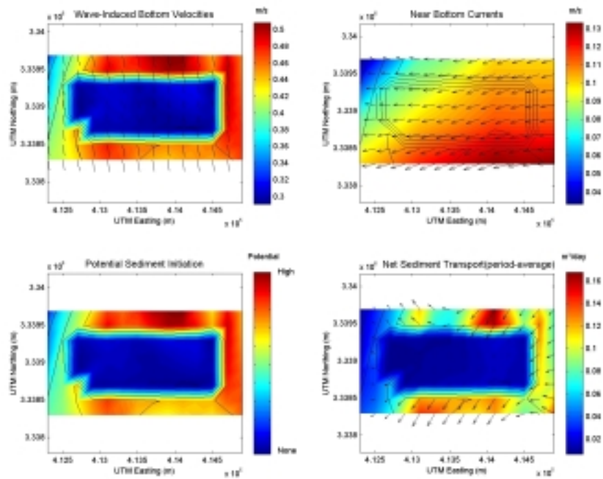
Figure C1-17. Fall hydrodynamic and sediment transport results at Sand Resource Area 3. The solid black lines represent depth contours, and sediment transport results are based on 200 m cell widths.
