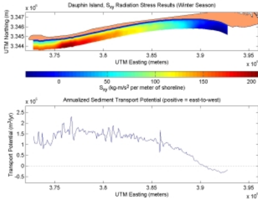
Figure C2-1. S_{xy} radiation stress and annualized sediment transport potential for existing conditions at Dauphin Island during the winter season.
