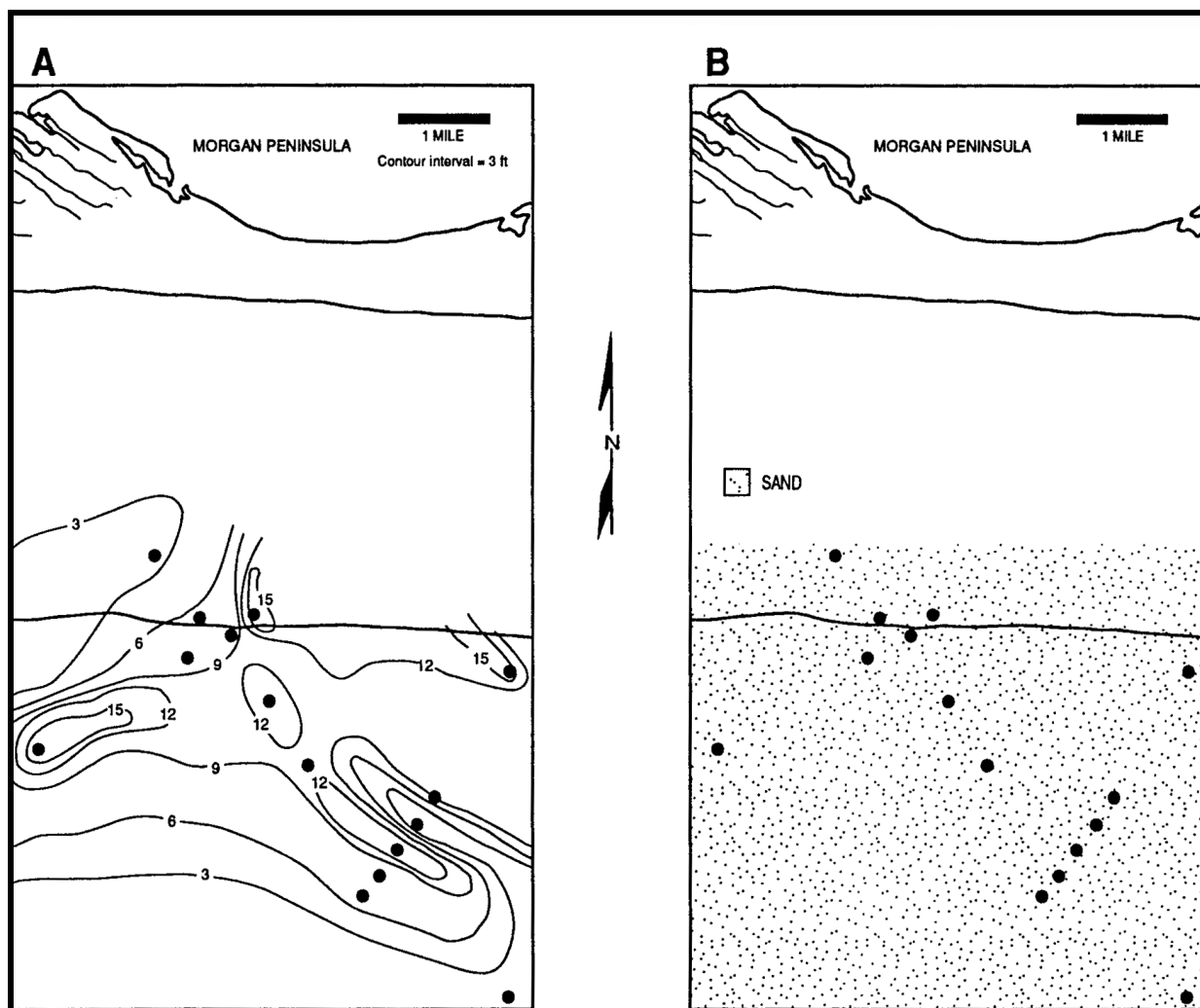
Figure 2-16. Sand isopach (A) and surface sediment texture (B) maps for Sand Resource Area 3 (from Parker et al., 1997).
