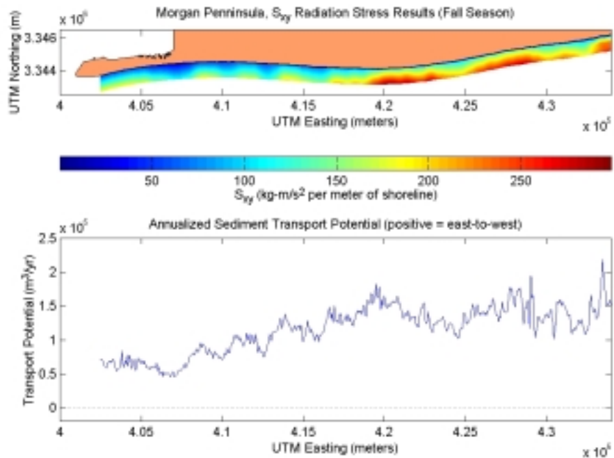
Figure C2-18. S_{xy} radiation stress and annualized sediment transport potential for post-dredging scenario at Morgan Peninsula during the fall season.
