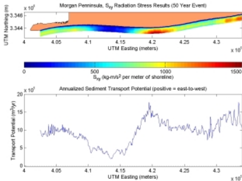
Figure C2-10. S_{xy} radiation stress and annualized sediment transport potential for existing conditions at Morgan Peninsula during a 50-year storm.
