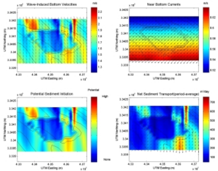
Figure C1-6. Storm hydrodynamic and sediment transport results at Sand Resource Area 1. The solid black lines represent depth contours, and sediment transport results are based on 200 m cell widths.
