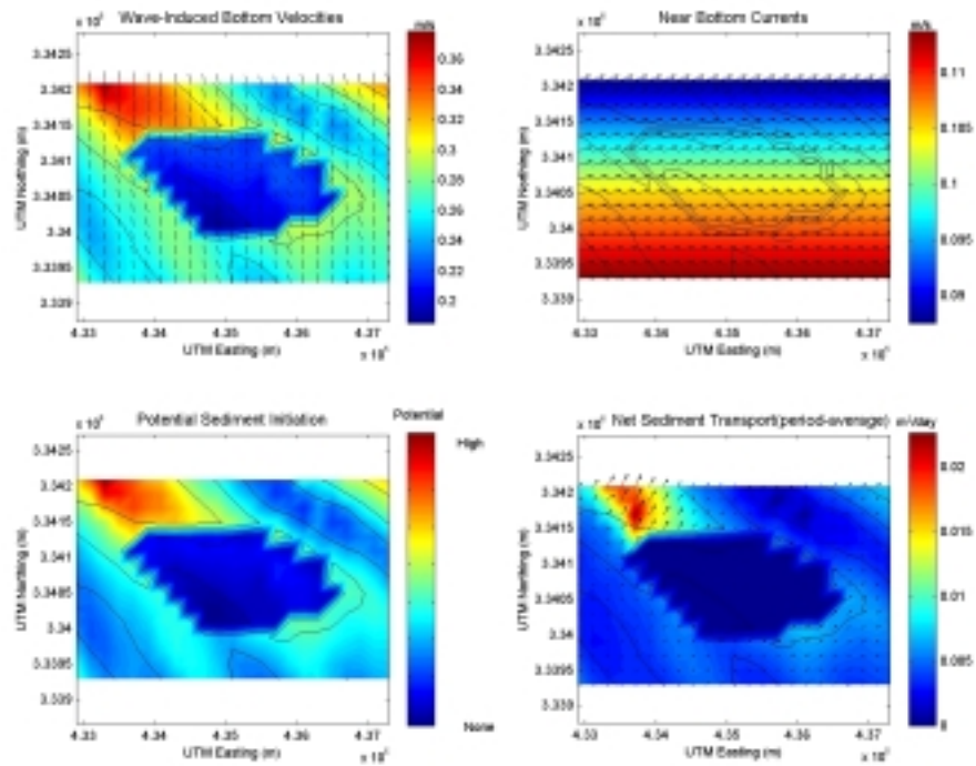
Figure C1-4. Summer hydrodynamic and sediment transport results at Sand Resource Area 1. The solid black lines represent depth contours, and sediment transport results are based on 200 m cell widths.
