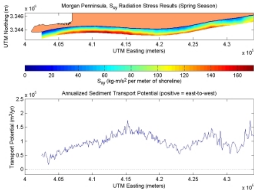
Figure C2-14. S_{xy} radiation stress and annualized sediment transport potential for post-dredging scenario at Morgan Peninsula during the spring season.
