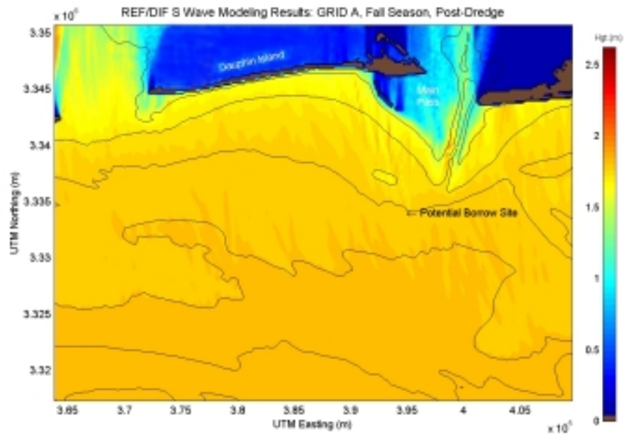
Figure B3-7. Spectral wave modeling results for post-dredged conditions utilizing a typical fall season at reference Grid A.
