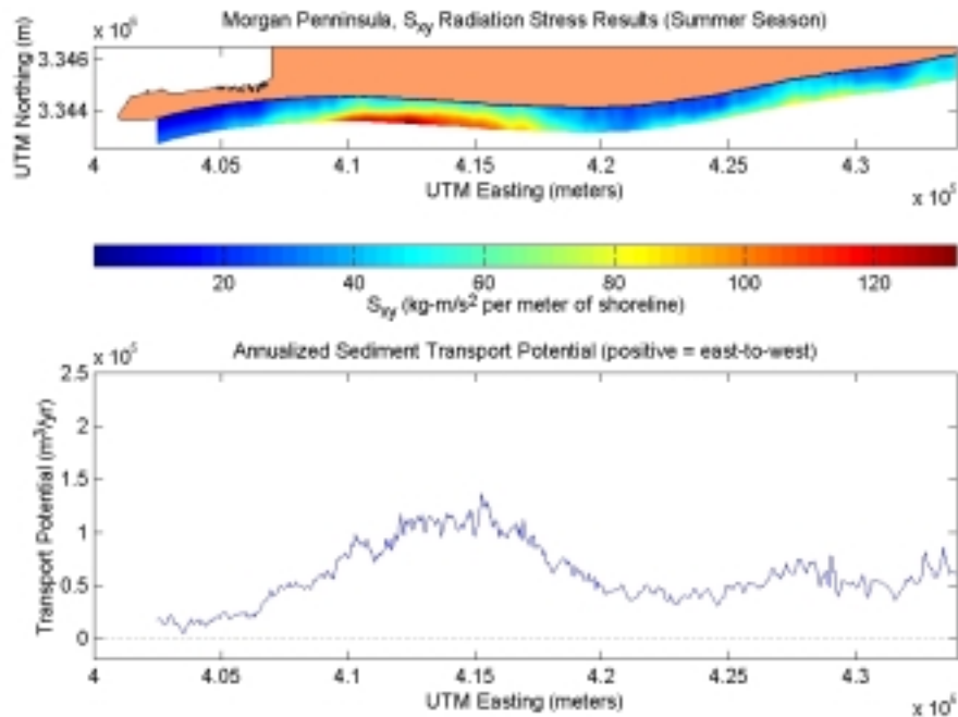
Figure C2-6. S_{xy} radiation stress and annualized sediment transport potential for existing conditions at Morgan Peninsula during the summer season.
