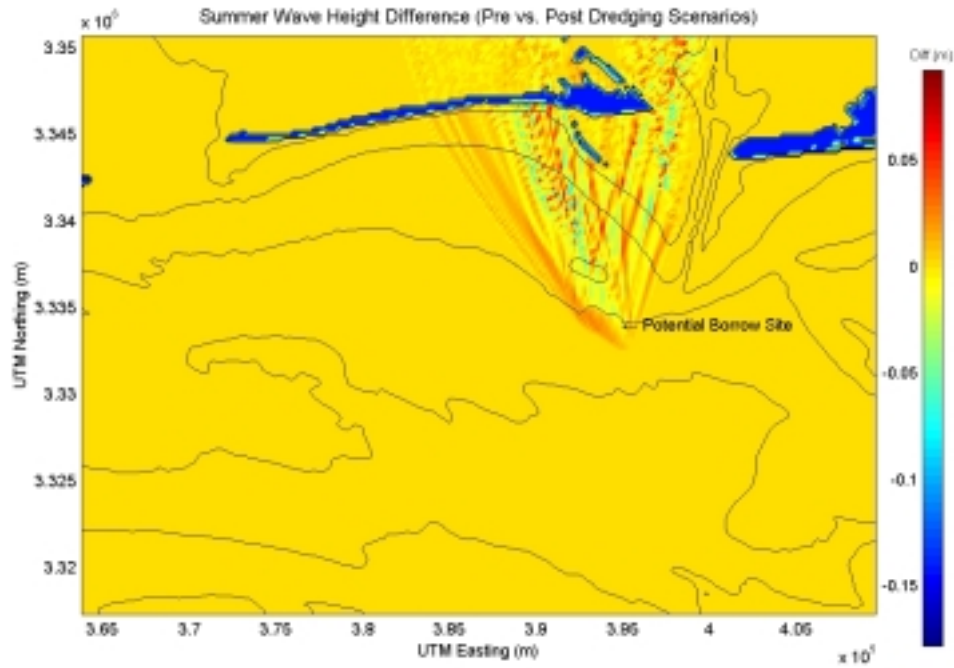
Figure B4-5. Wave height modifications caused by the offshore sand mining at Resource Area 4 for a typical summer season.
