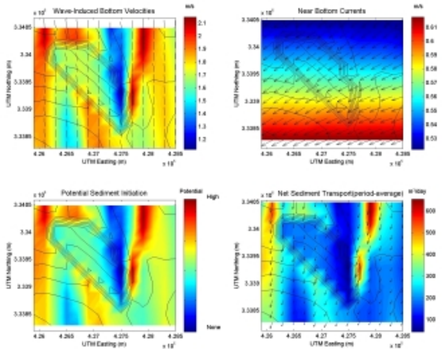
Figure C1-12. Storm hydrodynamic and sediment transport results at Sand Resource Area 2. The solid black lines represent depth contours, and sediment transport results are based on 200 m cell widths.
