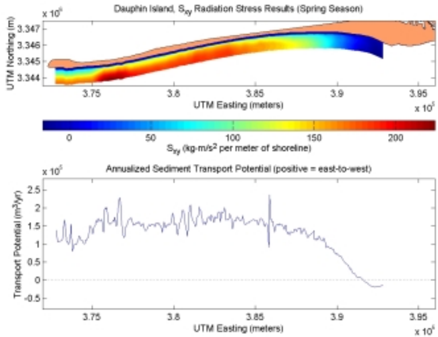
Figure C2-3. S_{xy} radiation stress and annualized sediment transport potential for existing conditions at Dauphin Island during the spring season.
