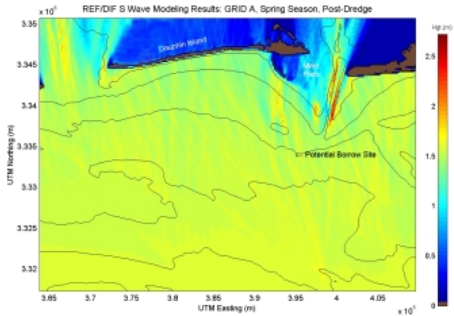
Figure B3-3. Spectral wave modeling results for post-dredged conditions utilizing a typical spring season at reference Grid A.
