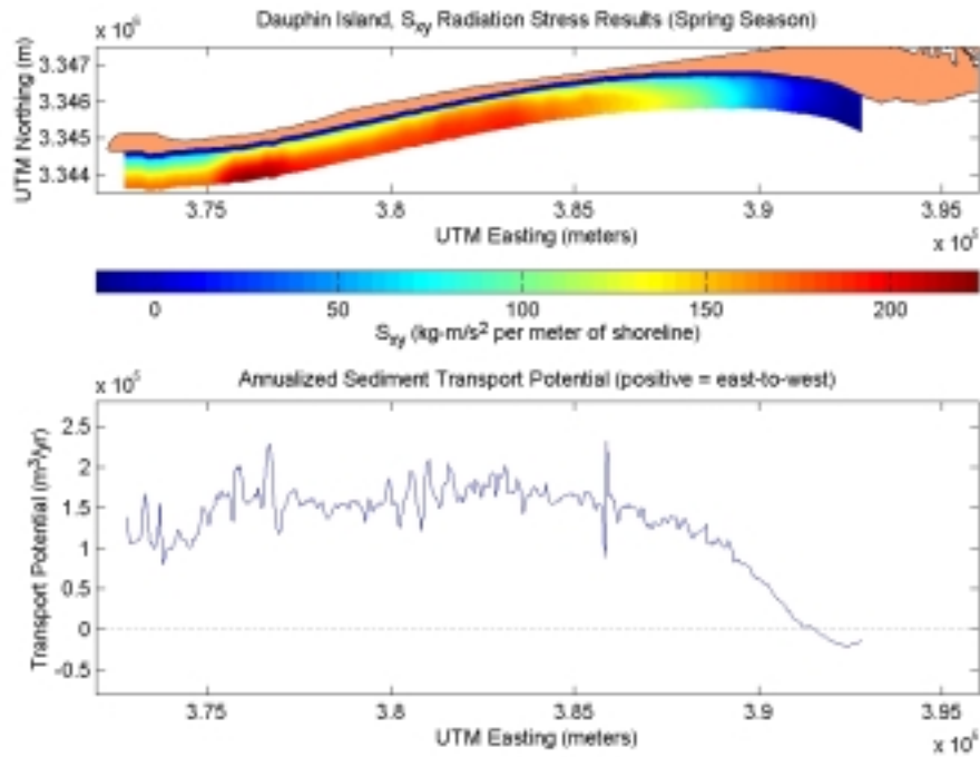
Figure C2-13. S_{xy} radiation stress and annualized sediment transport potential for post-dredging scenario at Dauphin Island during the spring season.
