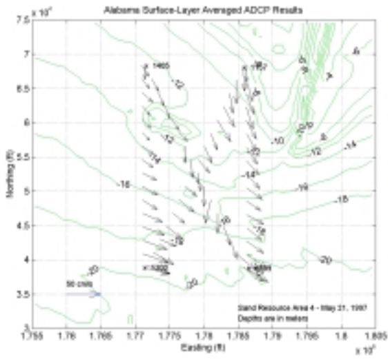
Surface Layer
