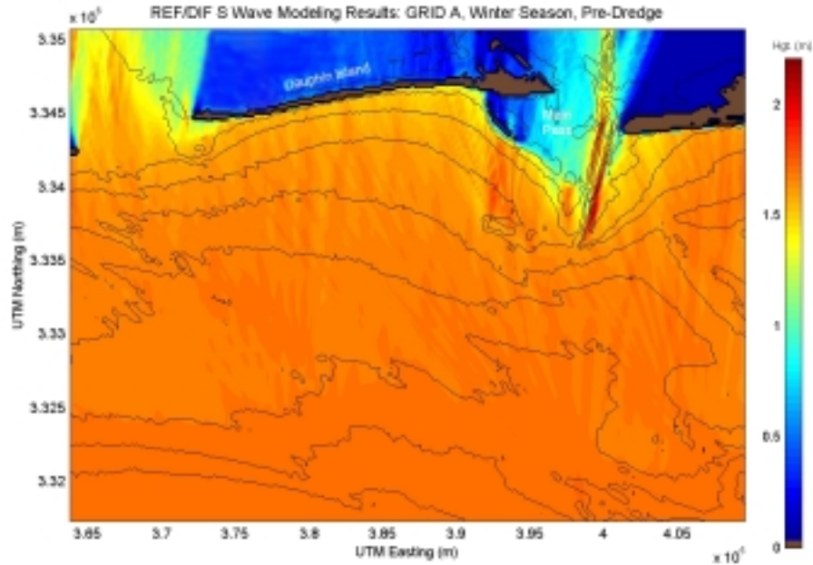
Figure B2-1. Spectral wave modeling results for existing conditions utilizing a typical winter season at reference Grid A.
