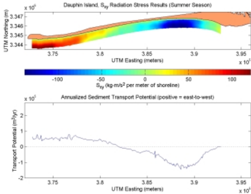
Figure C2-15. S_{xy} radiation stress and annualized sediment transport potential for post-dredging scenario at Dauphin Island during the summer season.
