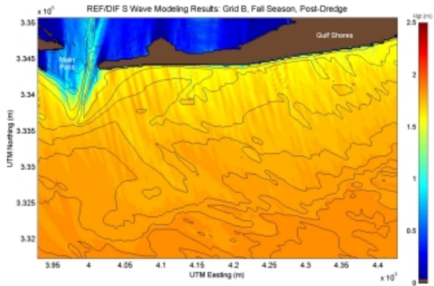
Figure B3-8. Spectral wave modeling results for post-dredged conditions utilizing a typical fall season at reference Grid B.
