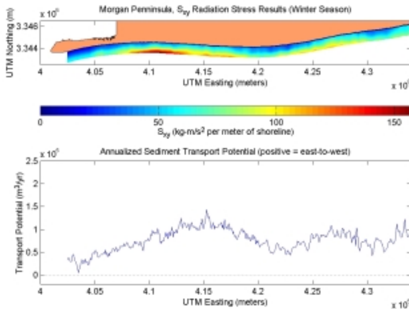
Figure C2-2. S_{xy} radiation stress and annualized sediment transport potential for existing conditions at Morgan Peninsula during the winter season.
