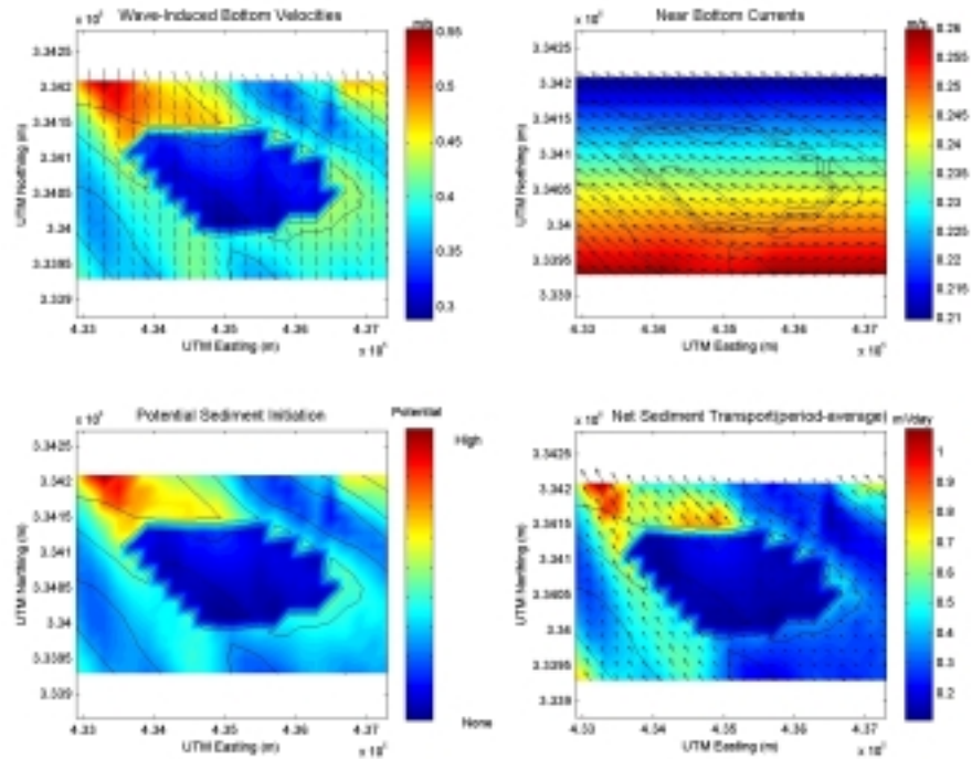
Figure C1-2. West winter hydrodynamic and sediment transport results at Sand Resource Area 1. The solid black lines represent depth contours, and sediment transport results are based on 200 m cell widths.
