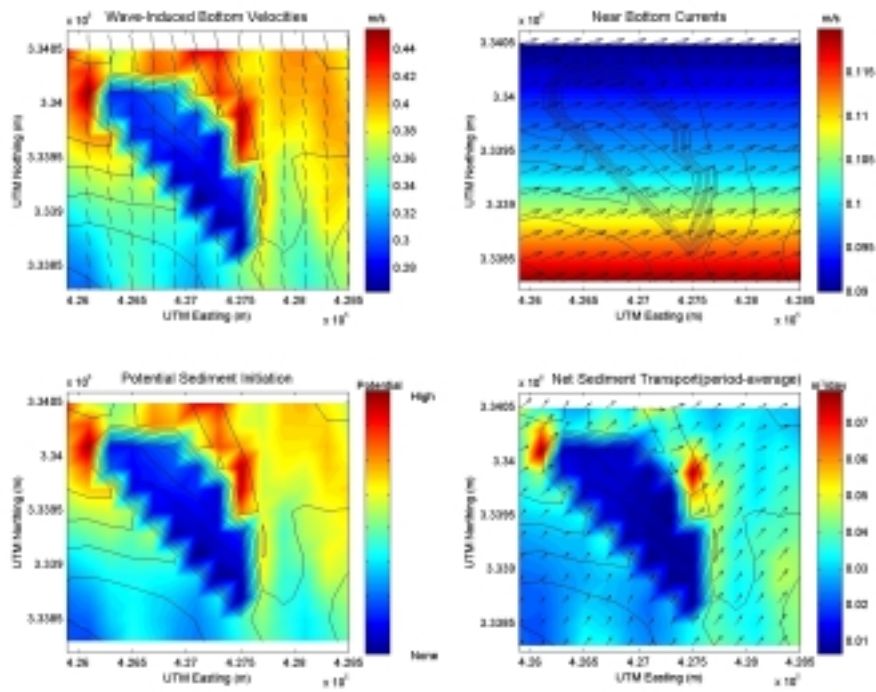
Figure C1-7. Northeast winter hydrodynamic and sediment transport results at Sand Resource Area 2. The solid black lines represent depth contours, and sediment transport results are based on 200 m cell widths.
