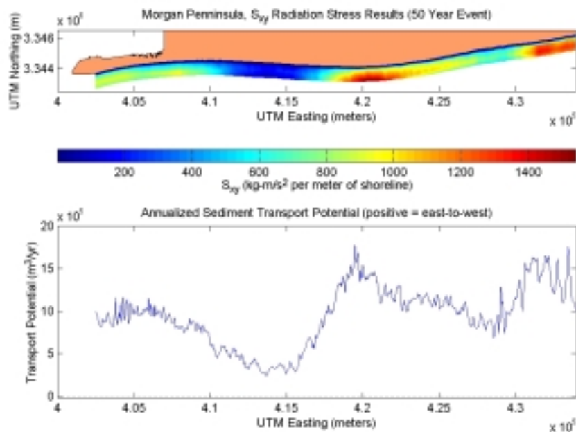
Figure C2-20. S_{xy} radiation stress and annualized sediment transport potential for post-dredging scenario at Morgan Peninsula during a 50-year storm.
