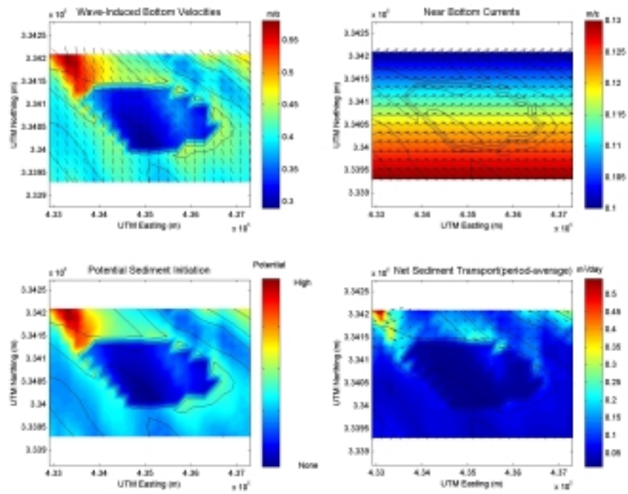
Figure C1-3. Spring hydrodynamic and sediment transport results at Sand Resource Area 1. The solid black lines represent depth contours, and sediment transport results are based on 200 m cell widths.
