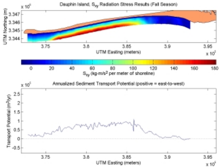
Figure C2-17. S_{xy} radiation stress and annualized sediment transport potential for post-dredging scenario at Dauphin Island during the fall season.
