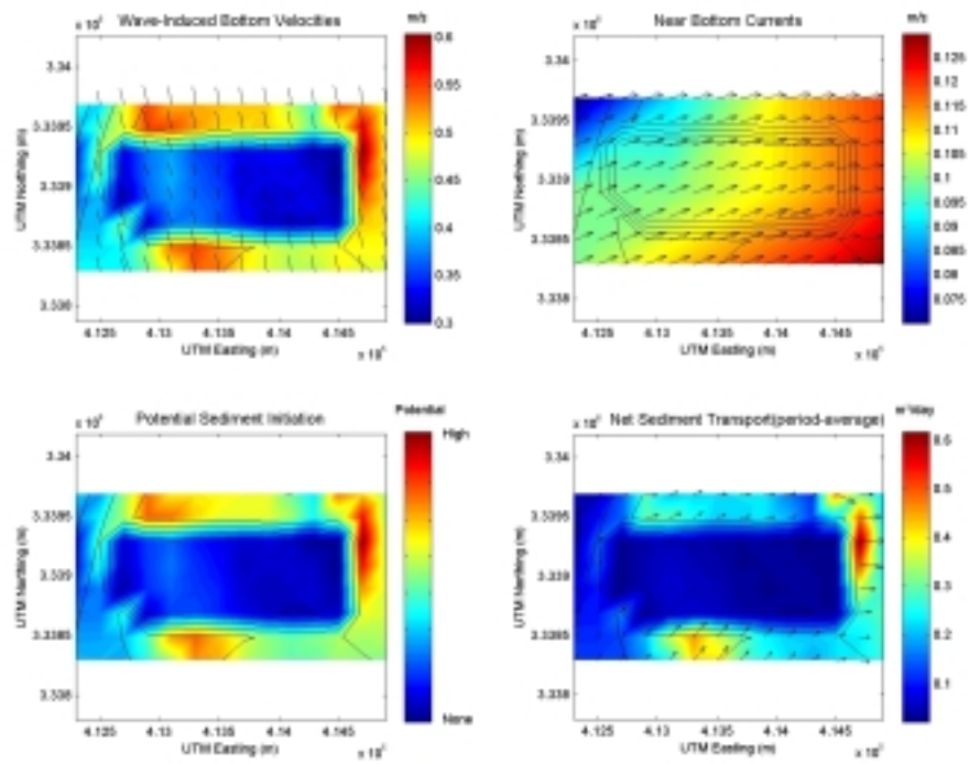
Figure C1-15. Spring hydrodynamic and sediment transport results at Sand Resource Area 3. The solid black lines represent depth contours, and sediment transport results are based on 200 m cell widths.
