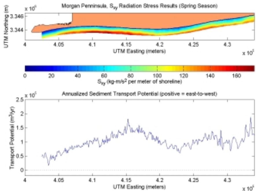
Figure C2-4. S_{xy} radiation stress and annualized sediment transport potential for existing conditions at Morgan Peninsula during the spring season.
