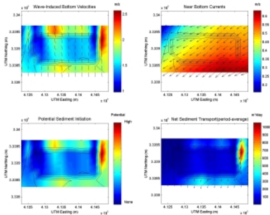
Figure C1-18. Storm hydrodynamic and sediment transport results at Sand Resource Area 3. The solid black lines represent depth contours, and sediment transport results are based on 200 m cell widths.
