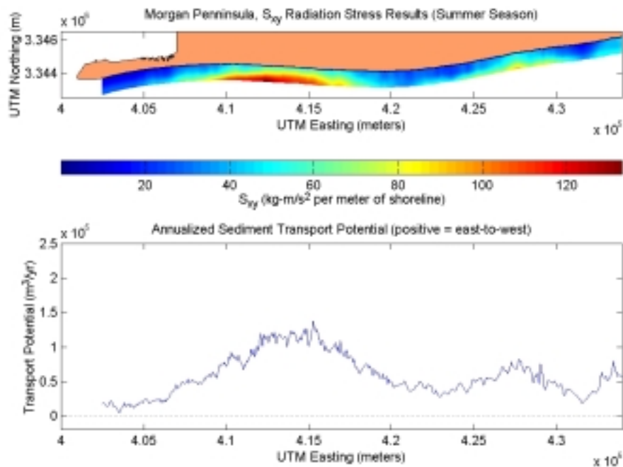
Figure C2-16. S_{xy} radiation stress and annualized sediment transport potential for post-dredging scenario at Morgan Peninsula during the summer season.
