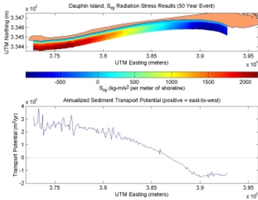
Figure C2-19. S_{xy} radiation stress and annualized sediment transport potential for post-dredging scenario at Dauphin Island during a 50-year storm.
