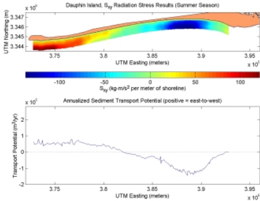
Figure C2-5. S_{xy} radiation stress and annualized sediment transport potential for existing conditions at Dauphin Island during the summer season.
