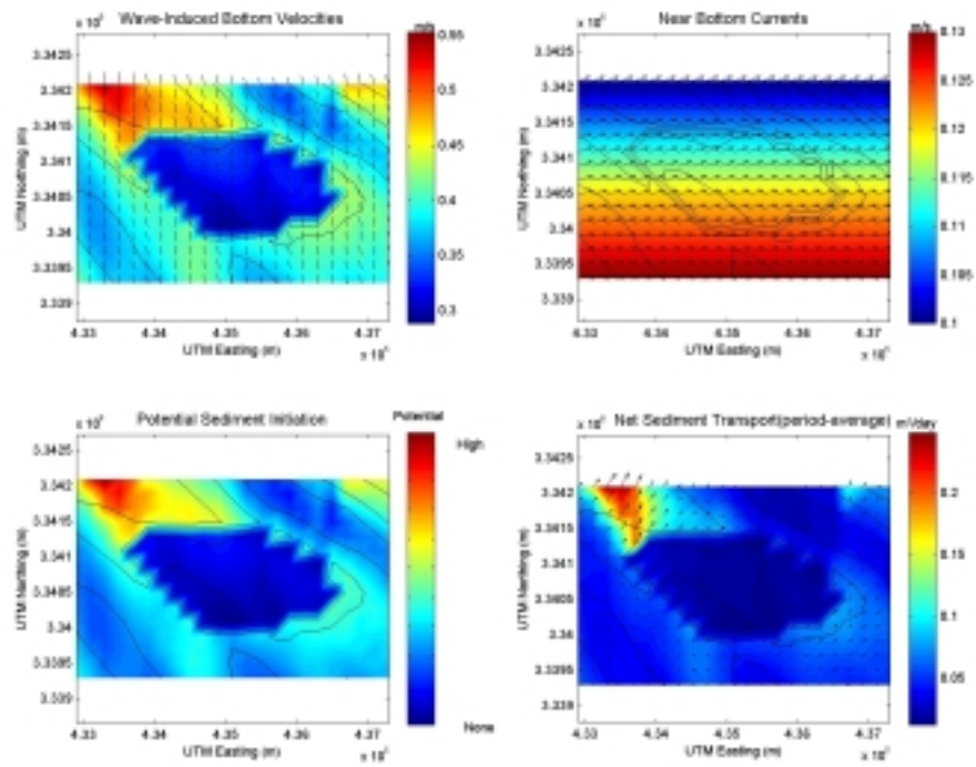
Figure C1-1. Northeast winter hydrodynamic and sediment transport results at Sand Resource Area 1. The solid black lines represent depth contours, and sediment transport results are based on 200 m cell widths.
