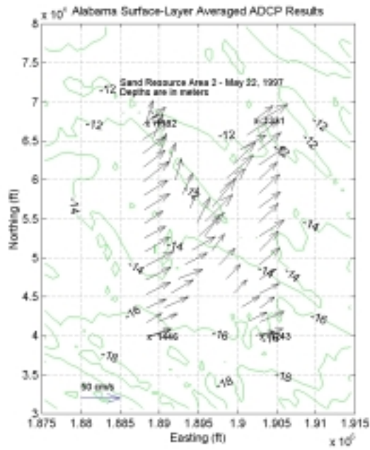
Surface Layer
