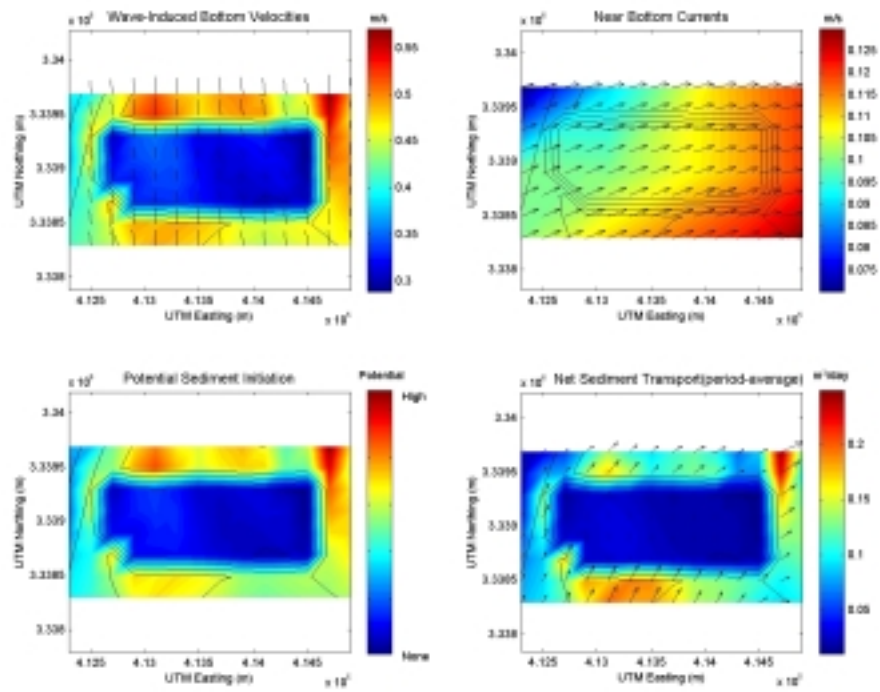
Figure C1-13. Northeast winter hydrodynamic and sediment transport results at Sand Resource Area 3. The solid black lines represent depth contours, and sediment transport results are based on 200 m cell widths.
