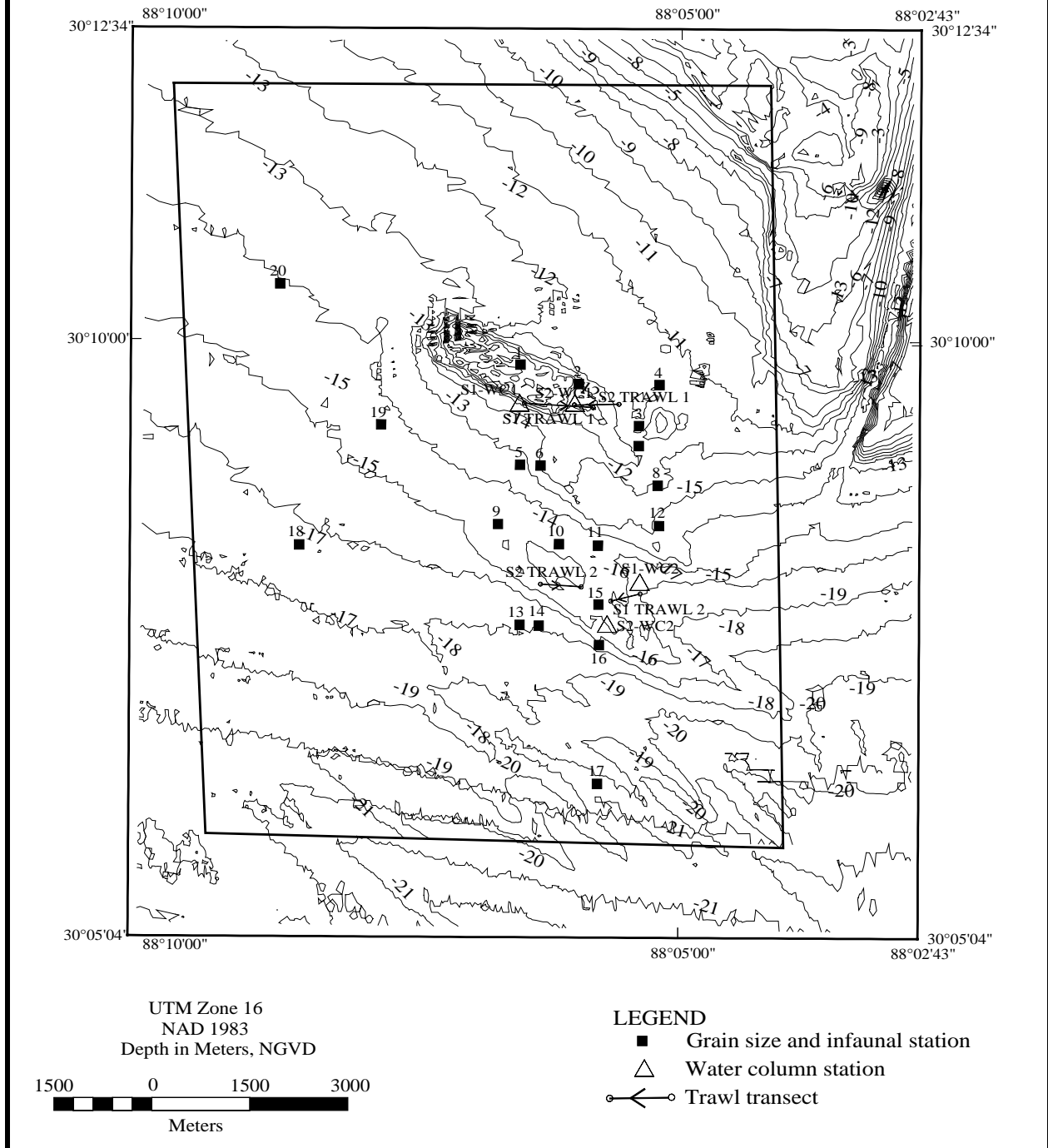
Figure 6-5. Sampling locations for Alabama Sand Resource Area 4. Inner box represents the limits of Area 4. Outer box provides reference coordinates.
