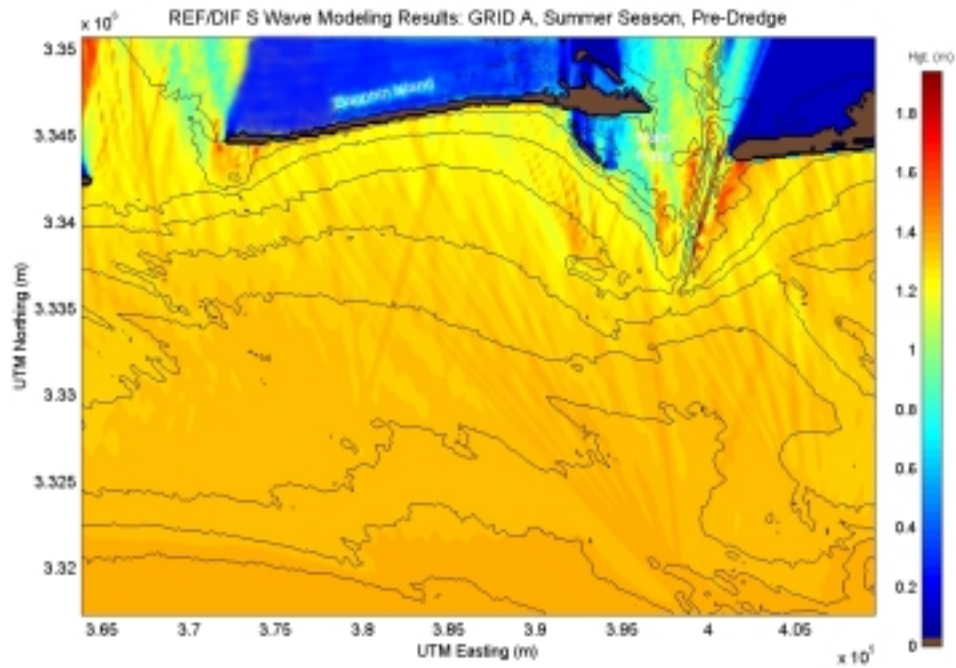
Figure B2-5. Spectral wave modeling results for existing conditions utilizing a typical summer season at reference Grid A.
