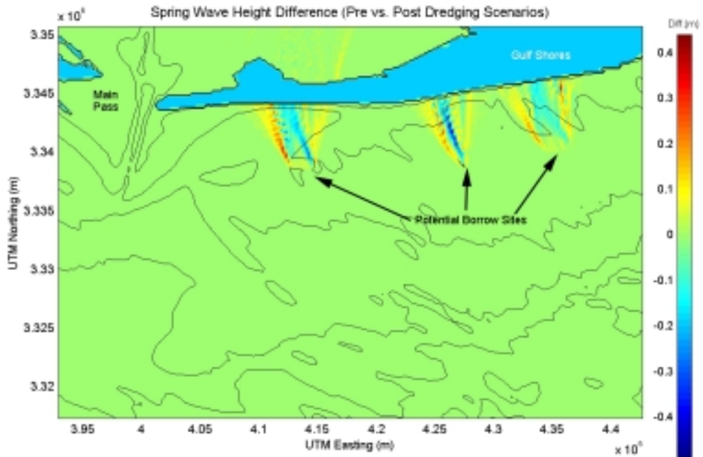
Figure B4-4. Wave height modifications caused by the offshore sand mining at Resource Areas 1, 2, and 3 for a typical spring season.
