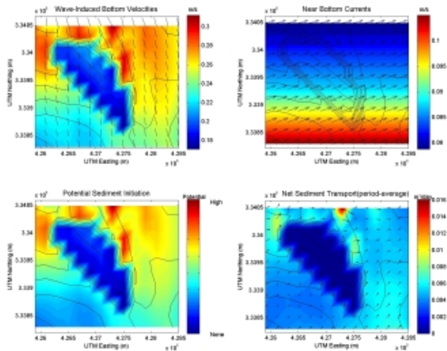
Figure C1-10. Summer hydrodynamic and sediment transport results at Sand Resource Area 2. The solid black lines represent depth contours, and sediment transport results are based on 200 m cell widths.
