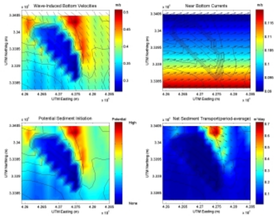
Figure C1-9. Spring hydrodynamic and sediment transport results at Sand Resource Area 2. The solid black lines represent depth contours, and sediment transport results are based on 200 m cell widths.
