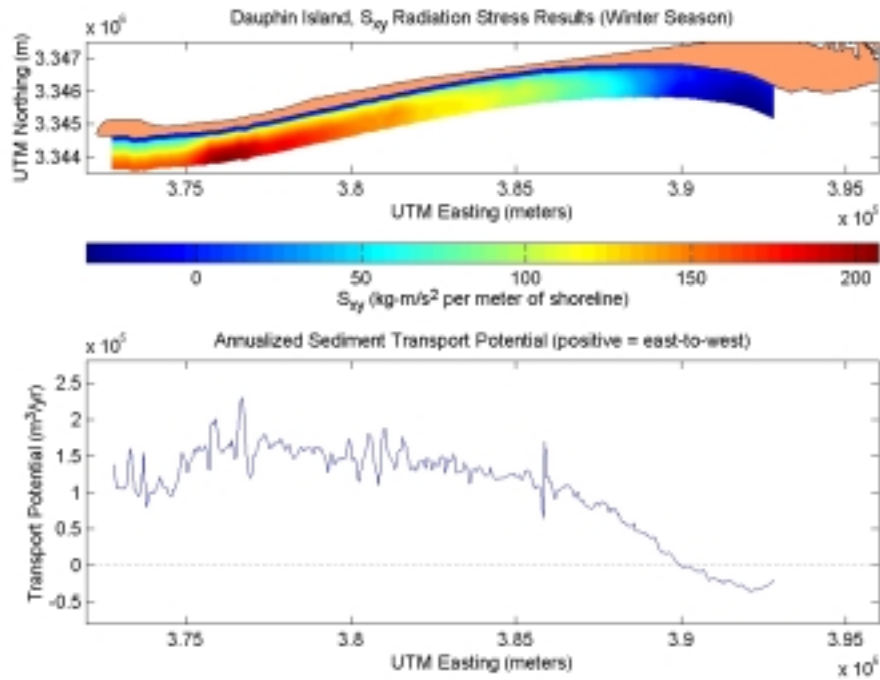
Figure C2-11. S_{xy} radiation stress and annualized sediment transport potential for post-dredging scenario at Dauphin Island during the winter season.
