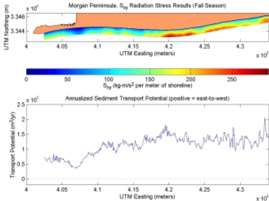
Figure C2-8. S_{xy} radiation stress and annualized sediment transport potential for existing conditions at Morgan Peninsula during the fall season.
