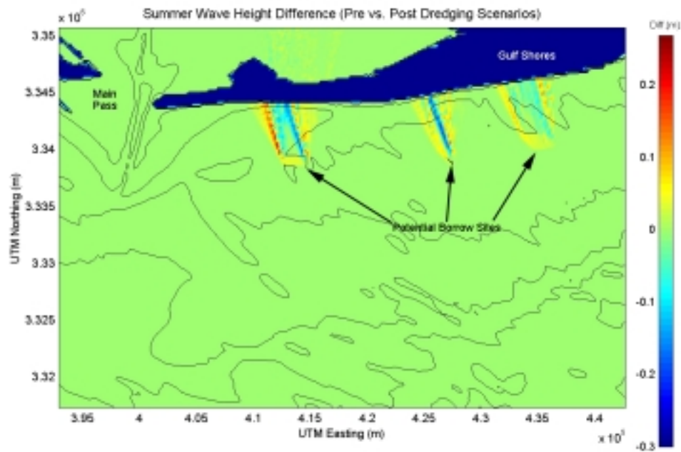
Figure B4-6. Wave height modifications caused by the offshore sand mining at Resource Areas 1, 2, and 3 for a typical summer season.
