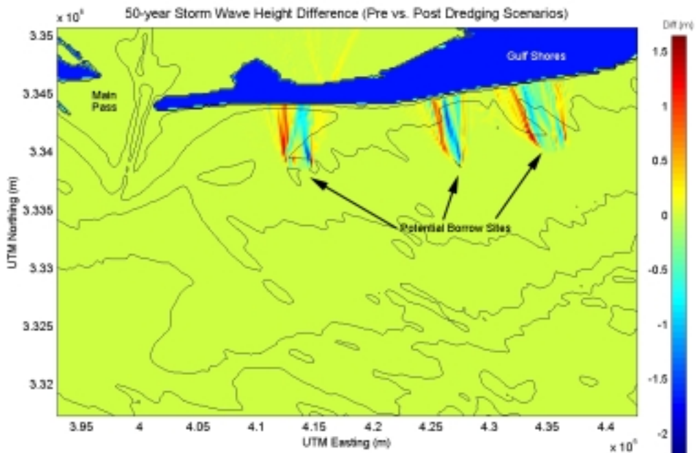
Figure B4-10. Wave height modifications caused by the offshore sand mining at Resource Areas 1, 2, and 3 for a 50-year storm.
