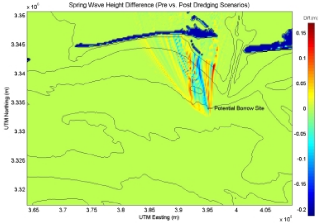
Figure B4-3. Wave height modifications caused by the offshore sand mining at Resource Area 4 for a typical spring season.
