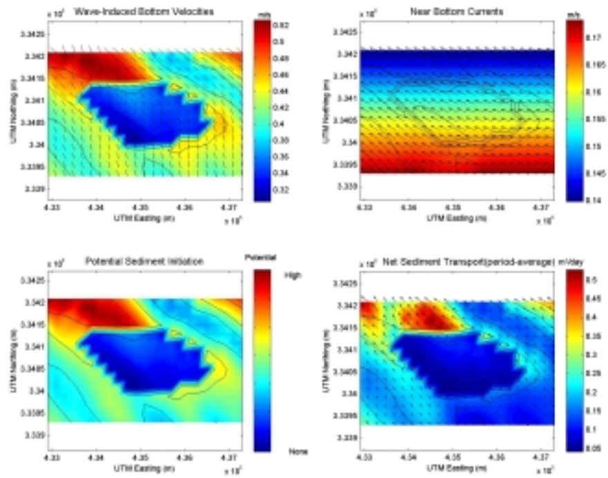
Figure C1-5. Fall hydrodynamic and sediment transport results at Sand Resource Area 1. The solid black lines represent depth contours, and sediment transport results are based on 200 m cell widths.
