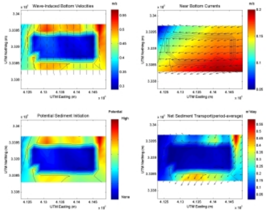
Figure C1-14. West winter hydrodynamic and sediment transport results at Sand Resource Area 3. The solid black lines represent depth contours, and sediment transport results are based on 200 m cell widths.
