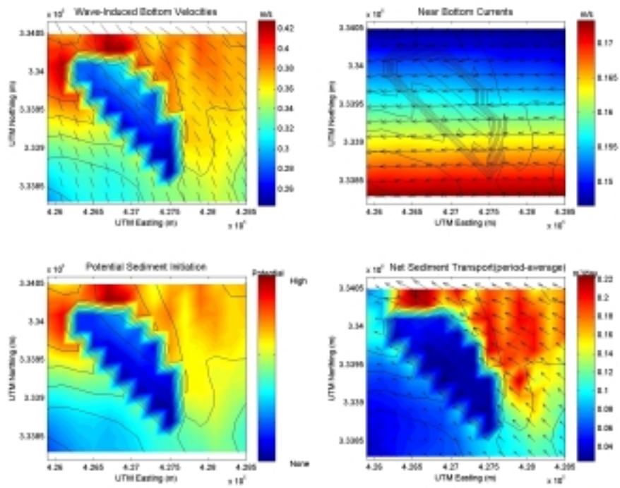
Figure C1-11. Fall hydrodynamic and sediment transport results at Sand Resource Area 2. The solid black lines represent depth contours, and sediment transport results are based on 200 m cell widths.
