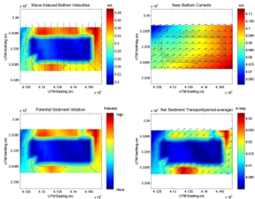
Figure C1-16. Summer hydrodynamic and sediment transport results at Sand Resource Area 3. The solid black lines represent depth contours, and sediment transport results are based on 200 m cell widths.
