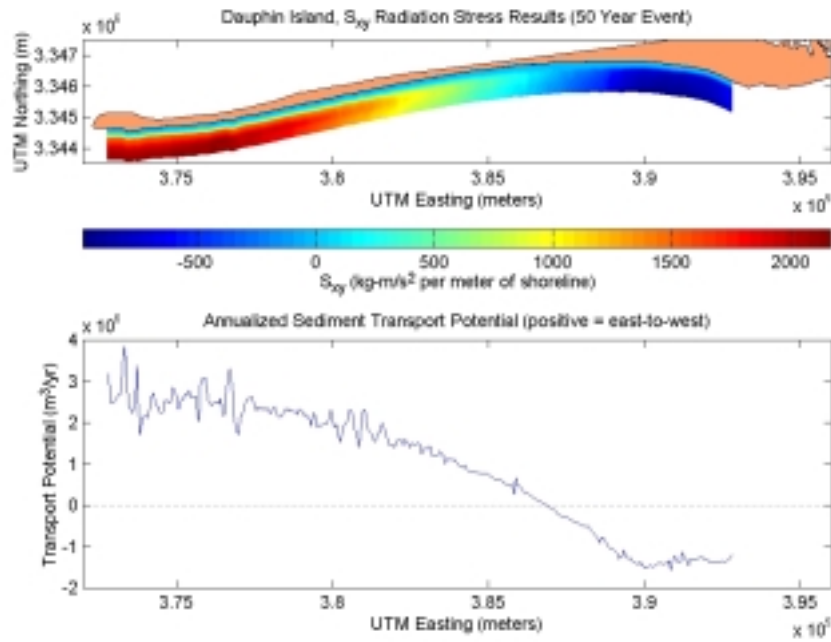
Figure C2-9. S_{xy} radiation stress and annualized sediment transport potential for existing conditions at Dauphin Island during a 50-year storm.
