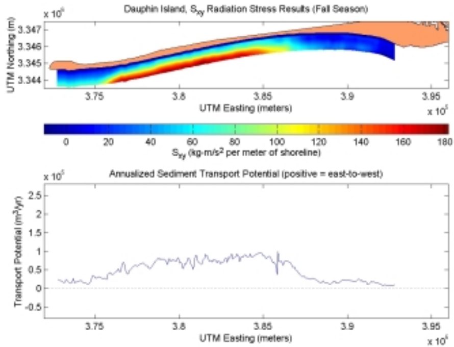
Figure C2-7. S_{xy} radiation stress and annualized sediment transport potential for existing conditions at Dauphin Island during the fall season.
