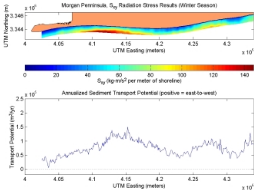
Figure C2-12. S_{xy} radiation stress and annualized sediment transport potential for post-dredging scenario at Morgan Peninsula during the winter season.
