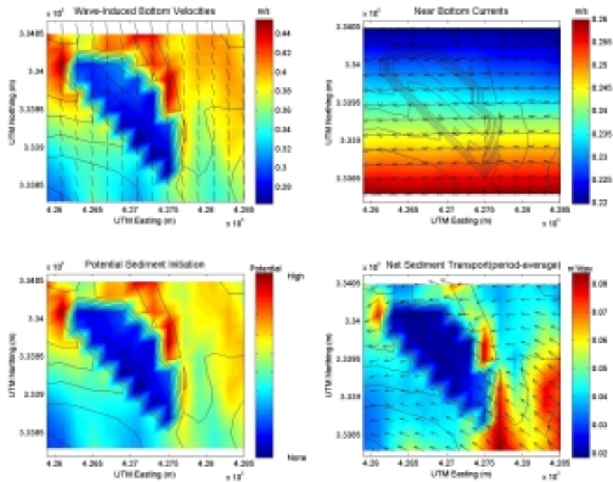
Figure C1-8. West winter hydrodynamic and sediment transport results at Sand Resource Area 2. The solid black lines represent depth contours, and sediment transport results are based on 200 m cell widths.
