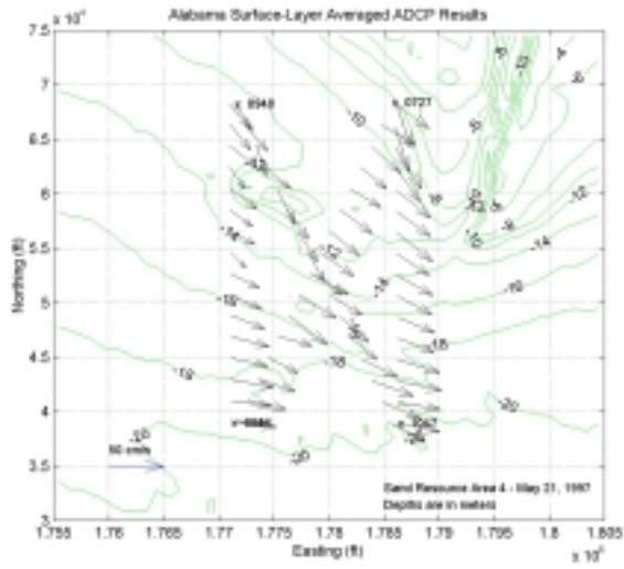
Surface Layer
