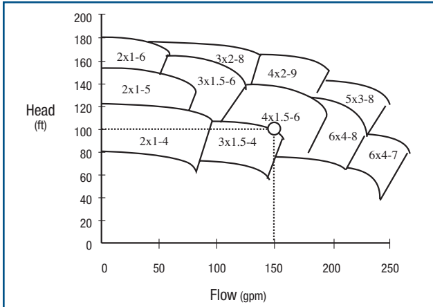
Figure 11. Family of Pump Performance Curves
