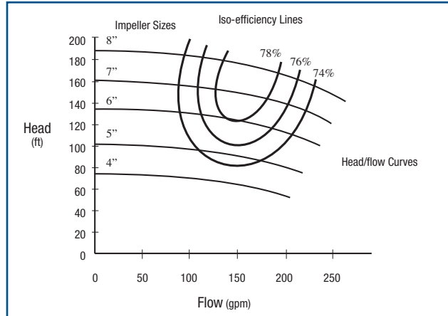
Figure 12. Performance Curves for Different Impeller Sizes
