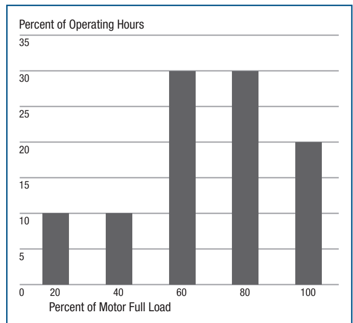
Figure 12. Load duty cycle – Example 2
