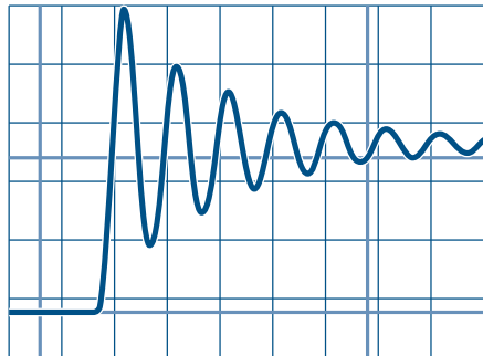
Figure 1. PWM pulse with reflected voltage or ringing
