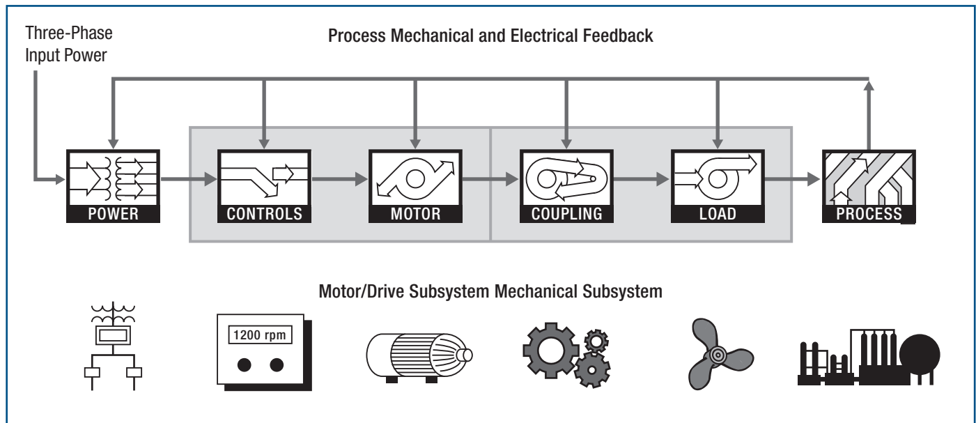
Figure 17. Electric Motor System
