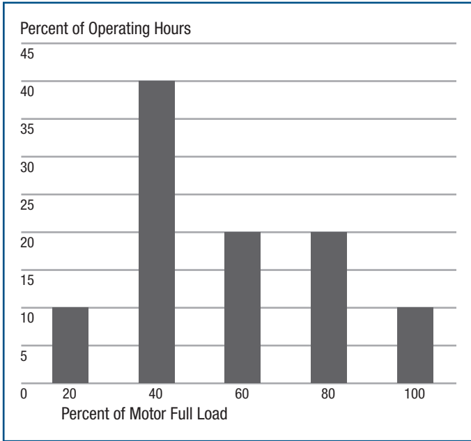
Figure 10. Load duty cycle – Example 1
