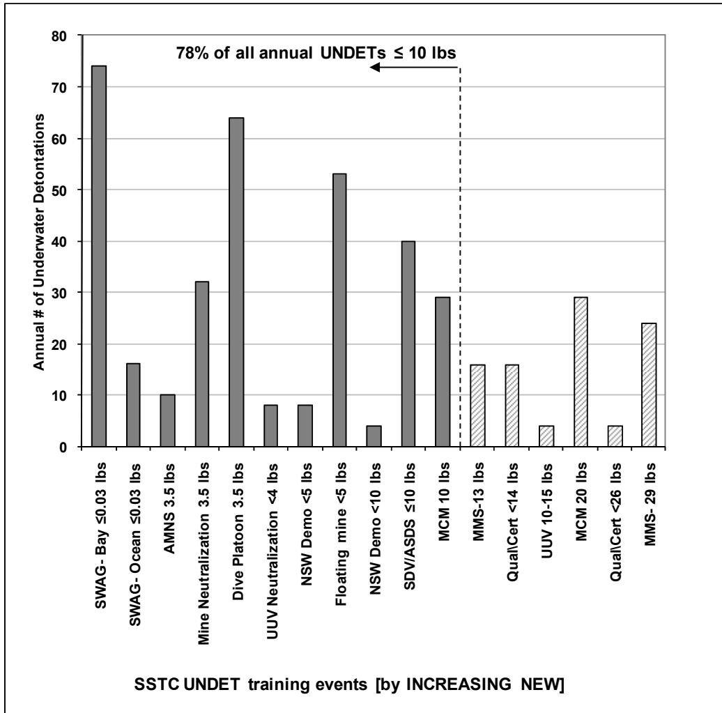
Figure 2-2. SSTS underwater detonations listed by increasing charge weight.
