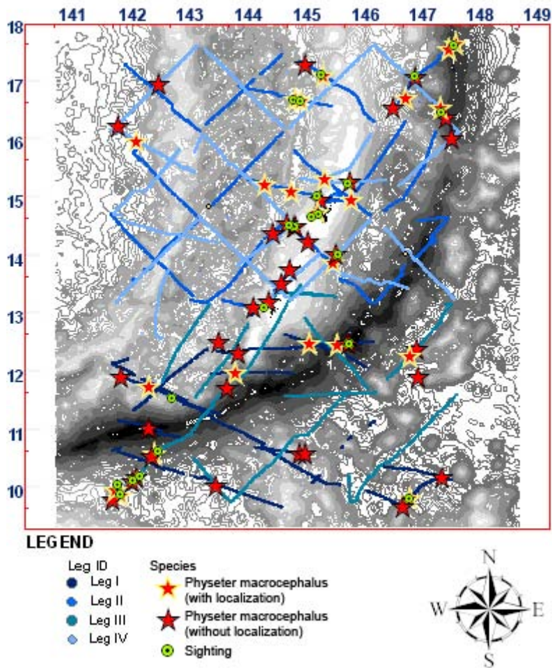
Sperm whale acoustic detections (red stars) and visual sightings (green bulls-eyes)
