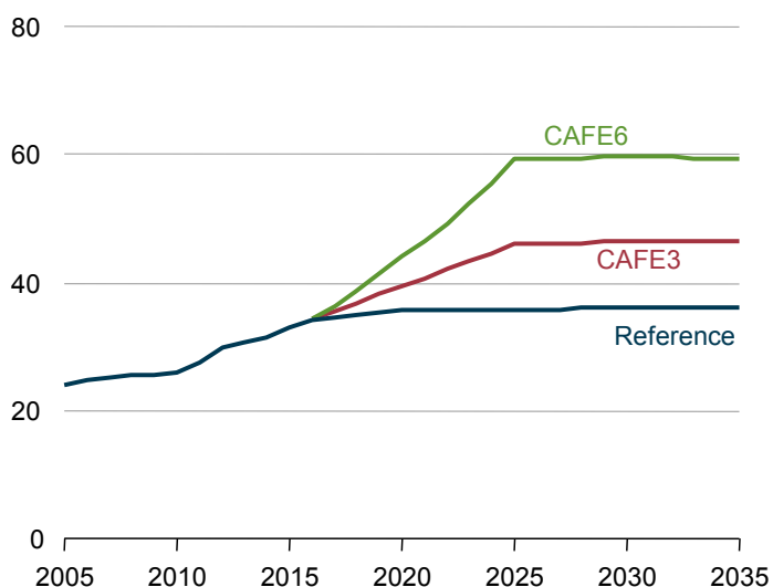
Figure 16. Combined CAFE standards for light-duty vehicles in three cases, 2005-2035 (miles per gallon)
