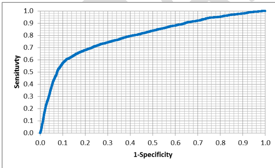
Appendix Figure 1. ROC Plot of Sensitivity against 1-Specificity with an AUC of 0.792 for the Young Chicken Salmonella Predictive Model
