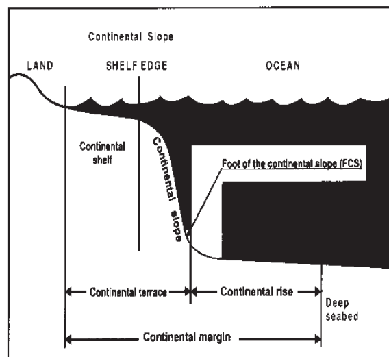
Figure 1. The foot of the Continental Slope (FCS) as located on cross-section of the continental shelf.
