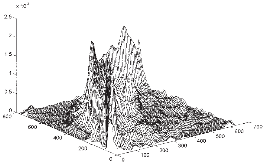
Figure 12. 3-D Net display of the SMC; x, y, and z axes are in kilometers using the spline-smoothed NOAA ETOPO5 data with smoothing parameters: p_x = 7.00728 \times 10^{-4} , p_y = 3.650 \times 10^{-4} 7 degrees longitude and 7 degrees latitude portion of U.S. Atlantic coast (28.135-kilometer grid interval x-axis; 35.000-kilometer grid interval y-axis (85 x 85 grid); FCS is the peak of the highest ridge).
