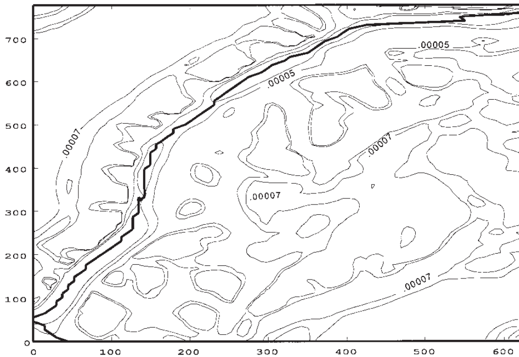
Figure 13. Contour map of the SMC; x, y, and z axes in kilometers with smoothing parameters: p_x = 7.00728 \times 10^{-4} , p_y = 3.650 \times 10^{-4} 7 degrees longitude by 7 degrees latitude portion of U.S. Atlantic coast (contour values in kilometers as labeled; 28.135-kilometer grid interval x-axis; 35.000-kilometer grid interval y-axis (85 x 85 grid); heavy line is a plot of the FCS as found by SMC).
