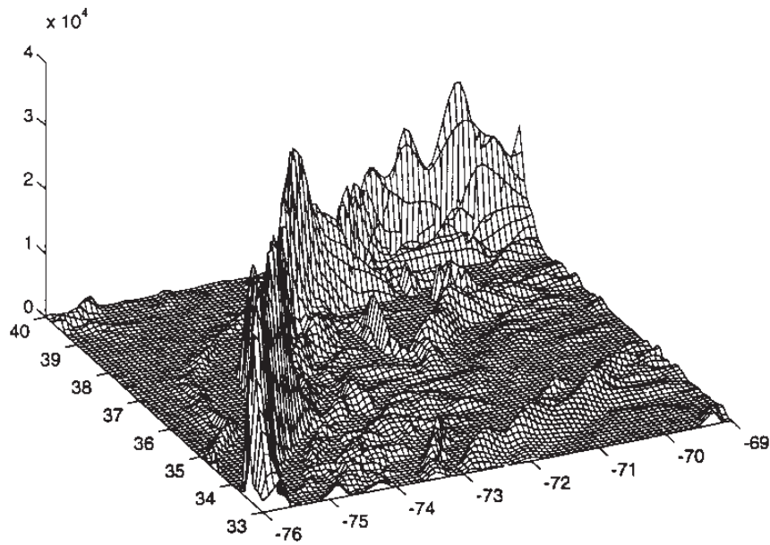
Figure 8. 3-D Net display of the SDG of spline-smoothed NOAA ETOPO5 data with p = p_x = p_y = .9990 from 7 degrees longitude by 7 degrees latitude portion of the U.S. Atlantic coast 5-nautical mile grid interval (85 x 85 grid); FCS is located by the peak of the highest ridge).
