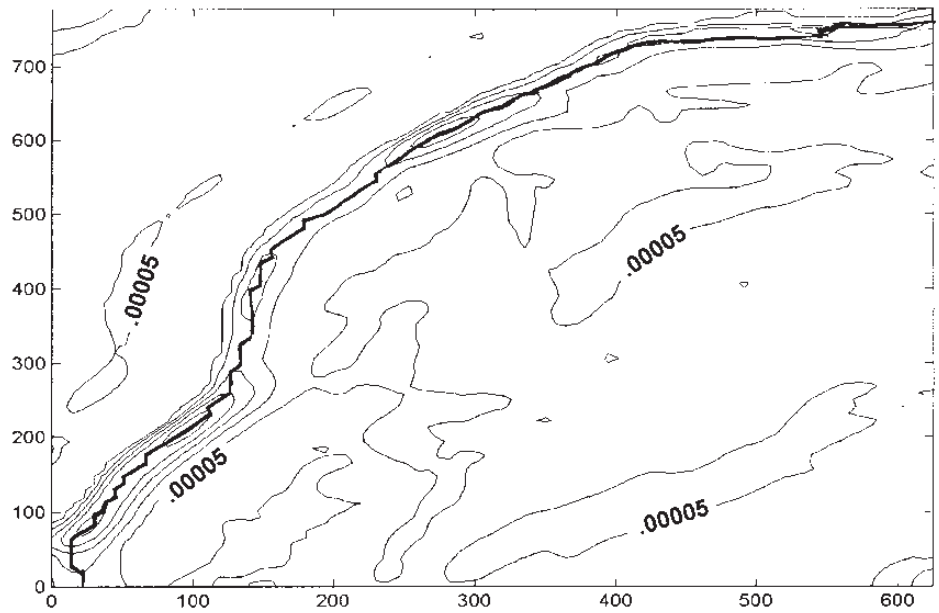
Figure 15. Contour map of the SDG, x , y , and z axes in kilometers with smoothing parameters: p_x = 7.00728 \times 10^{-4} , p_y = 3.650 \times 10^{-4} 7 degrees longitude by 7 degrees latitude portion of U.S. Atlantic coast (contour values in kilometers as labeled; 28.135-kilometer grid interval x -axis; 35.000-kilometer grid interval y -axis (85 x 85 grid); heavy line is a plot of the FCS as found by SDG).
