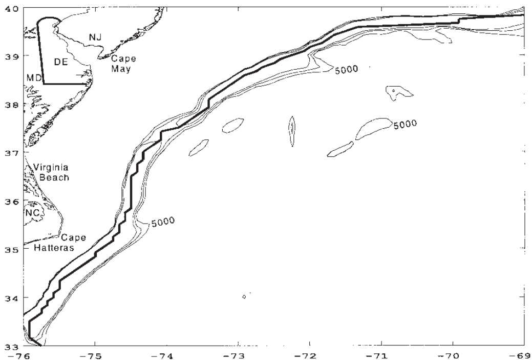
Figure 9. Contour map of the SDG using the spline-smoothing NOAA ETOPO5 data with smoothing parameters: p = p_x = p_y = .9990 , 7 degrees longitude by 7 degrees latitude portion of U.S. Atlantic coast (FCS is obtained from the crest of the highest ridge; 5-nautical mile grid interval (85 x 85 grid); heavy line is a plot of the FCS as found by SDG).
