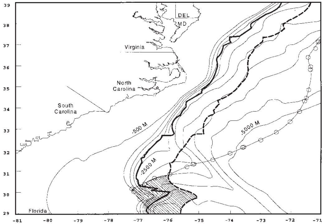
Figure B2. Contour map of the NOAA ETOPO5 data with smoothing parameter p=.9990 , U.S. Atlantic coast, 10 degrees longitude by 10 degrees latitude (5-nautical mile grid interval; contour interval=500 meters; heavy line is a plot of the location of FCS as found by SDG; heavy dashed line is location of the FCS plus 60 nautical miles; line with circles over it is the 200-nautical mile EEZ).
