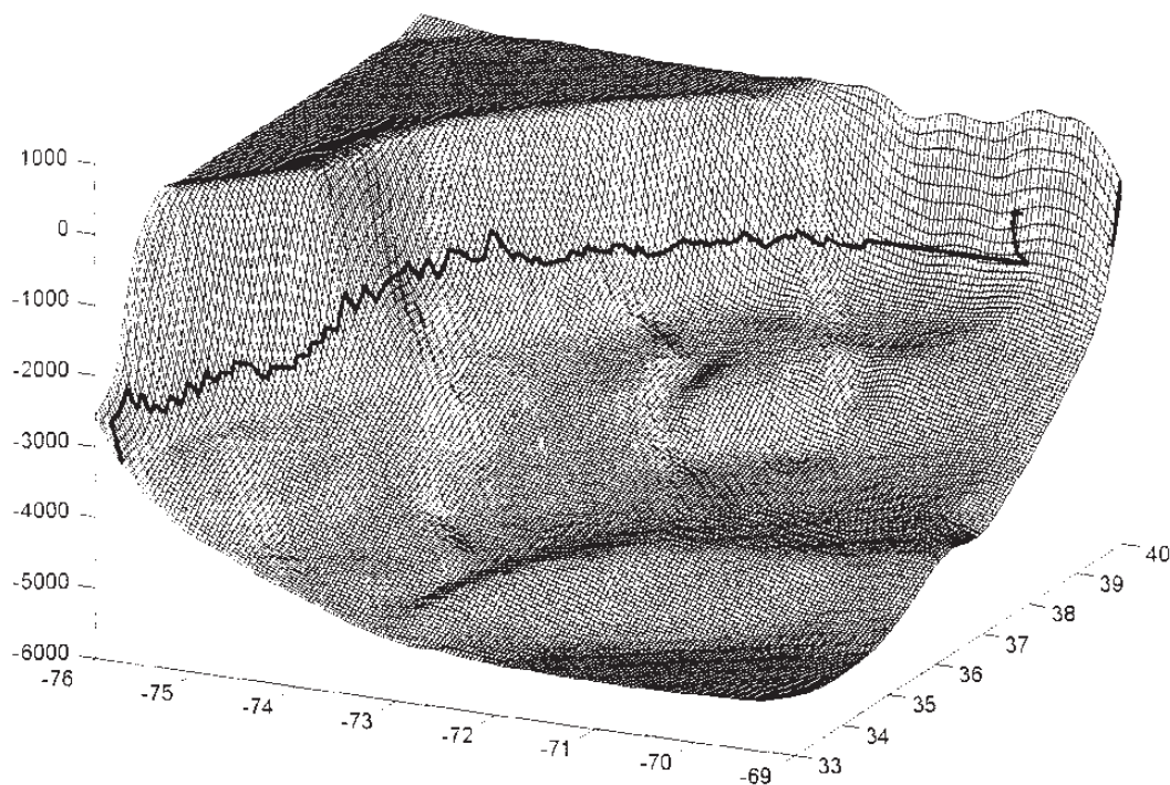
Figure 10. 3-D Net display of the spline-smoothed NOAA ETOPO5 data with smoothing parameters: p = p_x = p_y = .9990 from 7 degrees longitude by 7 degrees latitude portion of U.S. Atlantic coast ( Z = 0' is sea level; 2.5-nautical mile grid interval (170 x 170 grid); heave line is a plot of the FCS as found by SDG).
