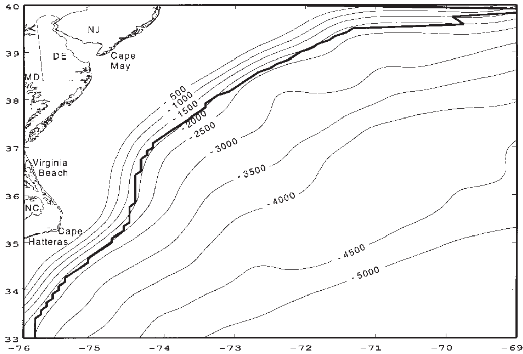
Figure 7. Contour map of the spline-smoothed NOAA ETOPO5 data with smoothing parameters: p = p_x = p_y = .9990 from 7 degrees longitude by 7 degrees latitude portion of U.S. Atlantic coast (contour interval = 500 meters; 5-nautical mile grid interval (85 x 85 grid); heavy line is a plot of the FCS as found by the SDG).
