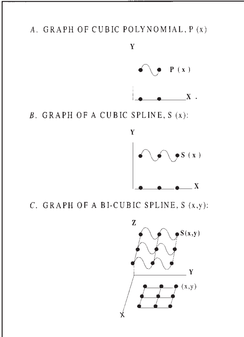
Figure A1. Graphs of (A) cubic polynomial P(x) , (B) cubic spline S(x) , and (C) bi-cubic spline S(x,y) .
