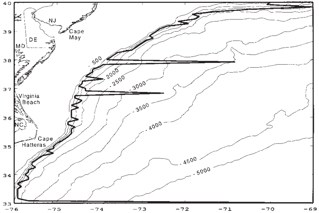
Figure 4. Contour map of original NOAA ETOPO5 data with smoothing parameters: p = p_x = p_y = 1.0 of 7 degrees longitude by 7 degrees latitude portion of U.S. Atlantic coast (contour interval = 500 meters; 5-nautical mile grid interval (85 x 85 grid); heavy line is a plot of the FCS as found by SDG).
