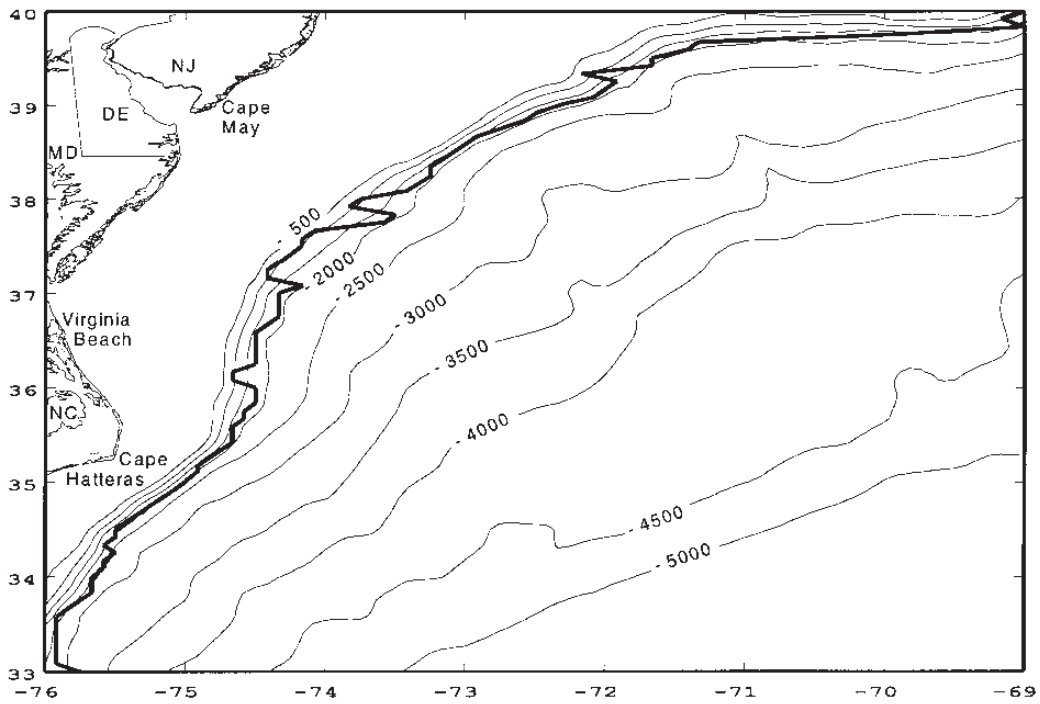
Figure 5. Contour map of the spline-smoothed NOAA ETOPO5 data with smoothing parameters: p = p_x = p_y = .9999 from 7 degrees longitude by 7 degrees latitude portion of U.S. Atlantic coast (contour interval = 500 meters; 5-nautical mile grid interval (85 x 85 grid); heavy line is a plot of the FCS as found by SDG).
