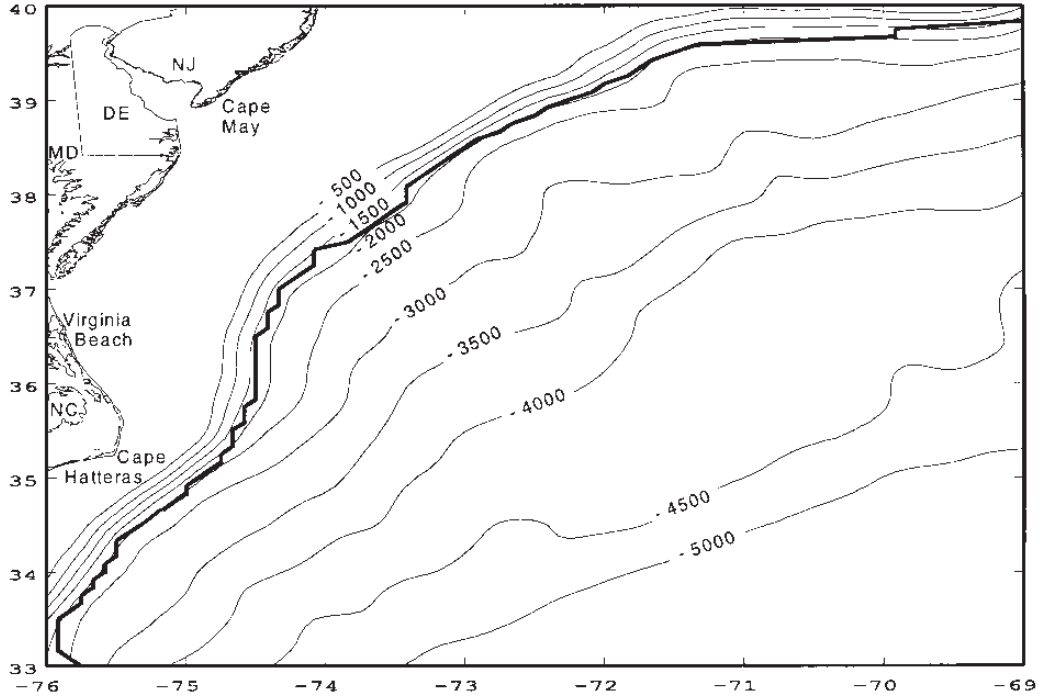
Figure 6. Contour map of the spline-smoothed NOAA ETOPO5 data with smoothing parameters: p = p_x = p_y = .9990 from 7 degrees longitude by 7 degrees latitude portion of U.S. Atlantic coast (contour interval = 500 meters; 5-nautical mile grid interval (85 x 85 grid); heavy line is a plot of the FCS as found by the SDG).
