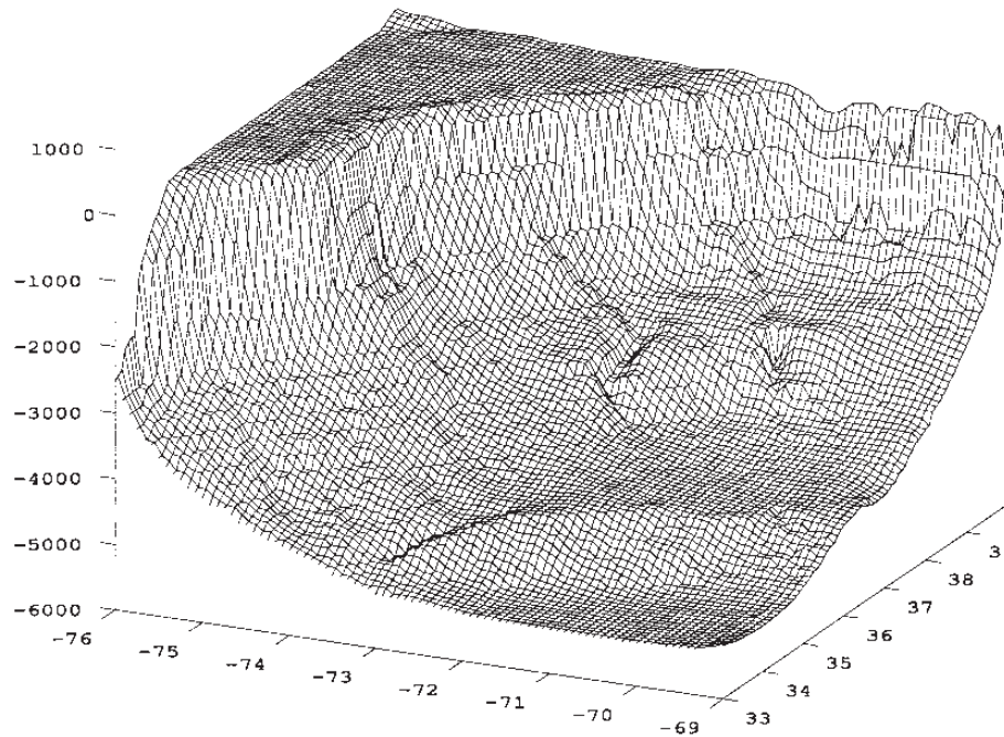
Figure 3. 3-D Net display of original NOAA ETOPOS data of 7 degrees longitude by 7 degrees latitude portion of U.S. Atlantic coast ('Z = 0' is sea level; 5-nautical mile grid interval (85 x 85 grid)) p=1 .
