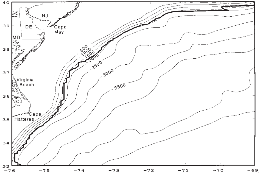
Figure 11. Contour map of the spline-smoothed NOAA ETOPOS data with smoothing parameters: p_x = p_y = p_z = .9990 from 7 degrees longitude by 7 degrees latitude portion of U.S. Atlantic coast (contour interval = 500 meters; 2.5-nautical mile grid interval (170 X 170 grid); heavy line is the FCS as found by SDG).
