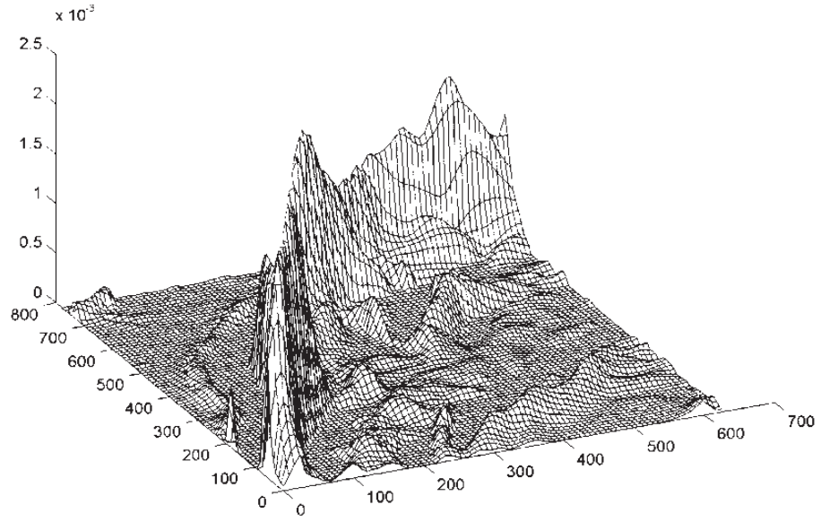
Figure 14. 3-D Net display of the SDG, x , y , and z axes are in kilometers using the spline-smoothed NOAA ETOPO5 data with smoothing parameters: p_x = 7.00728 \times 10^{-4} , p_y = 3.650 \times 10^{-4} 7 degrees longitude by 7 degrees latitude portion of U.S. Atlantic coast (28.135-kilometer grid interval x -axis; 35.000-kilometer grid interval y -axis (85 x 85 grid); FCS is the peak of the highest ridge).
