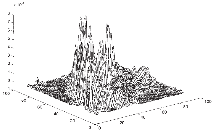
Figure 16. 3-D Net display of \Delta = \text{SMC} - \text{SDG} , x , y , and z axes are in kilometers using the spline-smoothed NOAA ETOPO5 data with smoothing parameters: p_x = 7.00728 \times 10^{-4} , p_y = 3.650 \times 10^{-4} 7 degrees longitude by 7 degrees latitude portion of U.S. Atlantic coast (28.135-kilometer mile grid interval x -axis; 35.000-kilometer grid interval y -axis (85 x 85 grid)).
