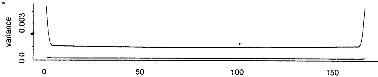
(b) variance of trend estimate
