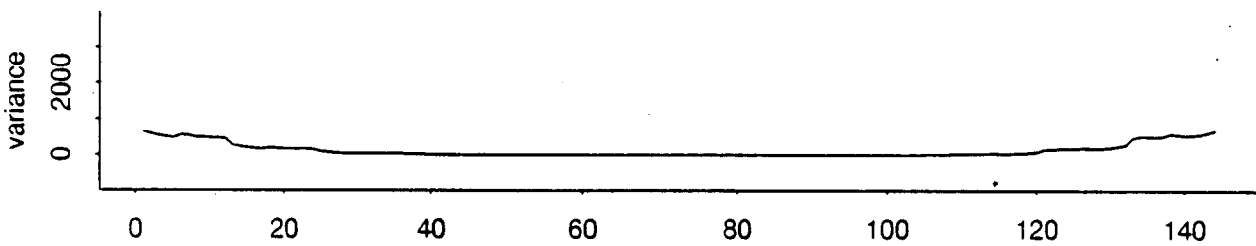
(c) contribution of fore/backcast error (b 0 f)
