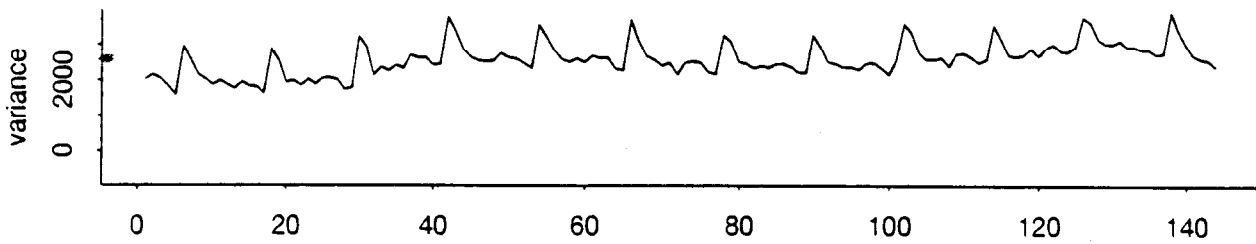
(b) contribution of sampling error (e)
