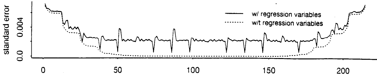
(a) standard error of seasonally adjusted data
