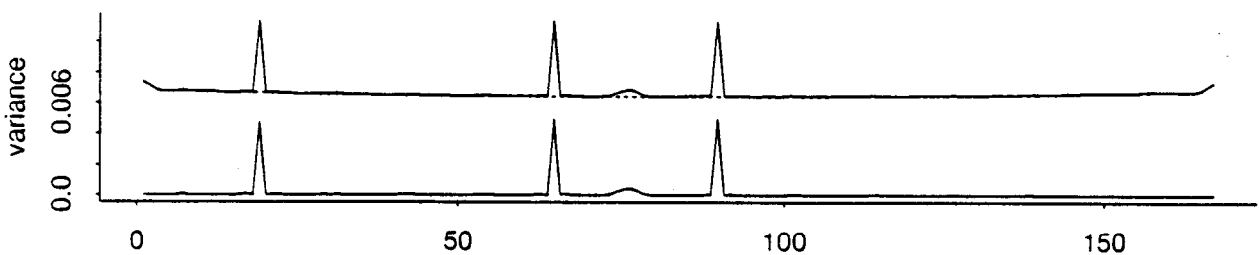
(c) variance of seasonally and outlier adjusted series
