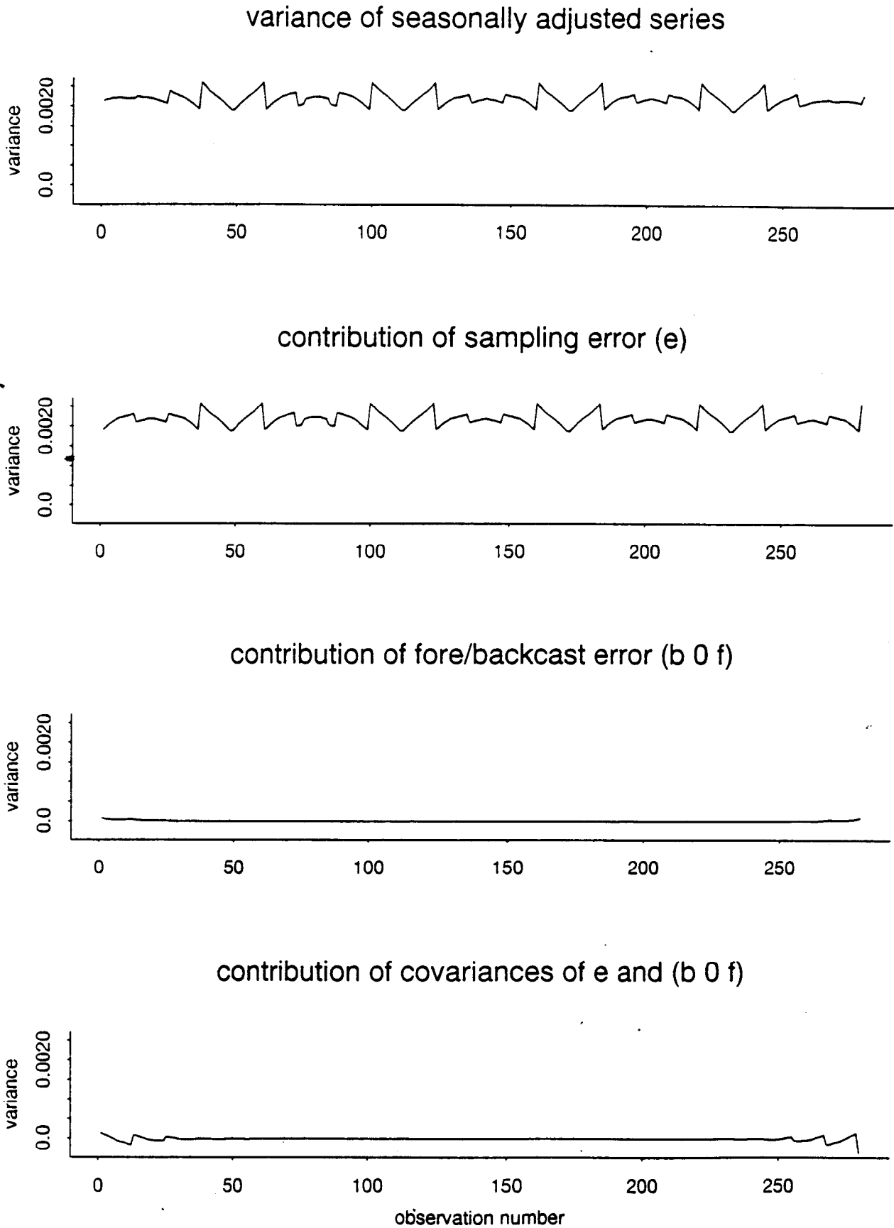
Figure 9. Drinking Places: Default X-11
