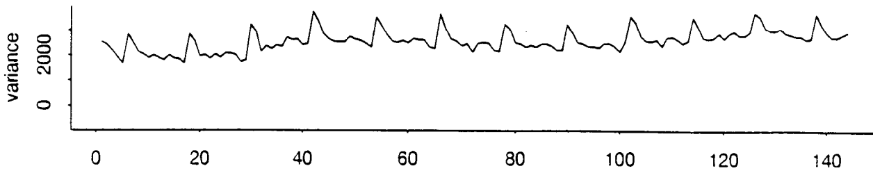
(a) variance of seasonally adjusted series
