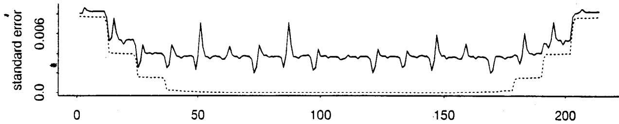
(b) standard error of month-to-month changes
