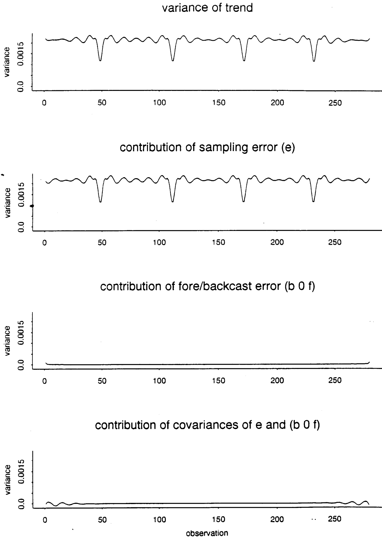
Figure 11. Drinking Places: Default X-11
