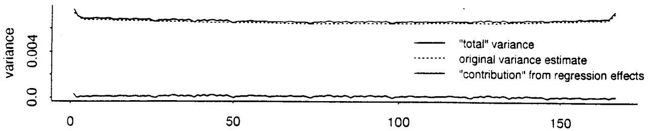
(a) variance of seasonally and trading-day adjusted series
