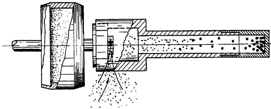
Figure 6. 10 mm cyclone with filter.
