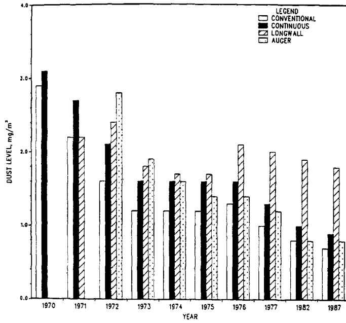
Figure 11. A yearly comparison of dust levels for four types of mining.
