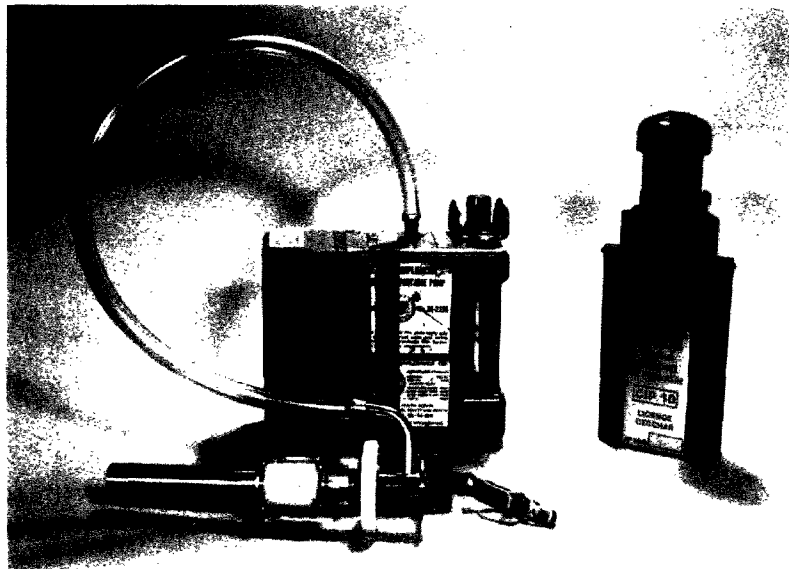
Figure 1—Coal mine dust personal sampler unit and CIP 10.
