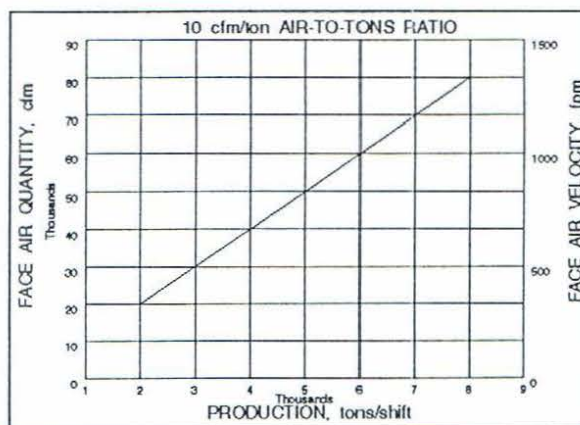
Figure 1. Relationship of airflow and production to maintain a 2.0 mg/m 3 dust concentration.
