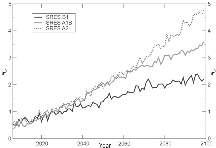
FIGURE 2-6 Annual surface air temperature anomaly, from the 1990–1999 average, for the eastern United States and for three different emissions scenarios (SRES = Special Report on Emission Scenarios ). (Source: Peterson et al. 2006, Figure 5.)
