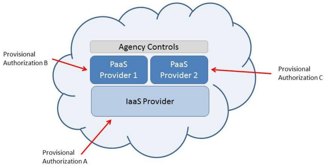
Figure 3-14. Three Providers, One IaaS and Two PaaS
