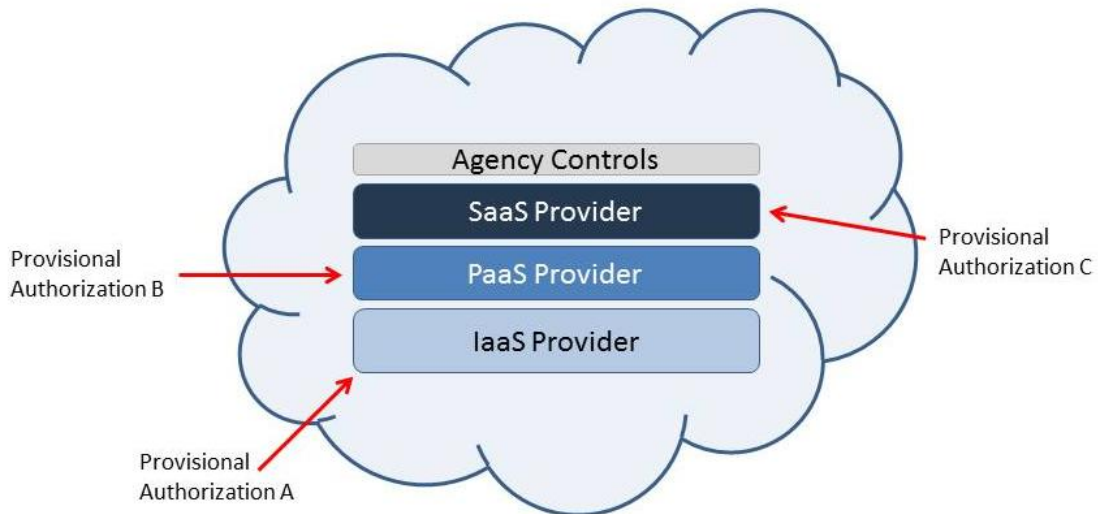
Figure 3-11. Three Providers, One IaaS, One PaaS, and One SaaS
