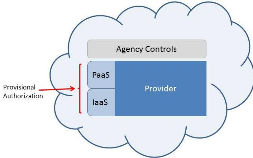
Figure 3-7. One Provider for IaaS and PaaS
