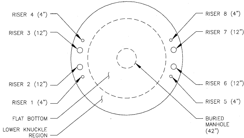
Figure 4. Catch Tank Riser Layout.
