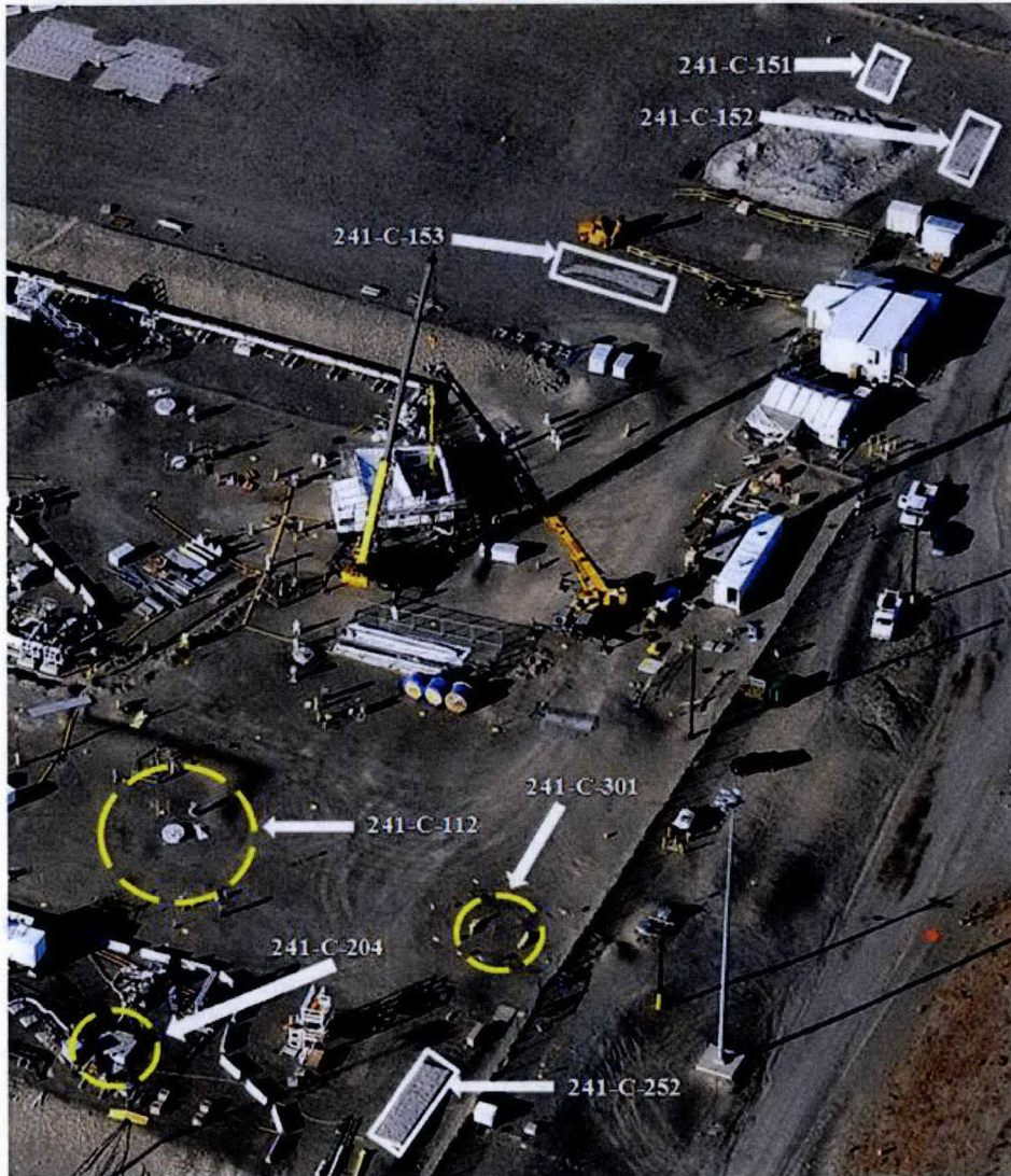
Figure 1. Aerial Photograph with Catch Tank and Diversion Boxes.
