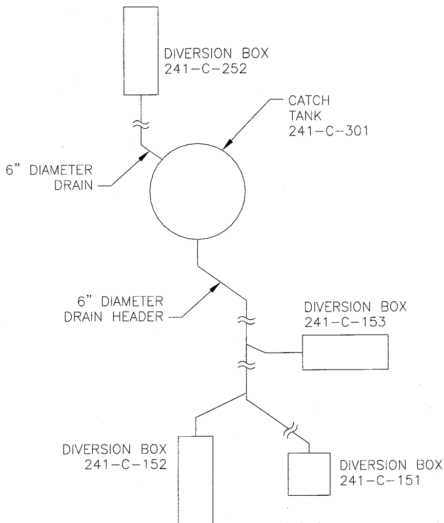
Figure 2. Catch Tank and Diversion Boxes.
