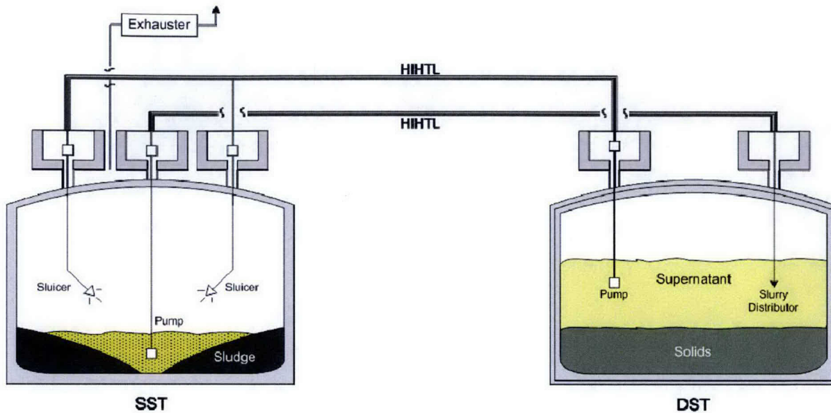
Figure 8. Modified Sluicing Retrieval Schematic.
