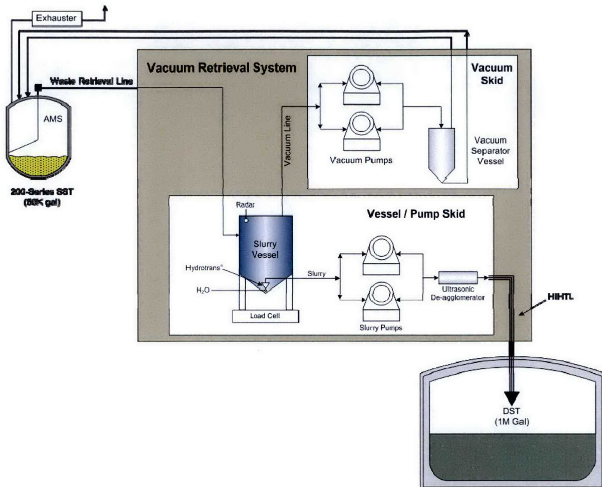
Figure 7. Vacuum Retrieval System Schematic.
