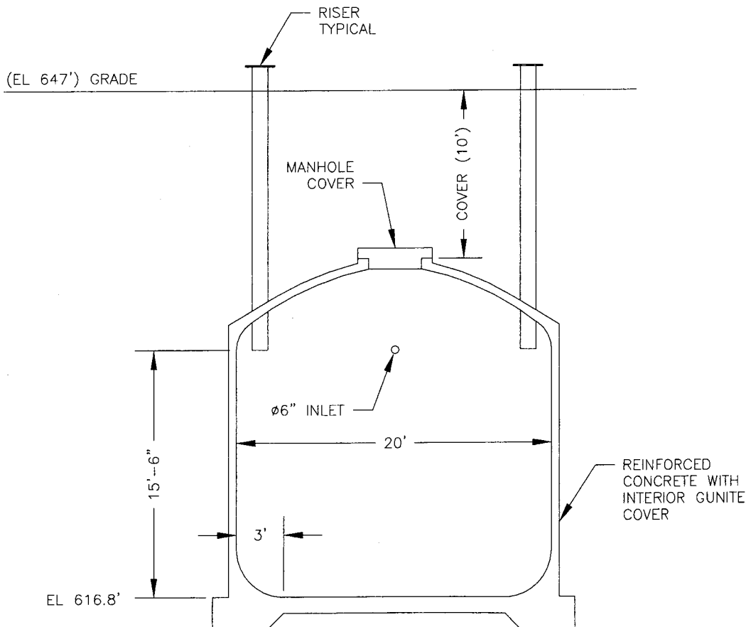
Figure 3. Catch Tank Configuration.
