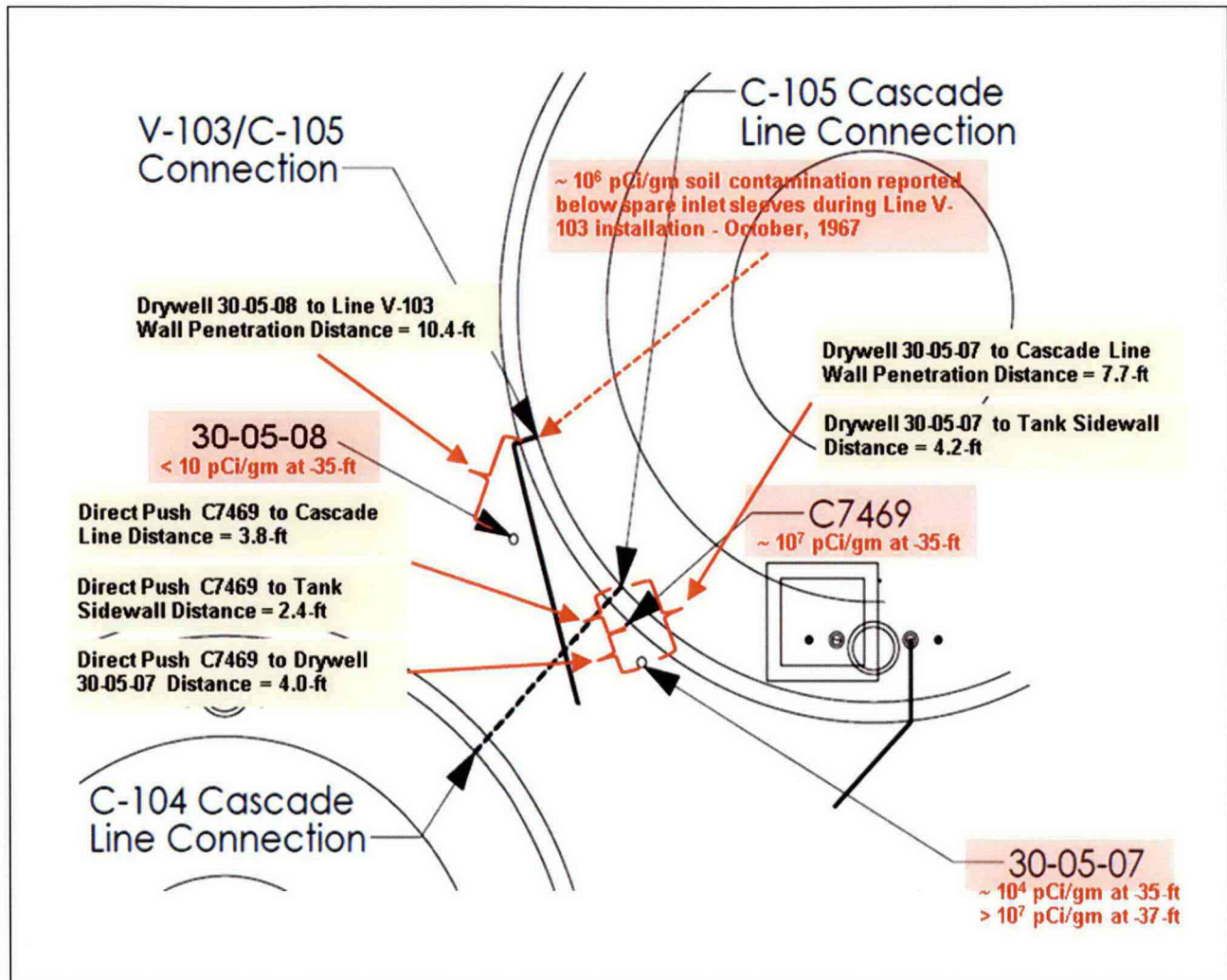
Figure 7-1 Tank Features and Separation Distances
